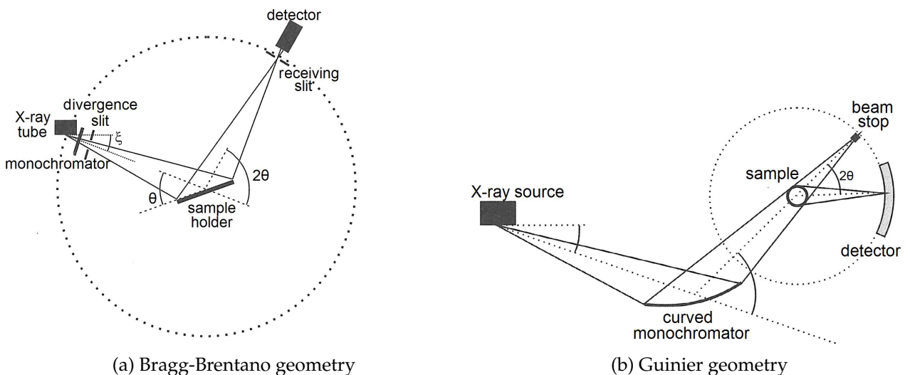
FIGURE 2.6: Schematic principle of Bragg-Brentano and Guinier powder X-ray diffractometer geometry
