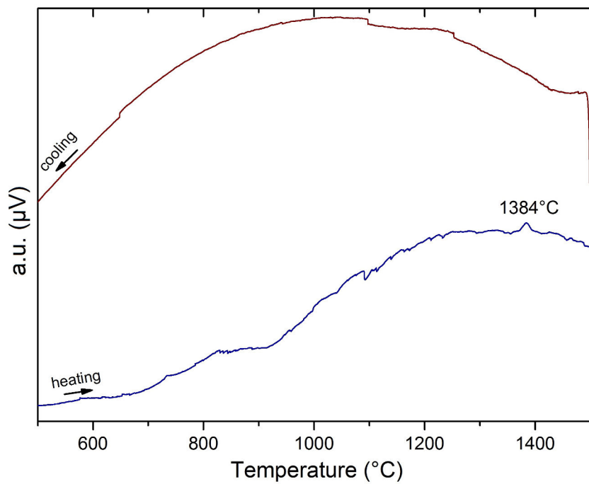
FIGURE 3.14: DSC heating and cooling curves of the sample n°33. The signal at 1384°C corresponds to decomposition of the \text{Al}_{2.4}\text{Ir} compound.
