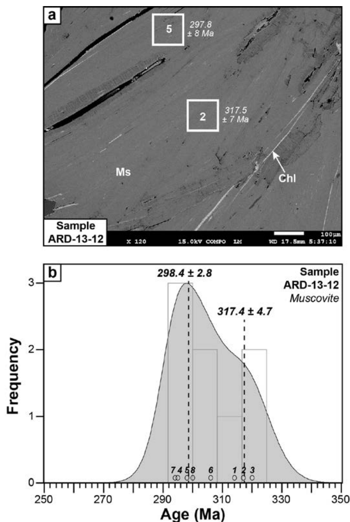
Fig. 88: Results of the ^{40}\text{Ar}/^{39}\text{Ar} dating for the selvage muscovite from the St-Mélany deposit (sample ARD-13-12). (a) BSE image of the dated muscovite (Ms) showing homogeneous internal texture, with minor interstitial chlorite (Chl). The location of two ablation spots (100 x 100 \mu\text{m} ) is indicated on the BSE image with the corresponding obtained ages. (b) Frequency histogram of the ^{40}\text{Ar}/^{39}\text{Ar} ages obtained on muscovite and identification of the two age modes. Data are given in Table 25.
