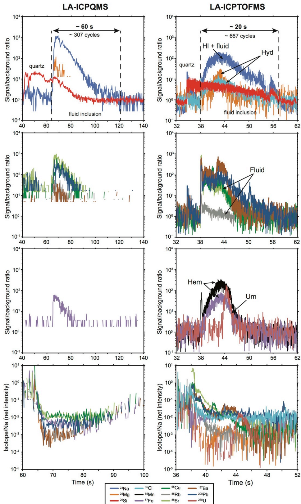
Fig. 43: Typical transient signals for 15 \mu\text{m} multi-phase fluid inclusions (sample 7703-25, Zambia) analysed by LA-ICPQMS and LA-ICPTOFMS. The signals for detected elements obtained by QMS with the standard ablation cell have all the same shape and are correlated in time (top left to middle left), as observed by constant ratios normalised to Na (bottom left). The signals obtained by TOFMS with the fast washout cell differ from one group of isotopes to another, as shown by variable ratios normalised to Na (bottom right), allowing to
