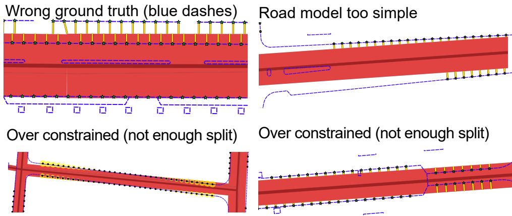
Figure 138: Various illustrations of optimisation process limitation. The data used as ground truth contains errors. Then road axis main not split enough. Last, the simple road model used can not deal with some features of Paris roadway.
