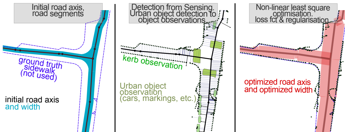
Figure 112: Approximate road axis network and road width are available, forming a basic road modelling. Various sensing methods produce urban feature detections which are processed into consolidated observations, and assigned to road axis segments. A robust non linear least square optimisation then fits the road modelling to observations. The result is much closer to ground truth, even when the road model is too simple for the actual road configuration (varying width, asymmetric changes, curves). The user can further input observations if necessary.
