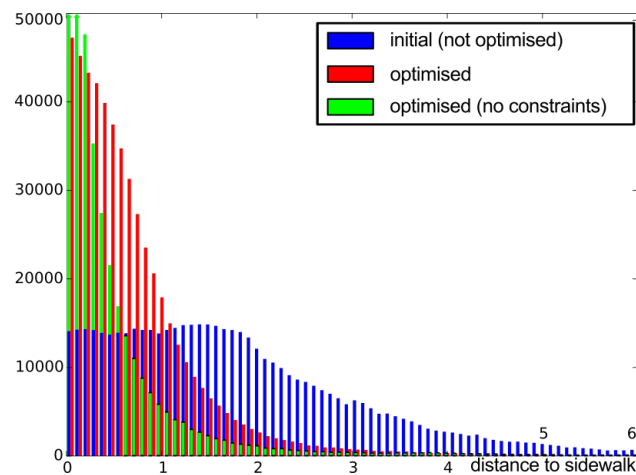
Figure 131: Histogram of absolute distance to ground truth side-walk for "Paris" (optimisation using ground truth as observations).
