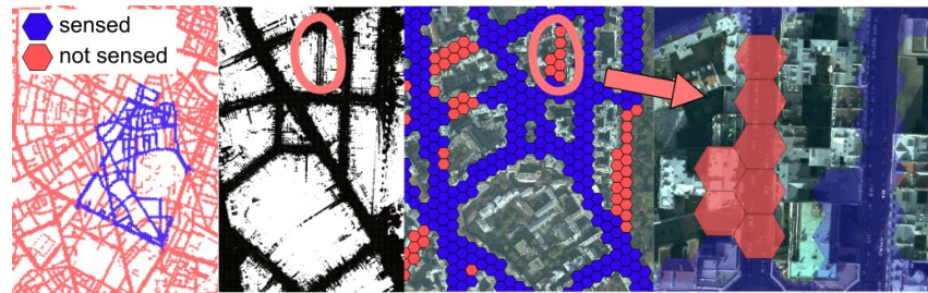
Figure 45: "To-Do" hexagonal map showing the places where the mapping vehicle has not sensed enough points (red hexagon), and where the sensing is sufficient (blue hexagon). Without this map, the zoomed missing part is challenging to notice on raw data.
