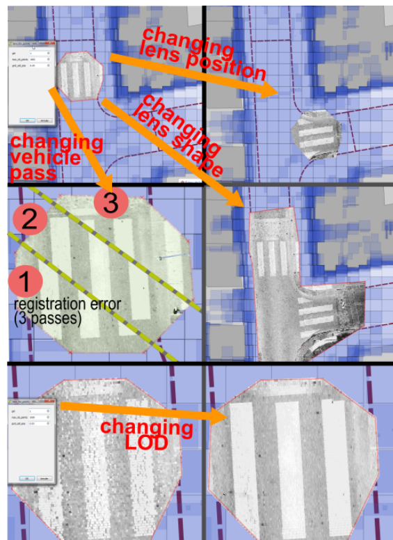
Figure 39: A polygon representing a lens that reveals points underneath it (among billions), with a given Level Of Detail and vehicle pass, at about 100 kpts /s. Points are automatically updated when the lens is modified by the user, using a pure in-base solution, which makes it compatible with any client.
