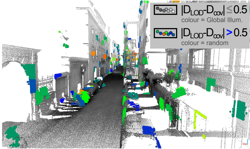
Figure 156: \text{Dim}_{\text{LOD}} and \text{Dim}_{\text{cov}} are mostly comparable, except for few patches (5%, coloured)
