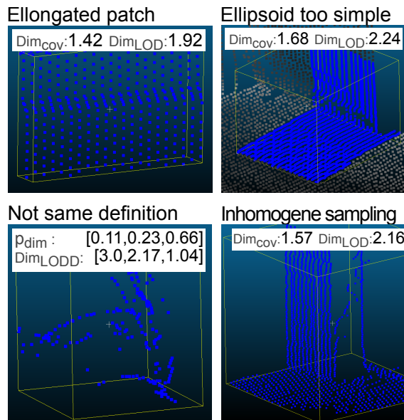
Figure 157: Representative patches for |\text{Dim}_{\text{LOD}} - \text{Dim}_{\text{cov}}| > 0.5 . Most differences are explained by \text{Dim}_{\text{cov}} limitations (See B.4.3.1).
