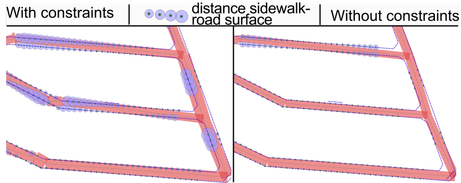
Figure 130: Constraints are necessary to stay close to the initial solution. However, they can significantly degrade the results when there are enough quality observations. Circles are proportional to the distance between ground truth and result. Note that constraint influence can be modulated with weights.
