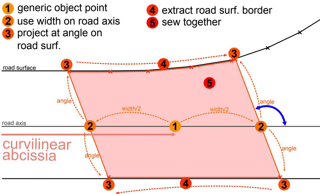
Figure 74: Building the pedestrian crossing surface based on its parameters and road axis and surface.
