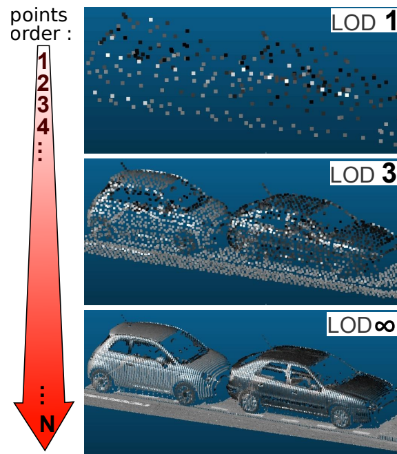
Figure 143: 3 Geometrical Level Of Detail (LOD) for the same point cloud. Reading points from 1 to N gradually increases the details, because of the specific order of points (MidOc).
