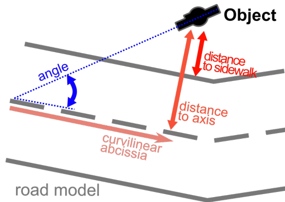
Figure 72: Object position and orientation can be defined relatively to road model.
