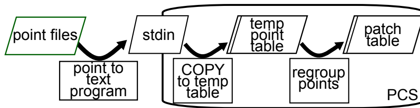
Figure 33: Conceptual schema for parallel loading.
