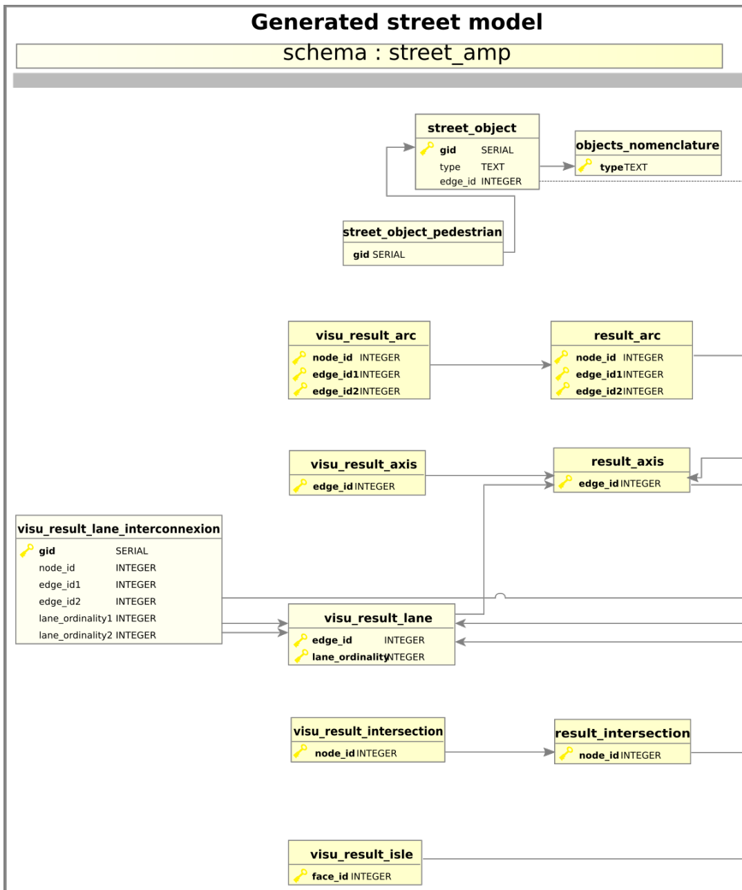
Figure 167: StreetGen base table schema in database (part 1/2)
