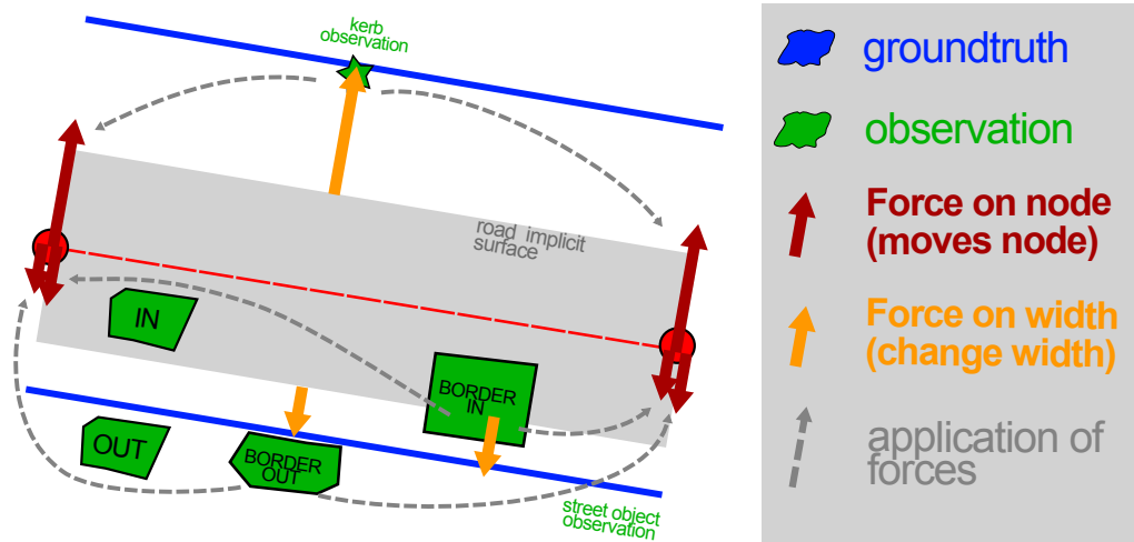
Figure 121: Example of forces induced by observations.
