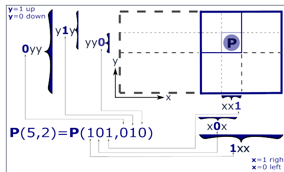
Figure 149: Principle of binary coordinates for a centered, scaled and quantized point cloud.
