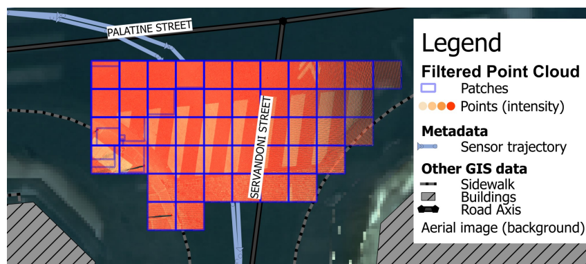
Figure 37: Illustration of a filtering conditions presented in Section 2.4.3.3 p.76. Among billions of points, only those respecting complex filtering conditions are found in ~ 0.1s. Results are shown in QGIS.
