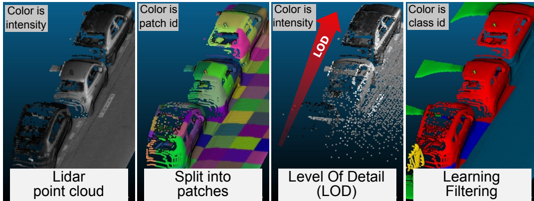
Figure 139: Graphical Abstract : a Lidar point cloud (1), is split it into patches (2) and stored in a Point Cloud Server, patches are re-ordered to obtain free LOD (3) (a gradient of LOD here), lastly the ordering by-product is a multiscale dimensionality descriptor used as a feature for learning and efficient filtering (4).
