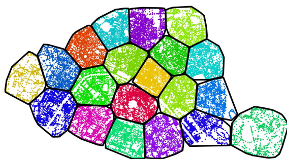
Figure 81: Clustering road axis centroid with K-Means, K=20 , (black segments are convex hull).
