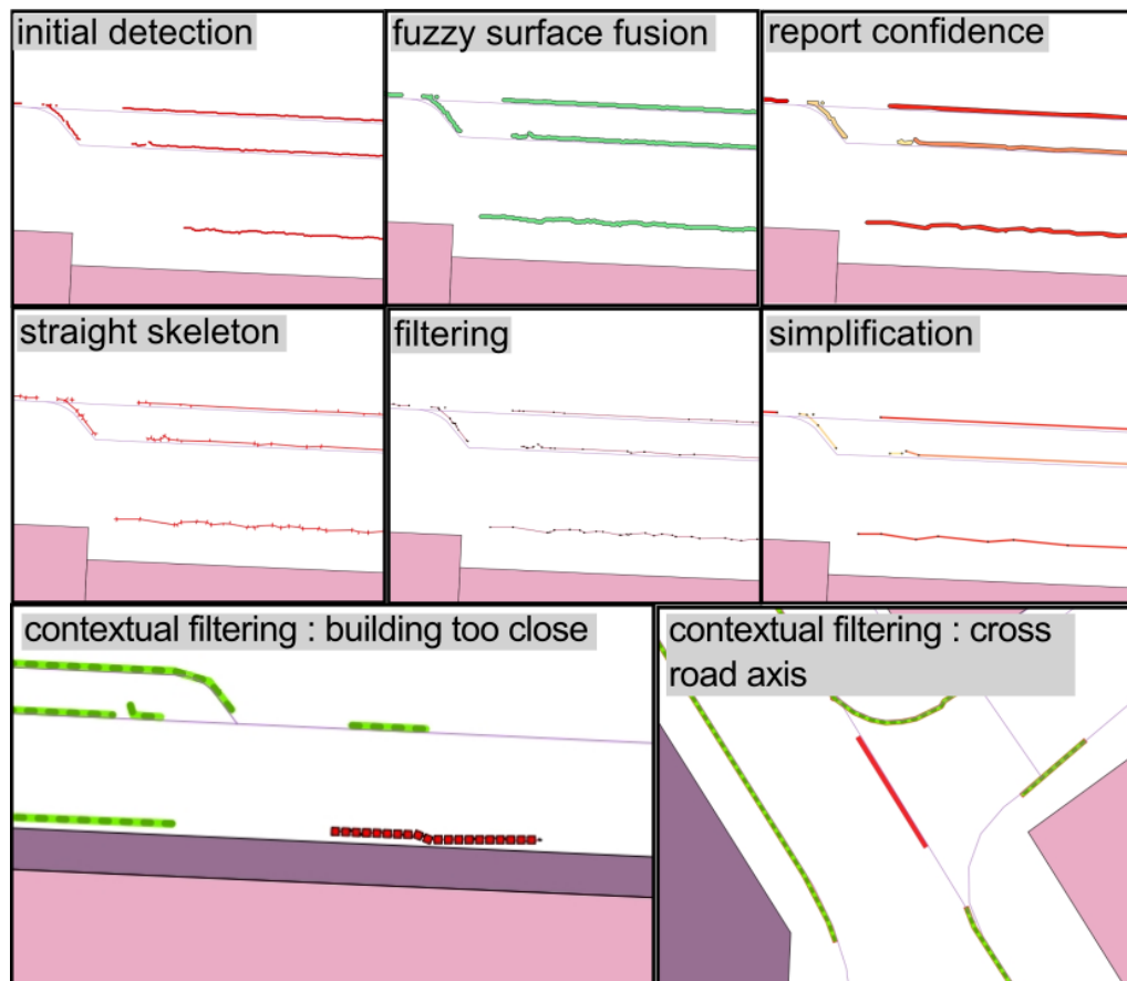
Figure 118: Input kerb detection is consolidated and filtered (both geometrically and with context) to produce suitable observations.
