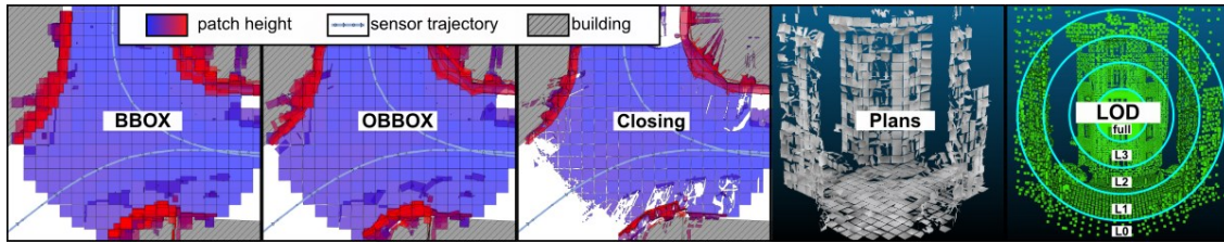
Figure 46: Streets and buildings. Generalisation like Bounding Box, Oriented BBox, Spatial closing. Closing on 3D plan detection. Level Of Details.
