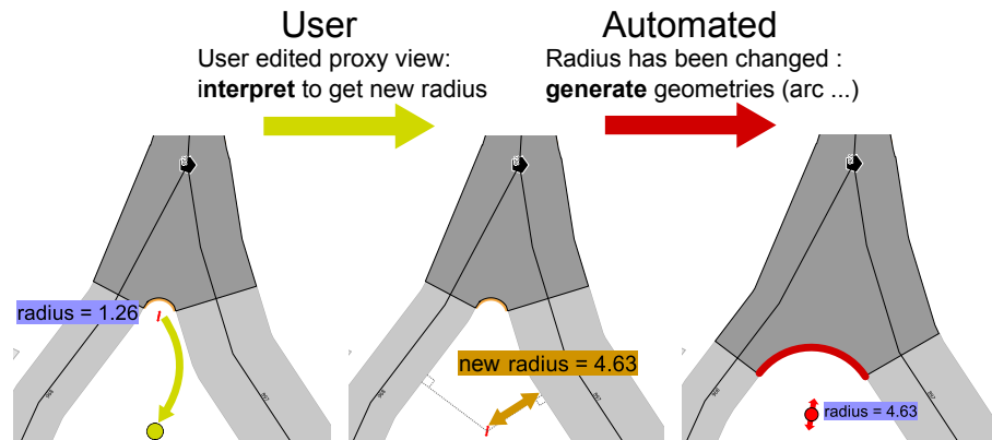
Figure 98: The curbstone arc centre is generated from the radius value and other geometries. We use it as an indirect geometric controller through a "Proxy view". The user edits the arc centre using this view, which is interpreted as a new radius. Then, another trigger re-generates arc centre and other geometries based on the new radius. No infinite cyclic trigger call occurs thanks to the proxy view which separates automated changes and user changes.
