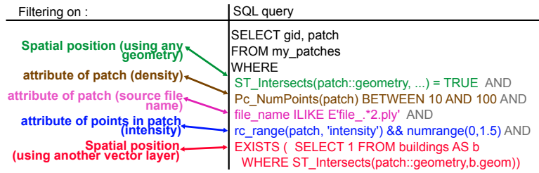
Figure 38: Example of a filtering query on patches with various type of filtering conditions.
