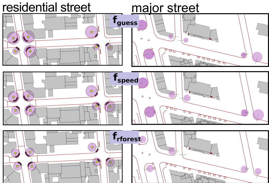
Figure 77: Illustrating radius predicted with various methods, for major and residential roads.
