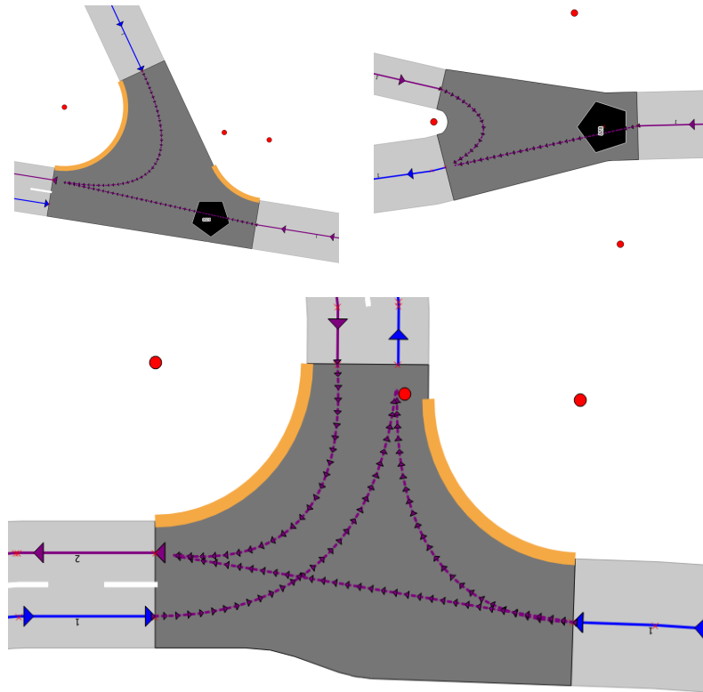
Figure 69: interconnection trajectory, Bezier curve influenced by start/end and possibly intersection centre.
