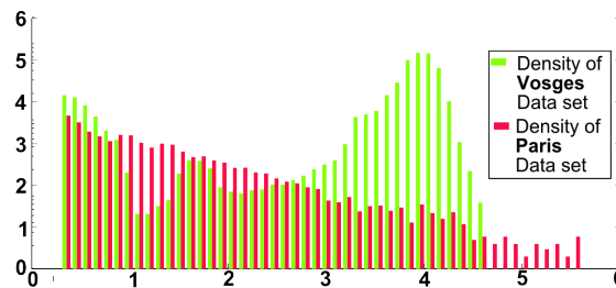
Figure 146: Histogram of number of points per patch, with a logarithmic scale for X and Y axis
