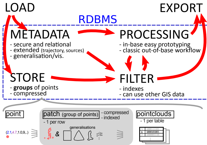
Figure 142: Overall and storage organisations of the Point Cloud Server.
