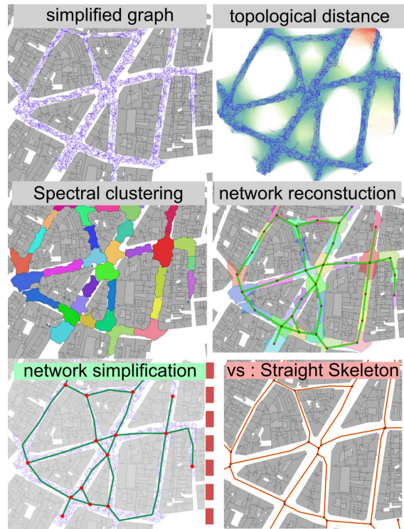
Figure 51: From simplified graph, all topological distance from a vertex to any vertices close enough are computed with PGRouting, the result is clustered using spectral clustering of Pedregosa et al., 2011. We then reconstruct the network with PostGIS Topology, and perform a final simplification step. For comparison an automated result using a straight skeleton based method.
