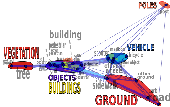
Figure 159: Result of automatic spectral clustering over confusion matrix for patch classification of Paris data set with all simple features. Edges width and colour are proportional to confusion. Manually drawn clusters for easier understanding.
