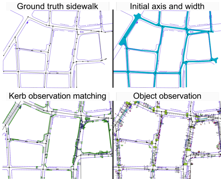
Figure 133: Input data (road axis network + width with matched observations from sensing) for optimisation in the "user" experiment area.
