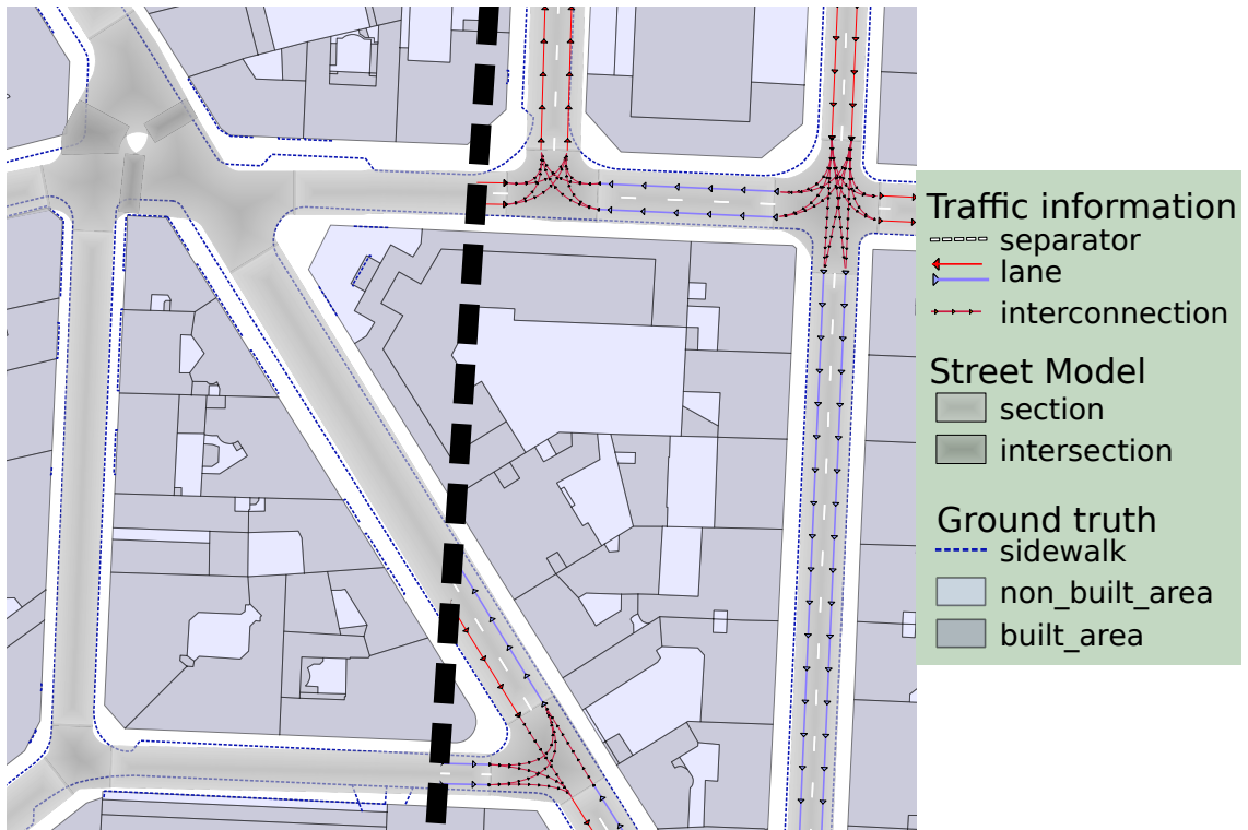
Figure 124: We use the optimised road model (kerb observation from sensing) as input to Street-Gen to generate a complete street model. Note that turning radius have not been optimised.
