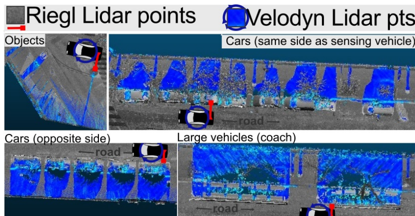
Figure 137: Point cloud sensing with static Lidar (Riegl) is occluded by cars and street objects, which hides side-walks. Adding a rotating Lidar (Velodyne) greatly reduces occlusion because the same spot can be sensed from different angles.
