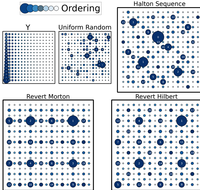
Figure 145: Several possible intra-level orders with various coverage from bad to good. Revert Morton and Revert Hilbert have offset for illustration.
