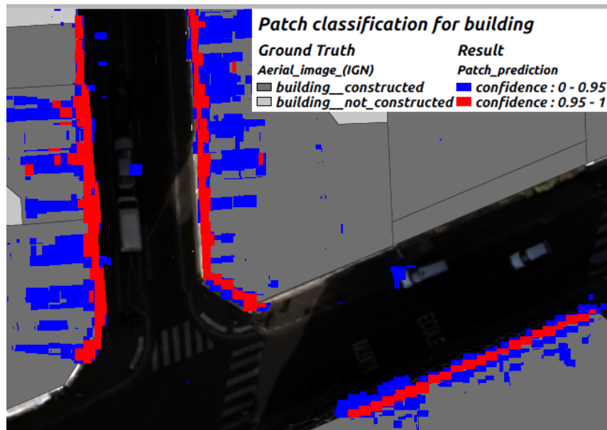
Figure 162: Plotting of patches classified as building, using confidence to increase precision. Ground truth from IGN and Open Data Paris
