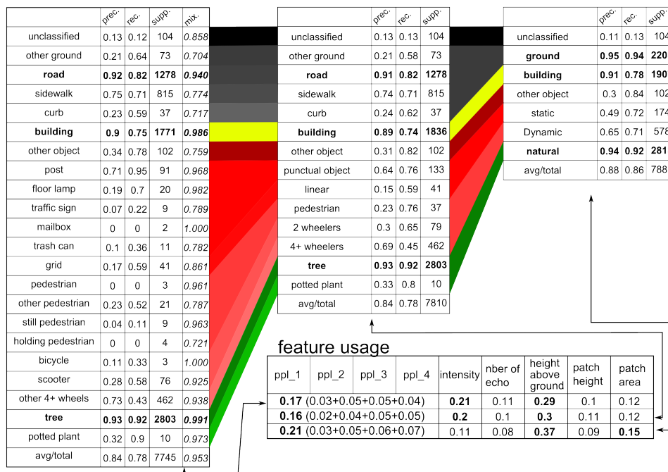
Figure 161: Results for Paris data set: at various level of class hierarchy. Precision(prec.), recall (rec.), support (sup.) and average percent of points of the class in the patches of the class, for comparison with point based method (mix.). Classes of the same type are in the same continuous tone. Feature usage is evaluated for each level in the class hierarchy.
