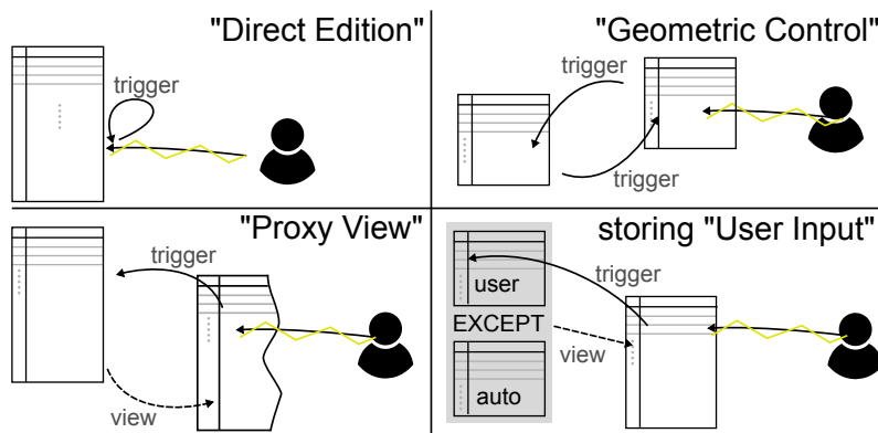
Figure 91: Various design patterns for in base user interactions. In "Direct Edition", a trigger intercepts data. In "Proxy View" a view is used as a man-in-the-middle to avoid cyclic trigger call. In "Geometric Control", another geometric object is used as a control (slider, etc.) for the targeted table. Last, storing "User Inputs" in separate table and combining it with automatically generated results solves the user input persistence problem.
