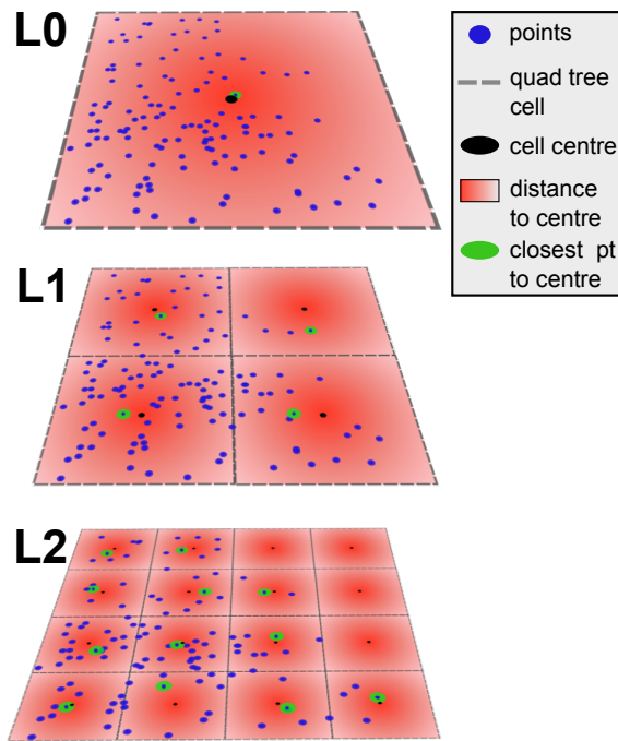
Figure 144: MidOc explained in 2D. Given a point cloud (Blue) and quad tree cells (dashed grey), the chosen point (green ellipse) is the one closest to the centre (black point) of the cell.
