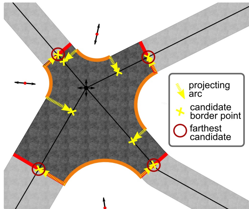
Figure 60: From circle centres, border points that limit the intersection are found by projection and filtering (farthest from intersection centre).
