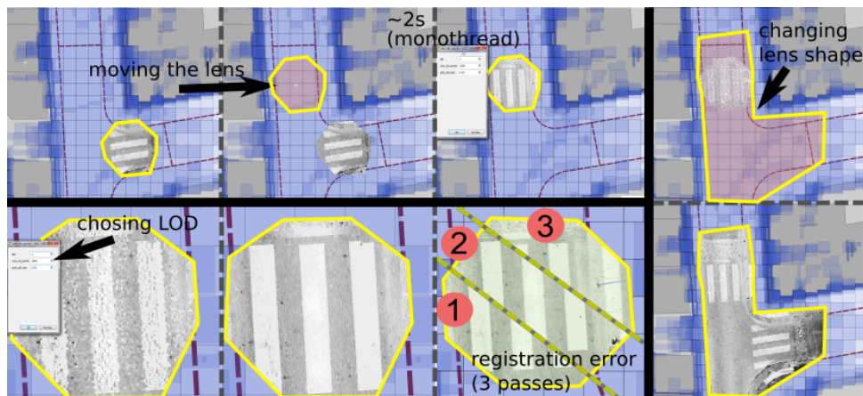
Figure 94: A GIS visualisation lens for point cloud, showed in QGIS. A lens (polygon) position and form controls what points are displayed (among several Billions points). In addition to lens geometry, lens attributes also controls other aspect of rendering, such as Level Of Detail (LOD) or the vehicle pass (temporal filtering).
