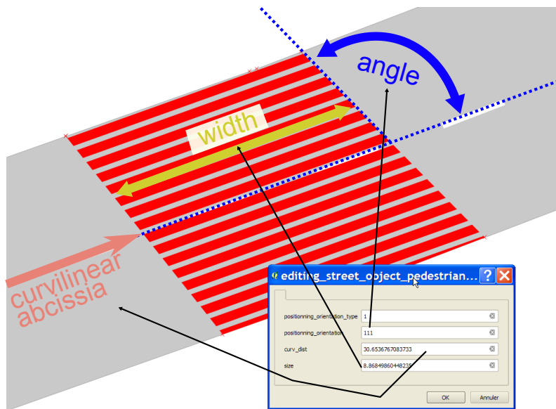
Figure 73: Specialized objects can be added, with adequate parameters (here width) and representation (here surface displayed with qgis dash pattern).
