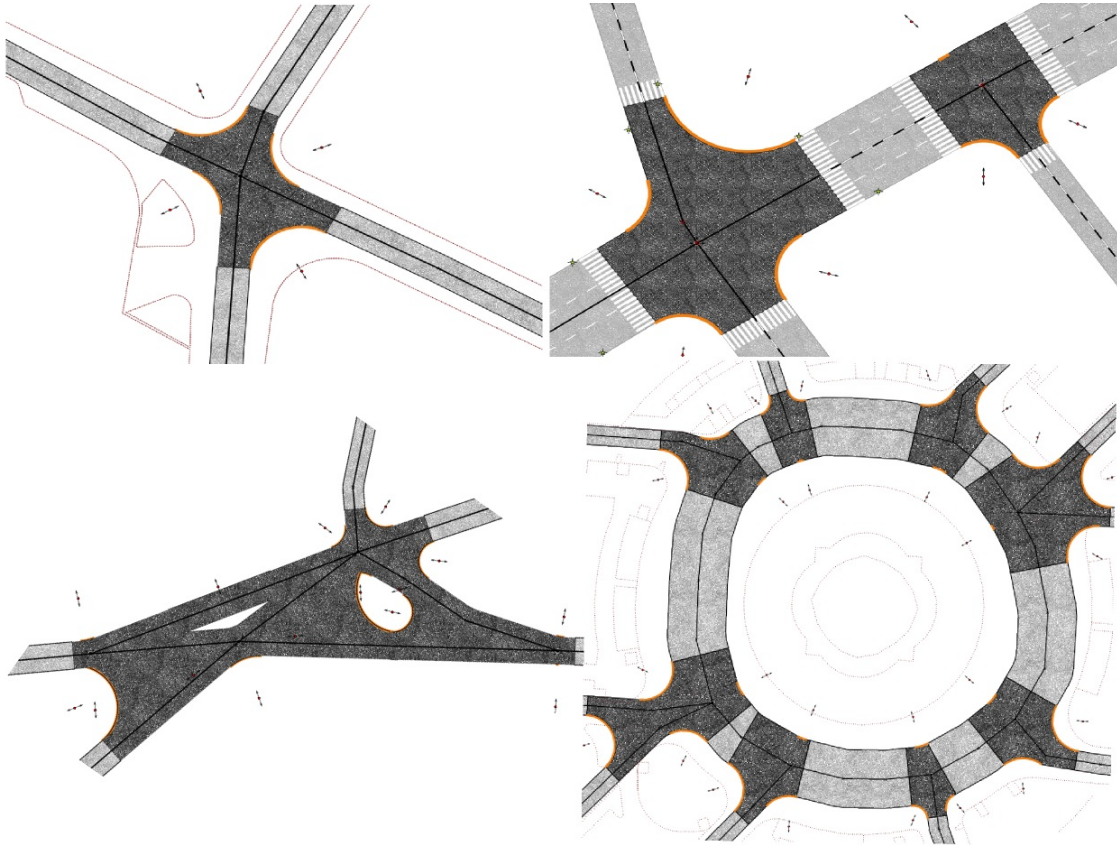
Figure 78: Example of results of increasingly complex intersection.
