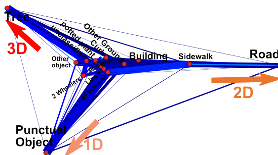
Figure 158: Spectral clustering of confusion matrix of Paris data set classification using only ppl descriptor. Edge width and colour are proportional to affinity. Node position is determined fully automatically. Red-ish arrows are manually placed as visual clues.
