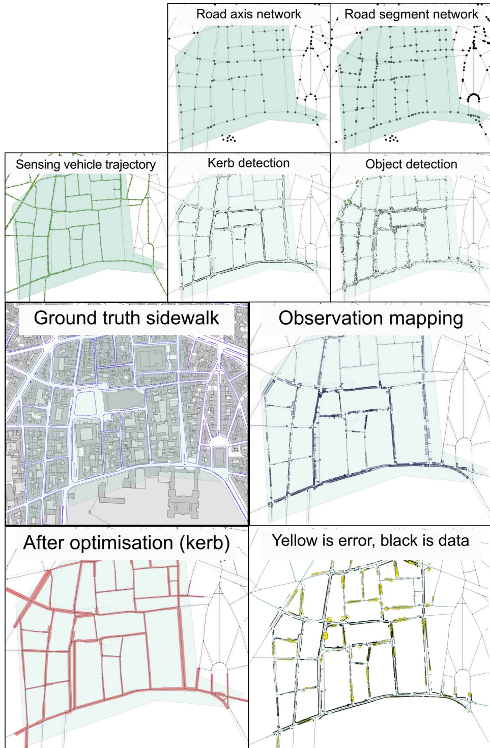
Figure 132: Optimisation parameters are the street axis network and width attribute, which get split into a road segment network. A street sensing vehicle detects kerbs and objects, which are processed into observations, and matched to street segments. Non-linear least square optimisation fits the parameters to these observations.
