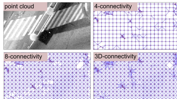
Figure 48: Classical example of possible connectivity by connecting patch centres that are closer (3D distance) than a threshold (1.4, 1.5, 1.9 metres), that is how connected is the graph.
