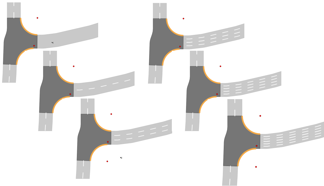
Figure 67: Generating various number of lanes, displayed in QGIS with dotted lines.
