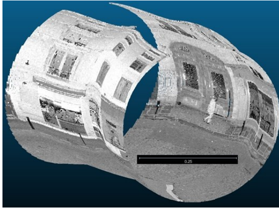
Figure 20: Lidar points can be seen as images (sensor image) as the acquisition process is regular.
