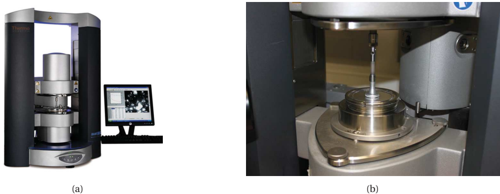
Figure 2.9 – Dynamic shear rheometer HAAKE™ MARS™ from ThermoFisher Scientific: (a) image of the complete device; (b) zoom on the area of interest during an experiment.
