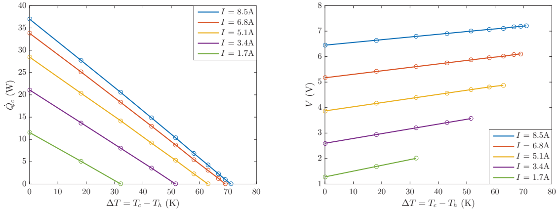
Figure 5.2 – Performances for QC-63-1.4-8.5M (Quick-Cool) at T_{h_0} = 25\text{ }^\circ\text{C} .
