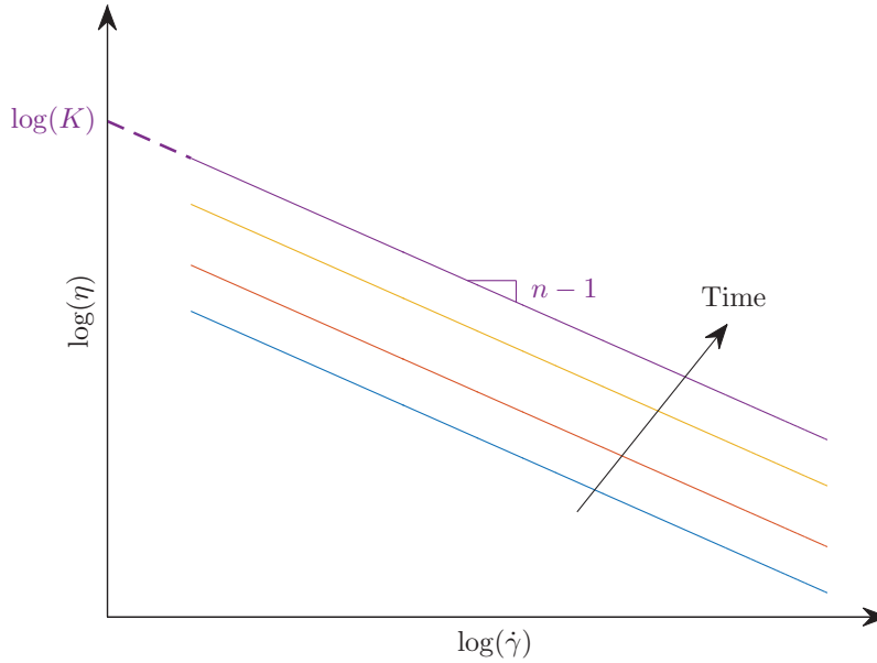
Figure 2.7 – Illustration of the Ostwald-de Waele law.
