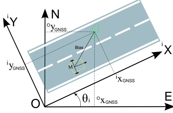
Figure 4.7: GNSS fix error and frame transformation
