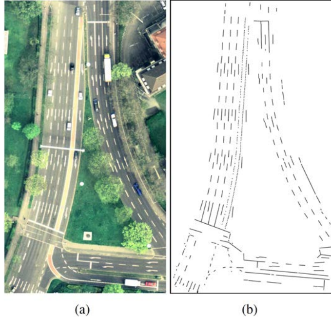
Figure 2.12: An example of the aerial image and the corresponding feature (lane marking) map used in [102]. The aerial images have a resolution of 10 cm per pixel. The resulting map is 2-dimensional. All detected lane markings are assumed to lie in one ground plane.
