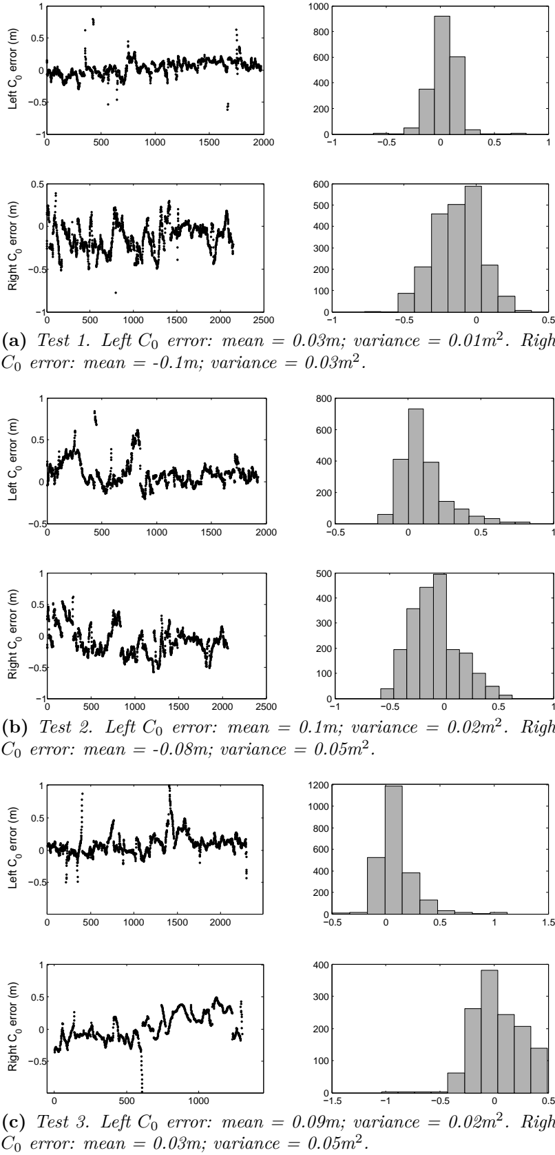
Figure 2.30: Camera C_0 measurement errors. The ground truth of C_0 is calculated by inserting the vehicle pose estimated by RTK-GPS into equation (2.32)
