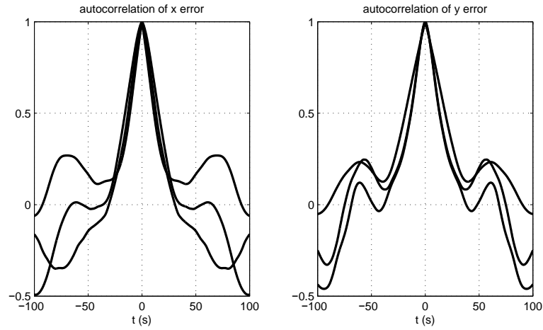
Figure 3.4: Autocorrelation of three different sequences
