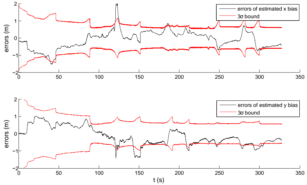
Figure 3.16: Estimated GNSS bias errors and error bounds
