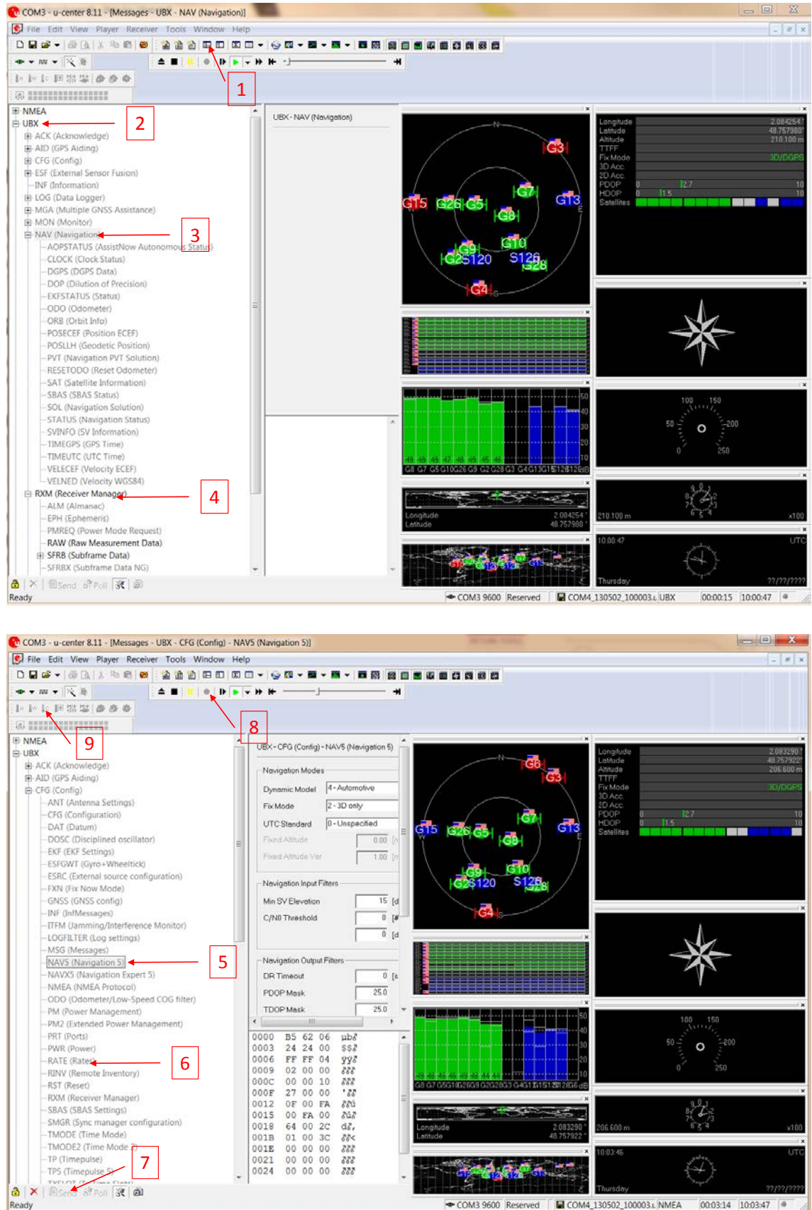
Figure B.1: Configuring u-blox receiver with UCenter
