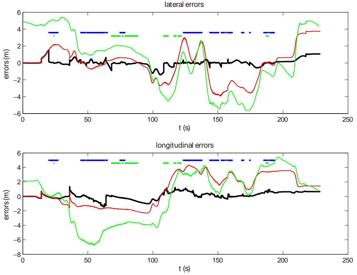
Figure A.5: Lateral and longitudinal positioning errors
