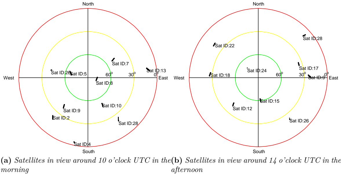
Figure 2.25: Azimuth-Elevation plot of the tracked GPS satellites during the experiments
