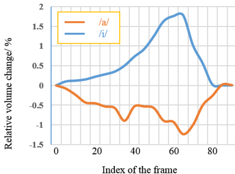
Figure 5-5 Volume change of the tongue model.
