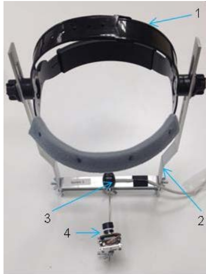
Figure 2-5 Multi-sensor Hyper-Helmet: (1) Adjustable headband. (2) Probe height adjustment strut. (3) Adjustable US probe platform. (4) Lip camera with proximity and orientation adjustment.
