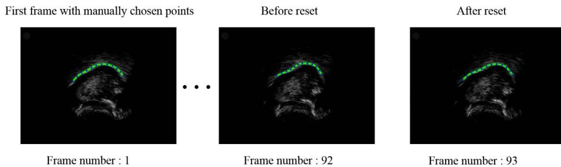
Figure 4-2 Example of automatic re-initialization in the contour tracking. As the CW-SSIM index between the first frame and the Frame 93 exceeds the threshold, the contour is re-initialized to the original position in the first frame. (The CW-SSIM index between Frame1 and frame 92 is 0.79).
