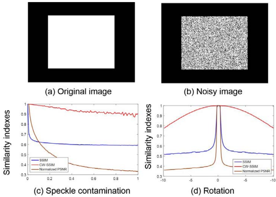
Figure 3-9 A quantitative comparison experiment was conducted on different similarity indexes using the synthetic image (the unit for the rotation is degree).
