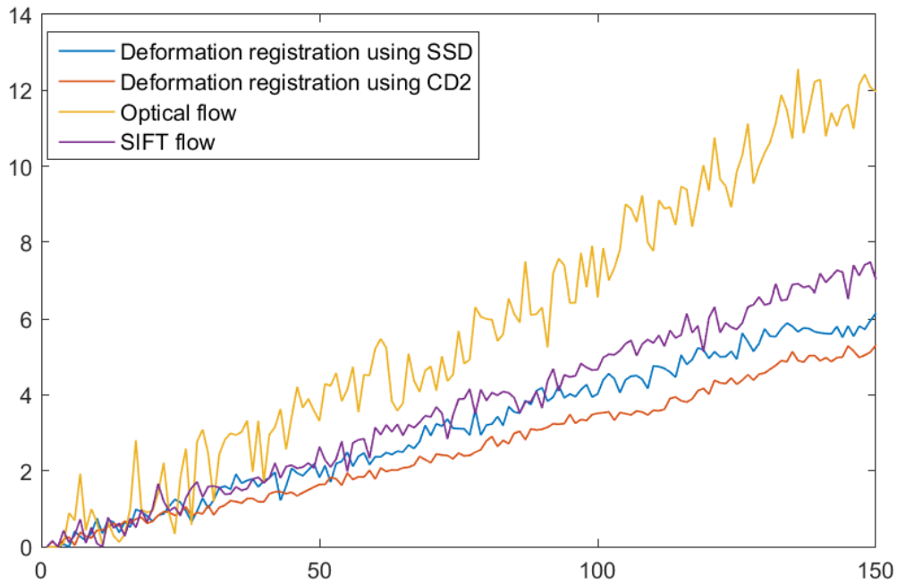
Figure 3-7 The MSD error of different speckle tracking methods.
