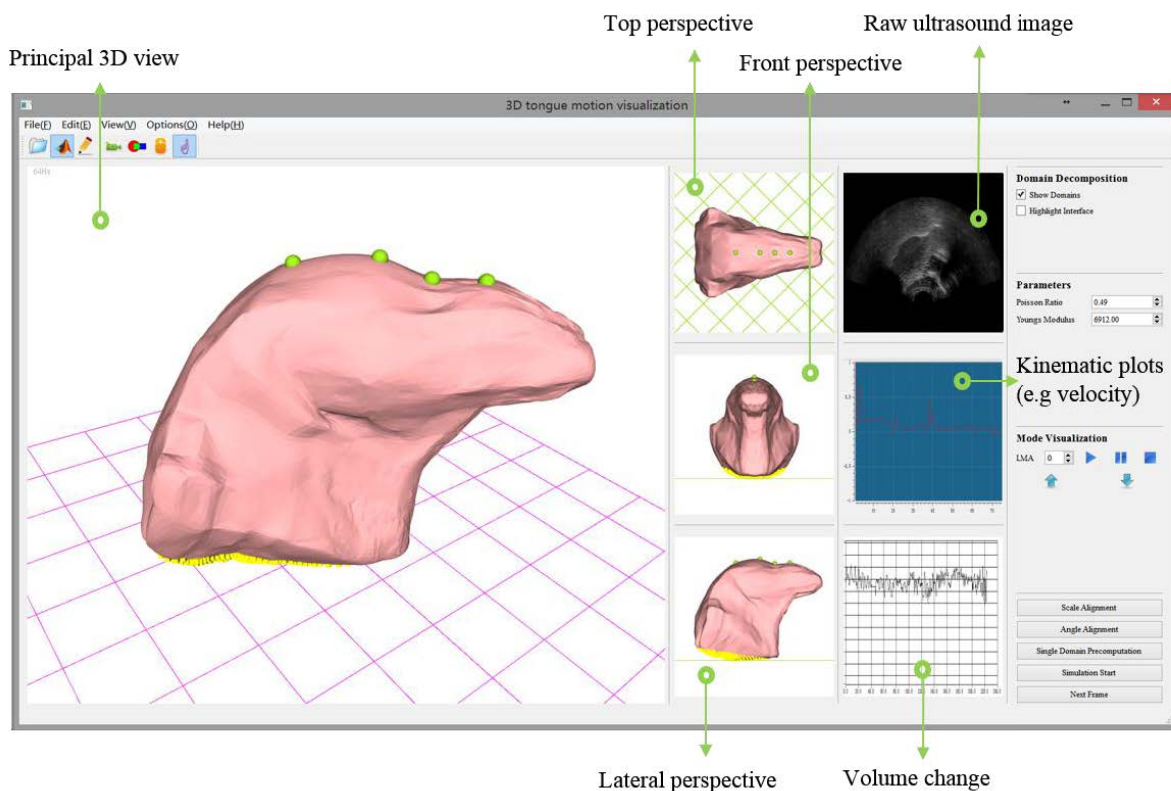
Figure 5-1 A snapshot of the user interface of the platform being developed.
