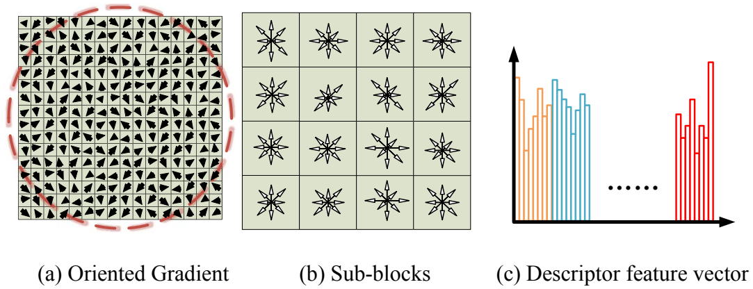
Figure 3-4 Describe the keypoints by using the feature vector.
