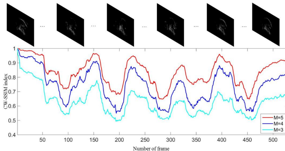
Figure 3-11 CW-SSIM index of the entire image in an ultrasound image sequence of five utterances of phoneme /k/. Three different levels of decomposition M are shown.
