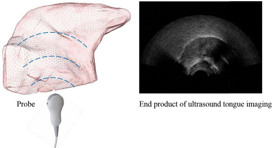
Figure 2-3 Ultrasound-tongue imaging.
