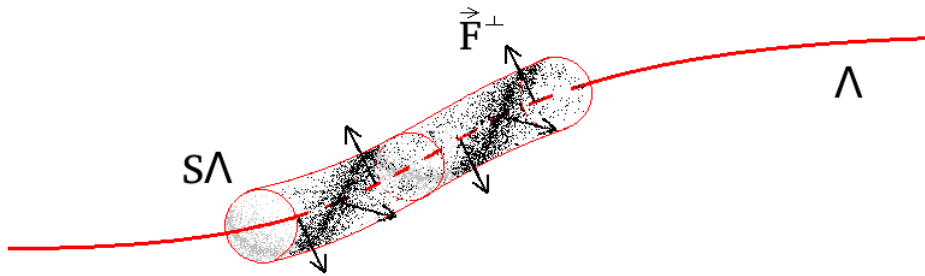
Figure 3.3.1: Above, we depict \Lambda encircled by its normal bundle in sphere S\Lambda (with fibres S_\sigma \Lambda = N_\sigma \Lambda / \mathbb{R}_+^* ). The mass concentration given by \nu is represented by the more or less strongly shadowed regions, and is directed by the normal force \vec{F}^\perp which is spinning around \Lambda in the example. Here, we took F(\sigma) = 1 and \nabla g(\sigma) = \mathbb{1} .
