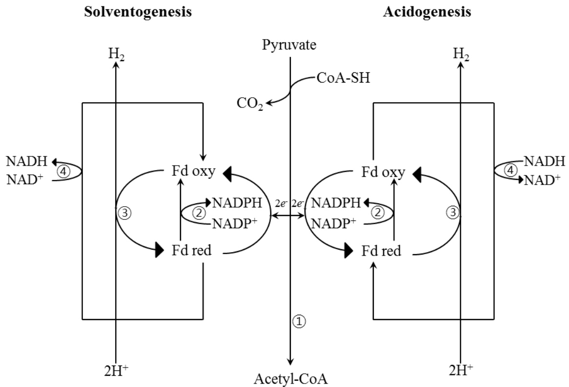
Figure 1.2. The breakdown of pyruvate to acetyl-CoA and electrons flux in C. acetobutylicum . ①Pyruvate ferredoxin oxidoreductase; ②Ferredoxin NADPH oxydoreductase; ③Hydrogenase; ④Ferredoxin NADH oxydoreductase
