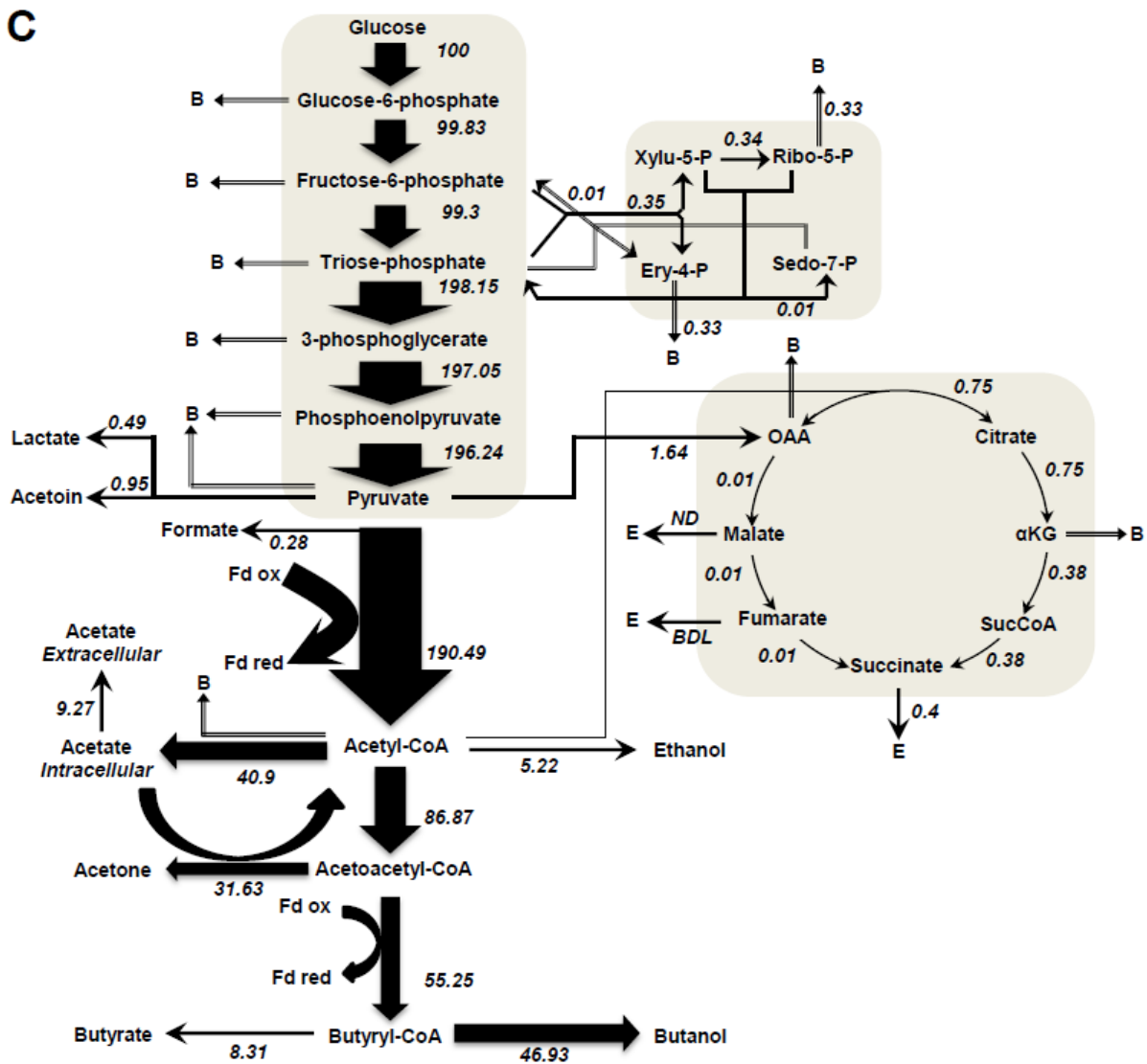
Fig.S4.2 Metabolic flux map of control and \Delta buk\Delta ptb300 strains under three metabolic states. (A) control under acidogenesis, (B) \Delta buk\Delta ptb300 under acidogenesis, (C) control under solventogenesis, (D) \Delta buk\Delta ptb300 under solventogenesis, (E) control under alcohologenesis, (F) \Delta buk\Delta ptb300 under alcohologenesis. All values are normalized to the flux of the initial carbon source (mmol/gDCW/h). Glucose flux is normalized as 100 for acidogenesis and solventogenesis, and the sum of glucose and half of the glycerol normalized as 100 for alcohologenesis. 2-KV, 2-keto-valerate; 2-HV, 2-hydroxyl-valerate.
