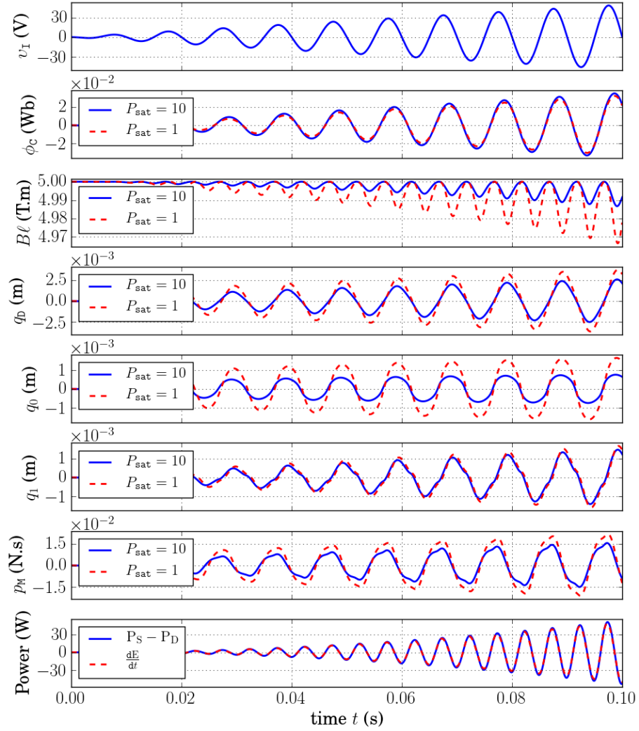
FIGURE 7.10 : Simulation of the model 1 in table A5 depicted in figure 7.10, for the parameters in tables A11 and A12 (except P_{\text{sat}}^{\text{S}} indicated in the legend). The input voltage is a 100Hz sine wave with increasing amplitude between 0V and 50V. The sampling rate f_s = 96\text{kHz} . The power balance is shown for P_{\text{sat}}^{\text{S}} = 10 only. Notice q_{\text{D}} = q_0 + q_1 .
