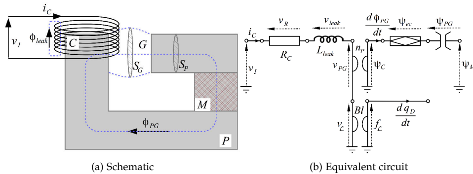
FIGURE 7.11 : Simplified modeling of the electromagnetic circuit, which includes : the coil wire resistance R_c , the linear inductance associated with the leakage flux \phi_{1eak} , the electromagnetic transduction with n_p the number of wire turns around the magnetic path, the magnetic energy storage in the ferromagnetic path described by the nonlinear induction–excitation curve \psi_{PG} \equiv \psi_{PG}(\phi_{PG}) from (C22), the fractional dynamics associated with eddy currents in the pole piece form (C33), and the constant source of magnetomotive force \psi_M due to the magnet from (C24).
