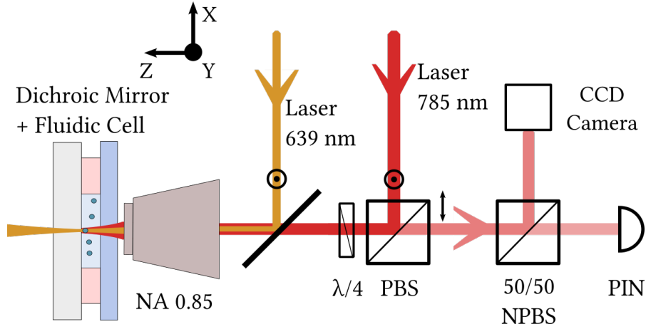
Figure 4.15: Schematic setup of the experimental configuration used to apply an external force on a trapped bead in a bistable potential. The gold mirror is replaced by a 0^\circ dichroic mirror used to form a SWOT with the 785 nm (Excelsior, 45 mW) laser beam. A second beam at 639 nm (Thorlabs laser diode, 70 mW) is inserted collinear to the trapping beam by a 45^\circ dichroic mirror. This second beam is modulated at a given amplitude and frequency acting as the external driving force.
