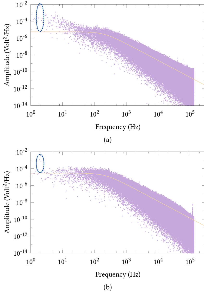
Figure 4.19: Power spectral density of a 1 \mu\text{m} melamine bead trapped in a bistable potential under the influence of an external sinusoidal drive at 2 Hz. Panel (a) displays the PSD calculated from the PIN signal. Panel (b) the transverse PSD acquired via the QPD.
