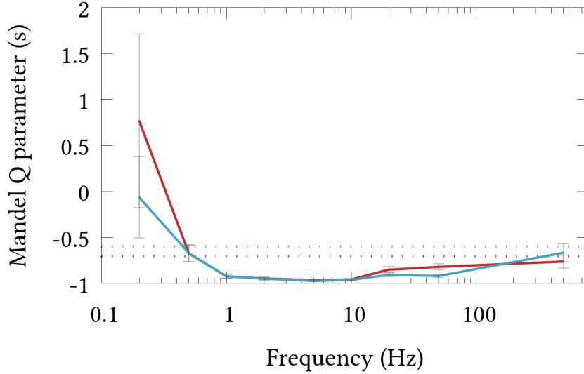
Figure 4.20: Evolution of the Mandel Q factors for the upper and lower state residency times. A 1\text{ }\mu\text{m} melamine bead is trapped in a rest symmetric bistable potential and the frequency of the external drive is changed while the amplitude remains constant. The blue curve represents the lower state and the red curve the upper state. The dotted lines display, in the same color code, the values Q_{\text{rest,down}} \simeq -0.6 (blue) and Q_{\text{rest,up}} \simeq -0.7 (red) of the rest Mandel factors.
