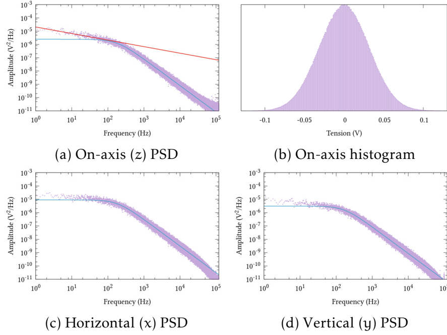
Figure 5.10: Power spectral densities along the 3 spatial axis for a trapped chiral NPy. Signals are taken from different detectors, the QPD for the transverse horizontal/vertical (x/y) components and the PIN photodiode for the axial z component. The pink curves represent the intensity PSDs averaged 8 time (for the sake of visibility). The blue curve gives the best Lorentzian fit of the data. The red line in panel (a) gives the best fit of the data on the low frequency part of the spectrum (from 1 to 200 Hz). The slope associated with the fit is -0.5 . The intensity histogram along the optical axis shows a Gaussian like distribution of positions, meaning that the chiral NPy is well localized in space, and therefore well trapped.
