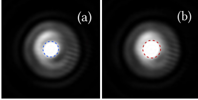
Figure 2.6: Recollected spots imaged on the CCD camera in the case of a bead trapped in a bistable configuration, with same exposition time. Panel (a) shows the bead in its most distant position from the mirror, i.e. the position behind the waist ( z < 0 ). Panel (b) shows the bead in front of the waist, thus closer to the mirror. The recollected intensity is higher near the mirror (image (b)) than away from it. The central area of the recollected spot is indicated by the superimposed circles, with a 44 pixel-diameter for (a) and 50 for (b).
