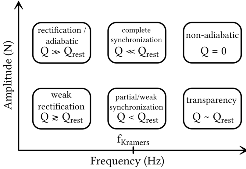
Figure 4.7: Diagram illustrating the different statistical regimes that a bead can explore in a bistable potential as a function of the external drive frequency and amplitude. These regimes are simply characterized by their Mandel Q factor with respect to Q_{\text{rest}} , the Mandel factor of the initial unperturbed bistable potential.
