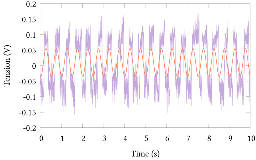
Figure 4.17: Experimental time-trace of 10 s recorded by the PIN photodiode. A 1\text{ }\mu\text{m} melamine bead is trapped in a bistable potential under an external drive at 2 Hz. The bead dynamics is strongly synchronized with the external displayed in orange.
