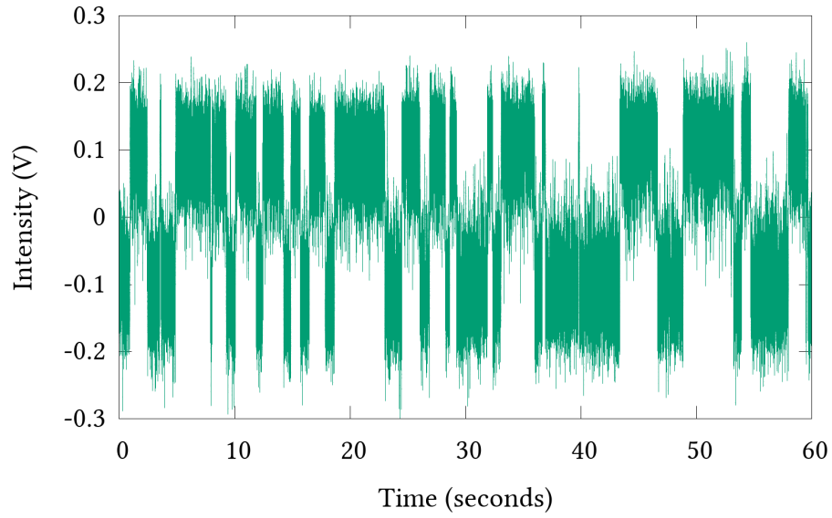
Figure 2.7: Time trace associated with a bistable motion of the bead as recorded by the PIN photodiode on the reflected beam intensity. The acquisition time is set to 60 s, at a rate of 262 kHz.
