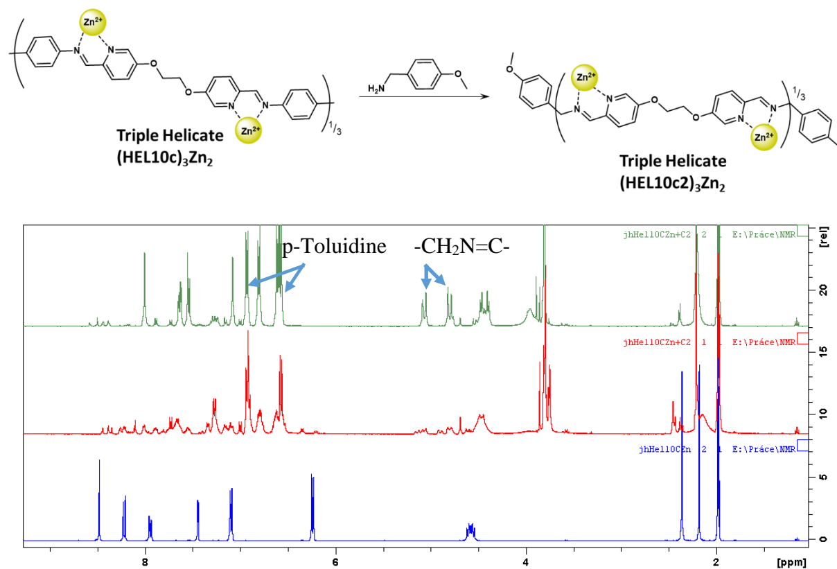
Figure E3.9.: The 1 H NMR (CD 3 CN) spectra of (\text{HEL10c})_3\text{Zn}_2 exchange process with 4-methoxybenzylamine. Bottom: (\text{HEL10c})_3\text{Zn}_2 (Triple helicate); Middle: freshly mixed (\text{HEL10c})_3\text{Zn}_2 + 4-methoxybenzylamine; Top: Newly formed triple helicate with 4-methoxybenzylamine (marked a new set of enantiotopic benzylic protons) and free p -toluidine
