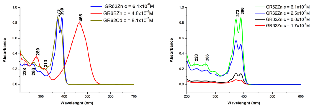
Figure 3.29: Left: Absorption spectra of GR62Zn (blue), GR62Cd (green) and GR6BZn (red). Right: Absorption spectra of GR62Zn at various concentrations.
