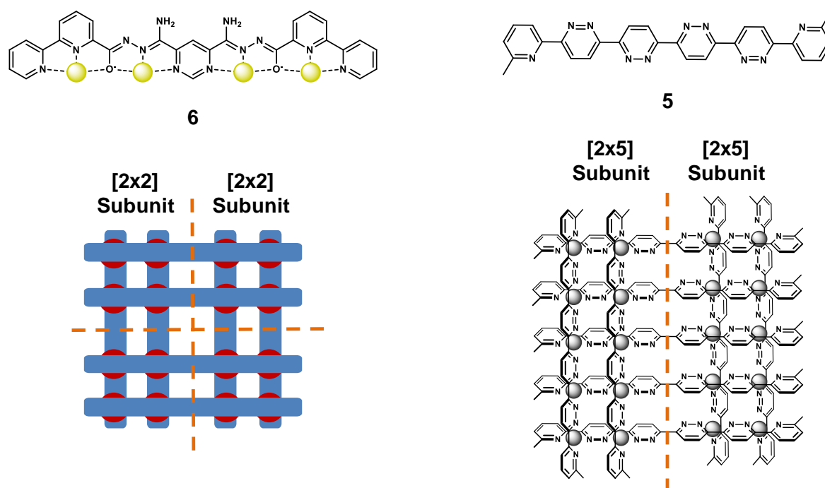
Figure 3.6: Illustrative examples of “grid of grids” assemblies with their respective ligands
