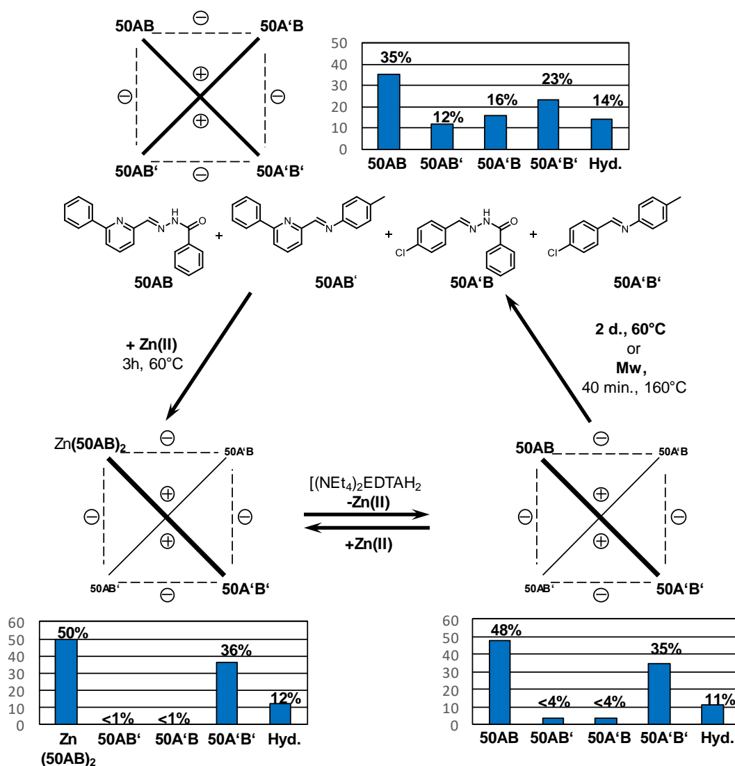
Figure 2.11: Formation of the Zn-trained DCL distribution by addition of Zn(OTf) 2 to the mixture of the four constituents 50AB, 50A'B', 50A'B and 50AB' (training; left top to bottom), which on cation removal retains its composition in the metal-free DCL obtained (information storage; bottom, left to right); recall by addition of zinc(II) (bottom, right to left) and erasing of the metal-free DCL by heating (right bottom to top) with return to the thermodynamically driven initial state. Mw = microwave irradiation
