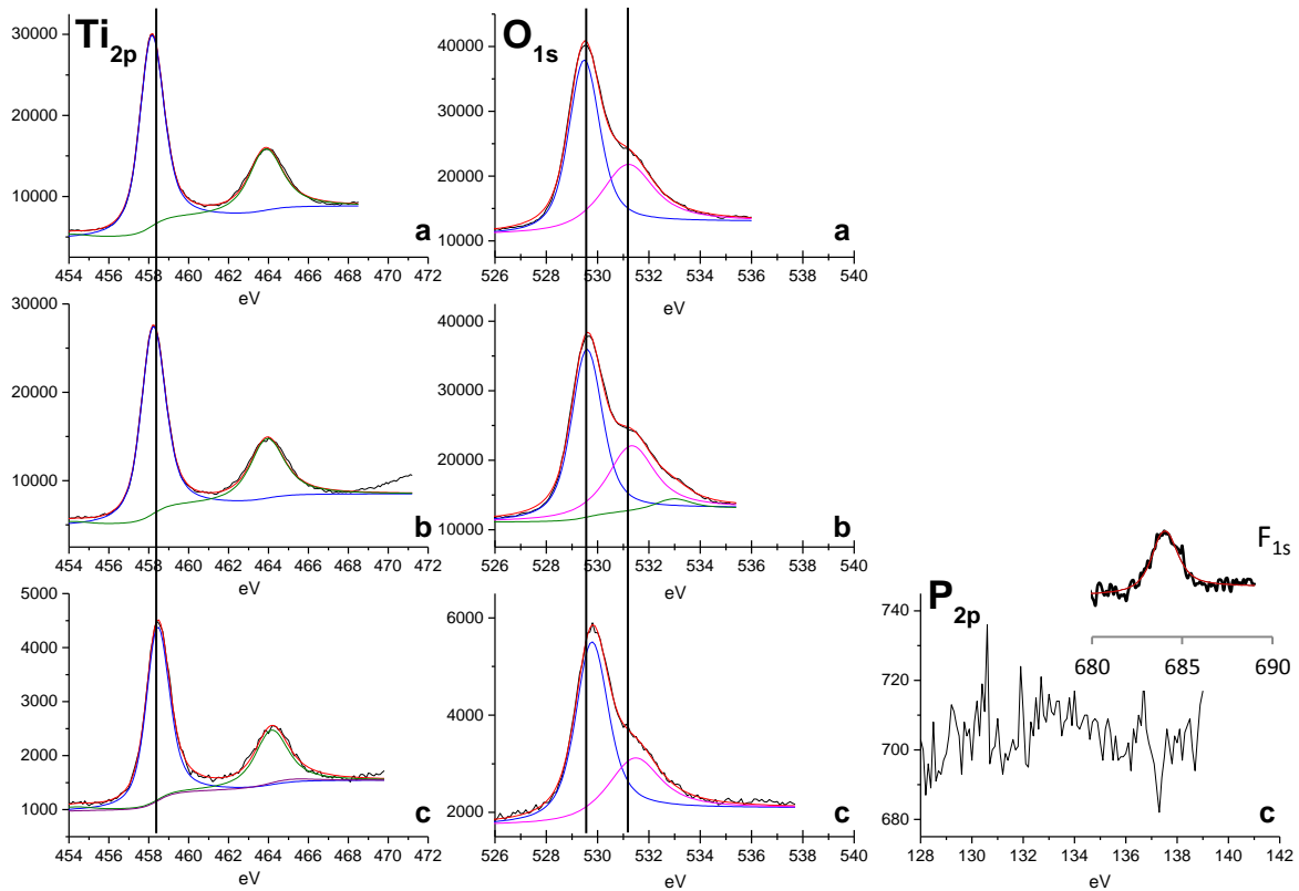
Fig 29: Ti 2p , O 1s and P 2p XPS patterns of dried TiO 2 samples with different BmimPF 6 /Ti ratio in the sol-gel synthesis: 0 (a), 0.03 (b) and 0.4 (c). The acid used was HAc and the aging duration was fixed at 6 days.
