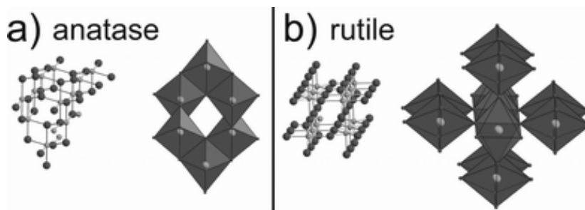
Fig 9: Crystalline structure of \text{TiO}_2 and the distorted octahedron (a) edge-sharing for anatase and octahedron (b) corner-sharing for rutile
