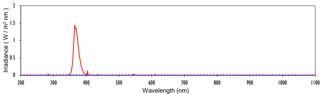
Fig 55 : Irradiance spectra of the UVA lamp used in this work.
