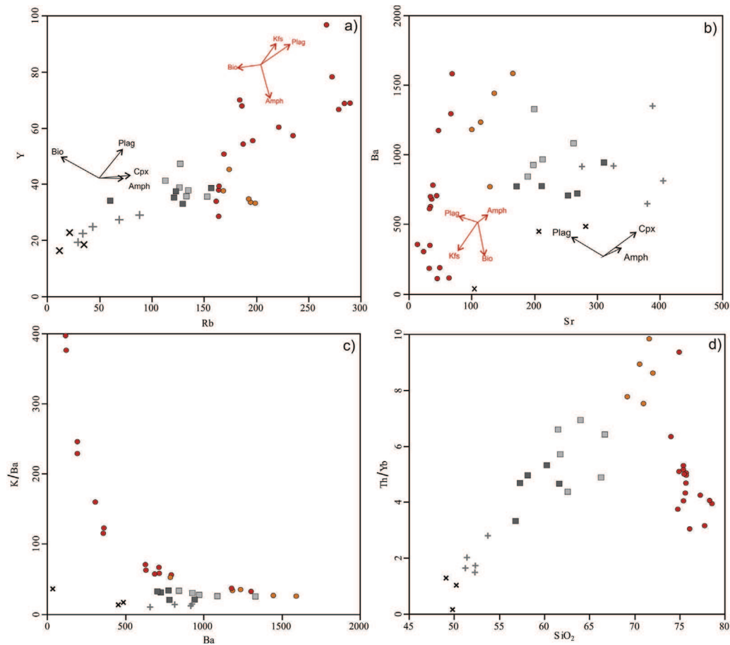
Fig. 11. Variation diagrams with calculated fractionating vectors for felsic and mafic dikes. a) Rb vs. Y; b) Sr vs. Ba; c) K/Ba vs. Ba diagram; d) Th/Yb vs SiO 2 diagram. Symbols as in Fig. 5.
