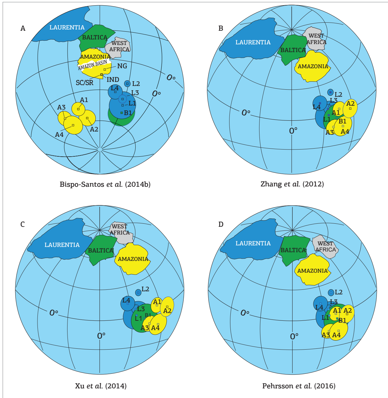
Figure 6. Comparison of Mesoproterozoic poles from the Amazonian Craton, Laurentia, and Baltica considering the reconstruction of Columbia proposed by (A) Bispo-Santos et al. (2014b); (B) Zhang et al. (2012); (C) Xu et al. (2014); and (D) Pehrsson et al. (2016) (based on D'Agrella-Filho et al. 2016). Mesoproterozoic paleomagnetic poles, and their confidence circles ( \alpha_{95} ): Amazonia – (A1) Rio Branco Sedimentary rocks; (A2) Salto do Céu sills; (A3) Nova Guarita Dykes; (A4) Indaivaí Intrusive (Tab. 1); Baltica – (B1) 1460 Ma mean pole (Bispo-Santos et al. 2014b); Laurentia – (L1) 1460 Ma mean pole; (L2) McNamara pole ( 1401 \pm 6 Ma); (L3) Electra Lake Gabbro ( 1433 \pm 2 Ma); (L4) Laramie Anorthosite ( 1429 \pm 9 Ma) (Bispo-Santos et al. 2014b). Euler rotation poles used for paleomagnetic poles and cratonic blocks as in D'Agrella-Filho et al. (2016). Geographical positions of Salto do Céu sills (SC), Rio Branco sedimentary rocks (SR), Indaivaí Intrusive (IND) and Nova Guarita Dykes (NG) are shown in (A).
