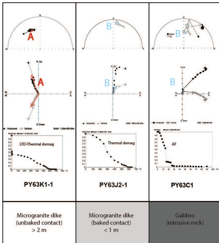
Figure 6.10: BCT-2. Localization in Figure 6.8. Figure shows stereographic projections (solid (open)) symbols represent positive (negative) inclinations), normalized intensity curves and Zijdeveld diagrams.
