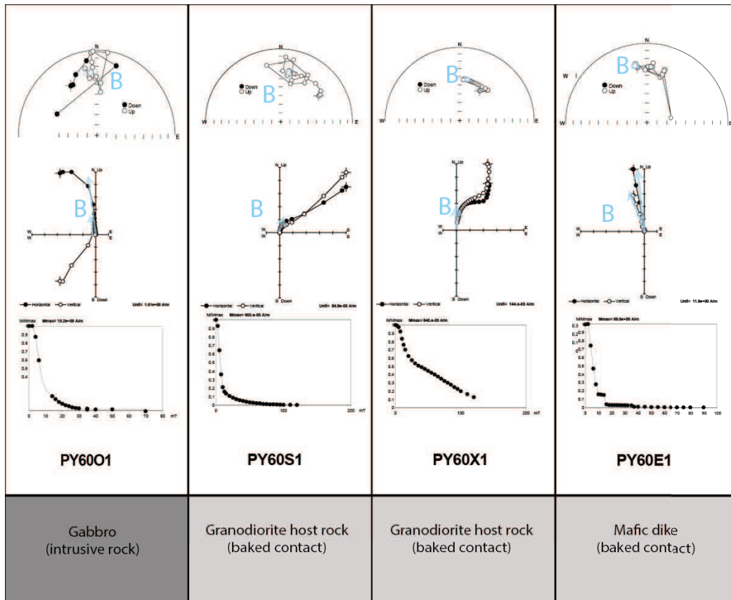
Figure 6.9: BCT-1. Localization in Figure 6.8. Figure shows stereographic projections (solid (open)) symbols represent positive (negative) inclinations), normalized intensity curves and Zijdeveld diagrams.
