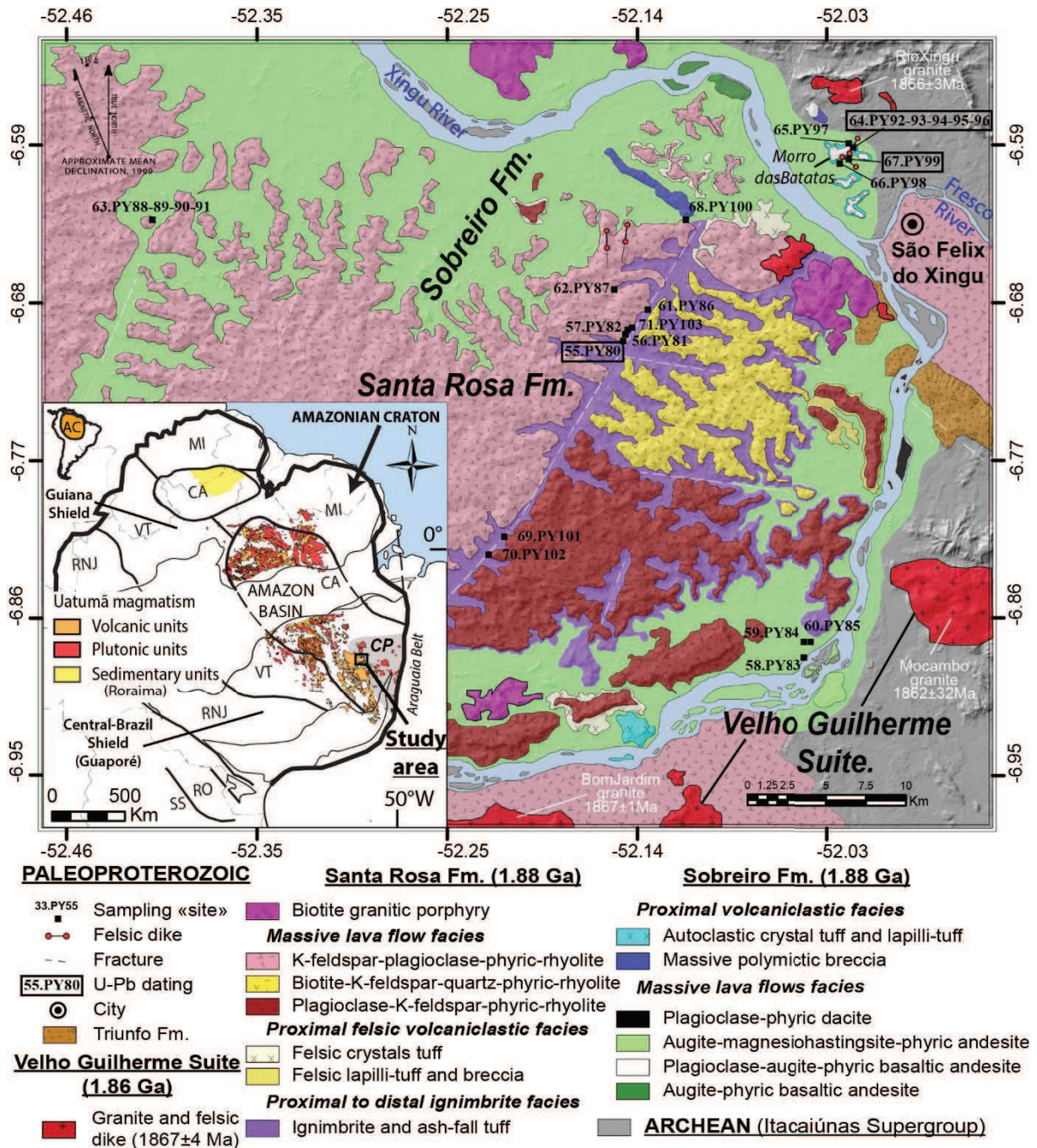
Figure 7.1: Geological map of São Felix do Xingu region with location of sampling sites (Full Square) for Santa Rosa and Sobreiro Formations (adapted from Juliani and Fernandes (2010)). Inset: The ~1880 Ma volcano-plutonic Uatumã event and the main tectonic provinces of the Amazonian craton (adapted from Cordani and Teixeira (2007)). Abbreviations: CP = Carajás Province (in grey); CA = Central Amazonian Province; MI = Maroni-Itacaiunas Province; VT = Ventuari-Tapajós Province; RNJ = Rio Negro-Juruena Province; RO = Rondonian-San Ignácio Province; SS = Sunsás province.
