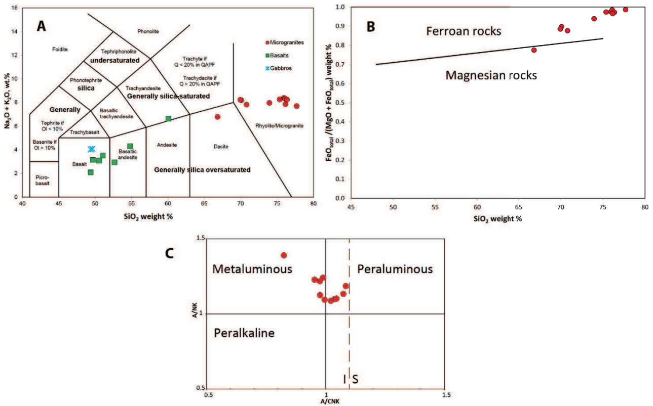
Figure 5.15: A: TAS diagram (Le Maitre et al., 2002). B: Major element variation diagrams showing the range of compositions, FeO_{tot} / (FeO_{tot} + MgO) . (Frost et al., 2001; Frost and Frost, 2008). C: Shand diagram, A/NK vs. A/CNK plot (Maniar and Piccoli, 1989).
