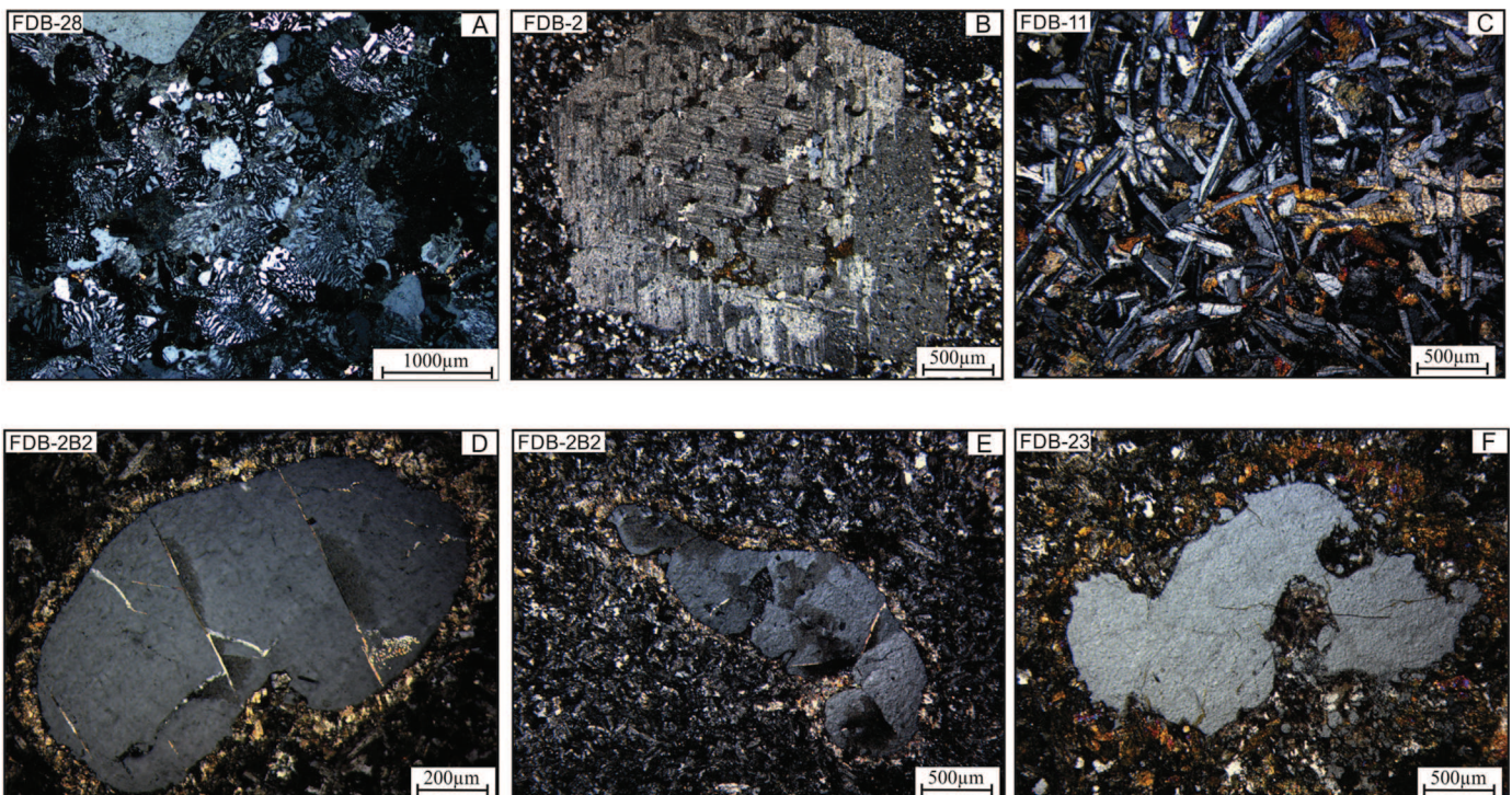
Fig. 4. Microtextural aspects of the Tucumã dikes: A) Radiate fringe and vermicular granophyric texture in rhyolite and an aggregate of quartz forming the glomoporphyritic texture; B) K-feldspar phenocryst with rapakivi texture; C) Subophitic texture, common feature of mafic dikes; D, E, F) Corona texture in quartz crystals with different degrees of embayment/engulfment.
