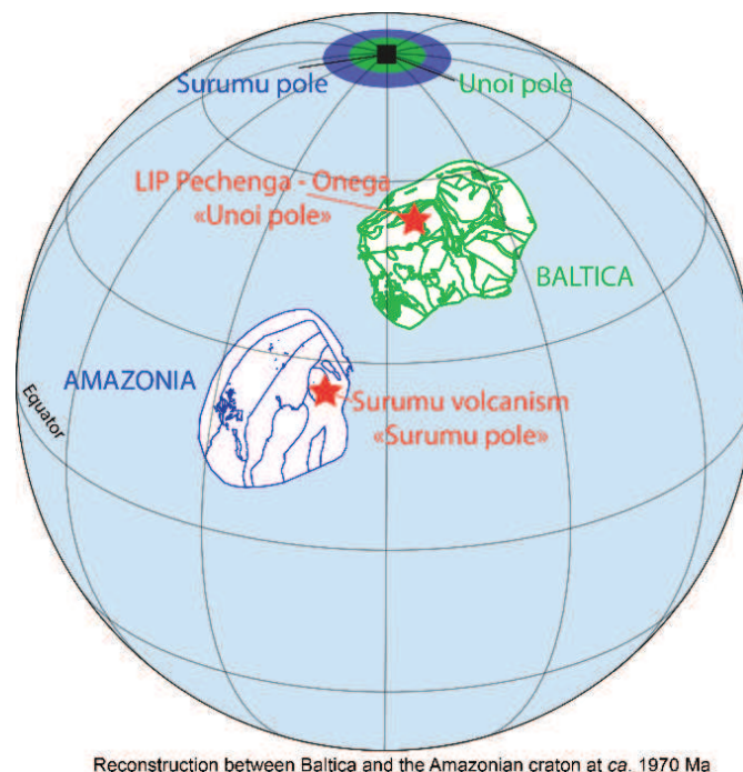
Figure 1.20: Possible reconstruction for the Amazonian craton and Baltica at ca. 1970 Ma.
