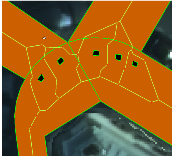
Figure 5.17: Straight skeleton centerlines for a real physical surface with obstacles (objects rendered in black are obstacles).
