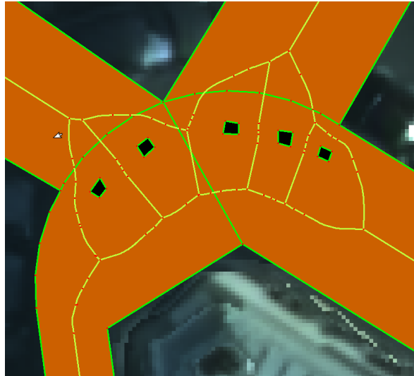
Figure 5.15: Medial axis centerlines for a real physical surface with obstacles (objects rendered in black are obstacles).
