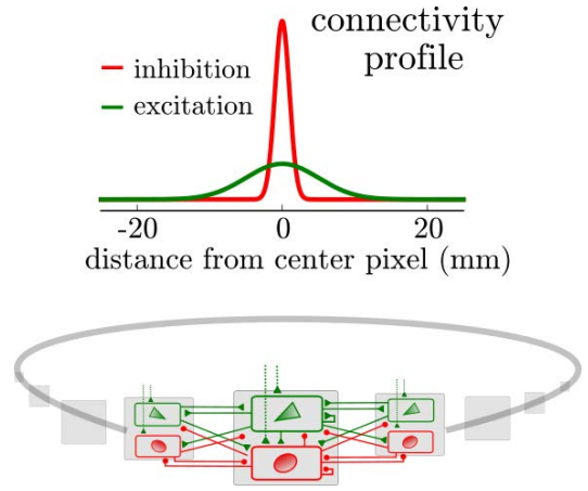
Figure 9: A spatial model of the cortical sheet. The balanced network units are embedded in a ring geometry. The lateral connectivity follows two Gaussian profile of extent l_{exc}=5\text{mm} and l_{inh}=1\text{mm} for the excitation and inhibition respectively.
