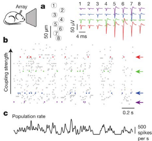
Figure 4: Spontaneous activity in awake mice visual cortex exhibits strong fluctuations of population activity. (a) Schematic of a single shank of silicon electrode array, and spike waveforms of four example wide-spiking neighbor neurons measured with the array in deep layers of V1 of an awake mouse. (b) Population raster of spontaneous activity in 66 neurons recorded from the whole array. (c) Population rate measured by summing all the spikes detected on the entire array (both well-isolated units and multi-unit activity) with 1ms resolution and smoothed with a Gaussian of half-width 12ms (N.B. the smoothing can be seen as a way to reduce the narrow sampling of the population). Reproduced from Okun et al. (2015).
