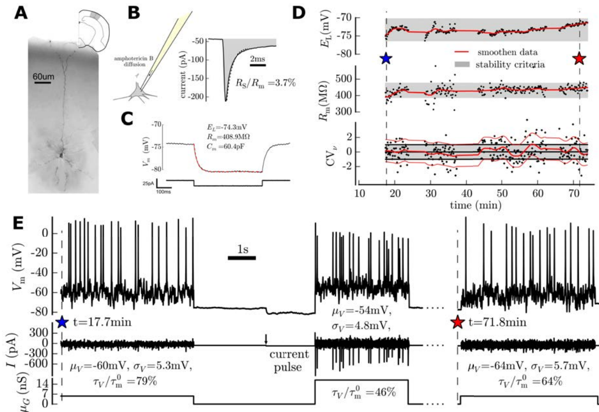
Figure 4: The exploration of a physiologically-relevant space in layer 5 pyramidal neurons of juvenile mice. From B to E , an example of a single cell. (A) A typical layer 5 pyramidal neuron in the primary visual cortex of juvenile mice. Picture from additional experiments: marking with 2% Biocytin (Sigma Aldrich) in whole cell configuration. (B) After diffusion of the perforant molecule toward the patch of membrane, a step voltage clamp protocol estimates the quality of the seal and perforation (see details in the Methods IV.2 ). (C) A step current clamp protocol estimate the passive membrane properties. Those properties are used by the stimulation protocols to constrain the V_m fluctuations (see Methods IV.7 ). (D) All along the recording, we monitor the cellular properties: the resting membrane potential E_L , the membrane resistance R_m and the variations of the firing rate with respect to the stationary behavior CV_\nu (see details in the main text V.5 and in the Methods IV.8 ). The smoothed data (red curve) show the global trend, it removes the measurement error due to the short sampling time for R_m and E_L (see E ), for CV_\nu , it removes the intrinsic spiking irregularity. For the CV_\nu curve we have added the standard deviation (mean \pm std in red) for comparison with a stationary Poisson process (mean \pm std in black). (E) Sample of the membrane potential V_m , the injected current I and the total conductance \mu_G at the beginning of the recording (left, t=17.7 min, blue star in D ) and one hour after (right, t=71.8 min, red star in D ). Within an episode, we scan one combination of the (\mu_V, \sigma_V, \tau_V^N) variables. For example, the middle episode corresponds to the most depolarized level \mu_V (hence the lower spike amplitude due to Na inactivation) with the fastest fluctuations \tau_V^N (i.e. an high input conductance \mu_G , also shunting the spikes, see the strong opposite current) and an intermediate variance \sigma_V . In between the two first episodes, one can see rest period (to monitor E_L ) followed by a current pulse (to monitor R_m ).
