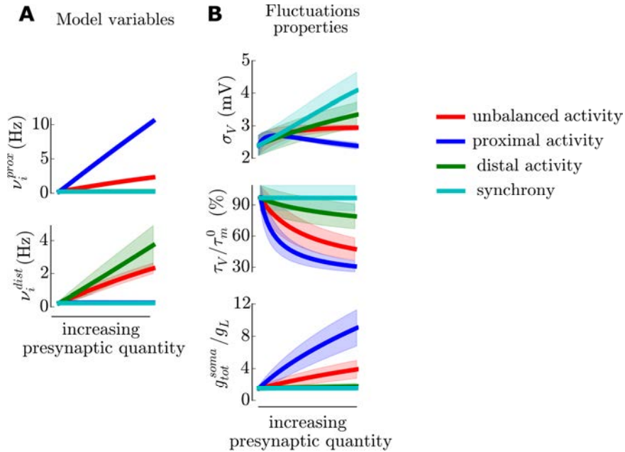
Figure 2: Variability in the fluctuations properties introduced by the different morphologies. Showing only the quantities that vary across cells, all other variables ( \nu_e^p , \nu_e^d , s ) or \mu_V are fixed across cells. (A) Model variables. The balance \mu_V is adjusted for each cells and the cells have different surfaces, so different number of synapses (and especially different ratio of excitatory to inhibitory numbers) so the inhibitory activity is adjusted differently for each cell. (B) Fluctuations properties.
