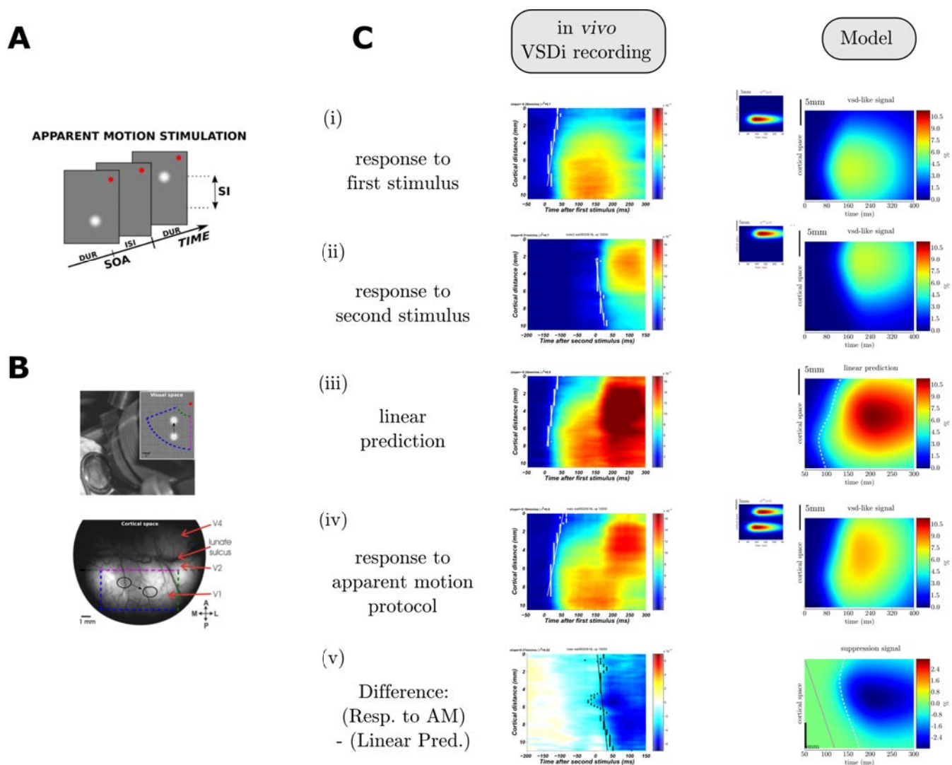
Figure 11: Deintricating the cortical operation underlying the response to an apparent motion (AM) stimulus: comparison between the model and VSDi recordings in fixating monkeys. (A) The apparent motion protocol. During a single trial, the monkey had to fixate on a central red dot for 1–2s. The animal’s gaze was constrained in a window of 2^\circ \times 2^\circ . Two Gaussian blob stimuli (each of 0.5^\circ spatial extent) at two different position were successively presented during fixation. (B) VSDi allows for a real-time visualization of large neuronal population in primary visual cortex of fixating monkeys. (C) To deintricate the cortical computation, both in the theoretical model and in fixating monkey in vivo , we show the VSDi signal of different quantities: (i) the response to the first stimulus alone (ii) the response to the second stimulus alone, (iii) the linear prediction of the signal resulting from the two stimuli alone, (iv) the response to the two stimuli (AM stimulus) and (v) the spatio-temporal profile of the suppression signal (the linear prediction minus the observed response to the AM stimulation). The dashed magenta line in the model plot represents the conduction velocity. Note that the spatial scale in the model is higher than in the recordings (i.e. the model shows an enlarged region).
