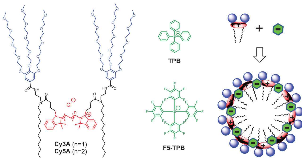
Figure 2.3.1. Amphiphilic dyes synthesized in this study and their assembly in the presence of non-coordinating anions into micellar NPs
