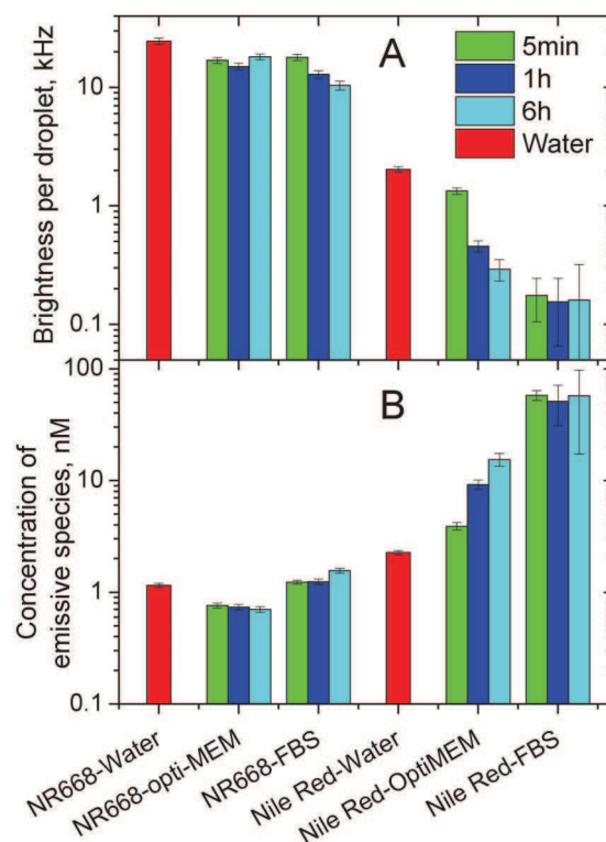
Fig. 6 Dye release studies by FCS. (A) Brightness and apparent concentration (B) of emissive species in water and in biological media determined from FCS data. Brightness is the photon count rate per droplet. The nano-emulsions prepared in water were measured 5 min after dilution in the indicated media at room temperature or after incubation in these media at 37 °C for 1 h or 6 h. Data in water, measured 5 min after dilution at room temperature, are presented for comparison.
