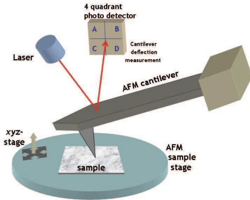
Figure 1.36 AFM operation combined with a use of an optical lever.
