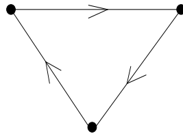
Figure 4.2: Graphe cyclique
