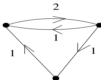
Figure 4.1: Graphe orient  G.
