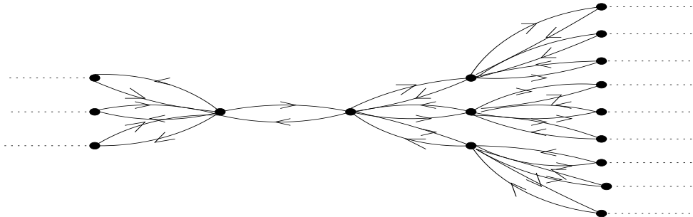
Figure 3.1: Arbre digraphe 8-régulier
