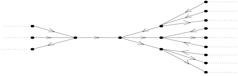
Figure 3.2: Arbre 4-régulier
