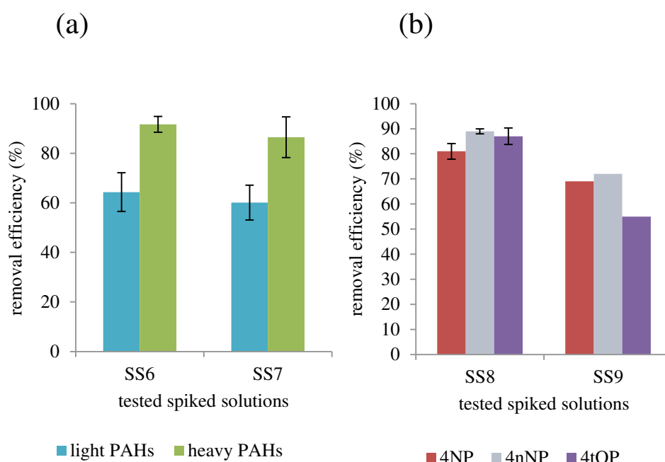
Figure 7: Removal efficiency (%) after treatment by activated polyBTCA-CD (dose = 2 g L -1 ) for (a) two concentrations of PAHs: low for SS6 and high for SS7 (n=3) and (b) two concentrations of APs: low for SS8 (n = 3) and high for SS9 (n = 1).
