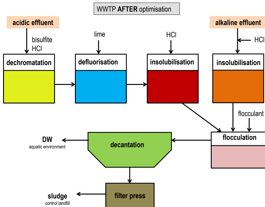
Figure 1: Physico-chemical treatment plant used by Silac Industry for the removal of pollutants from effluent, before and after modification
