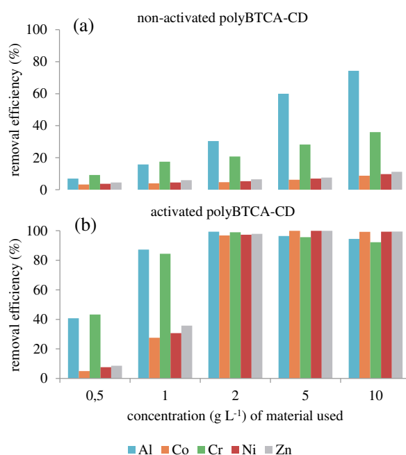
Figure 5: Adsorption capacity (%) of (a) the non-activated and (b) the activated (NaHCO 3 treatment) polyBTCA-CD at different doses for 5 metals (at 10 mg L -1 ).
