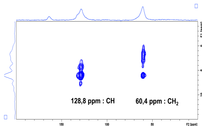
Figure 78. Spectre HETCOR du PET brut.
