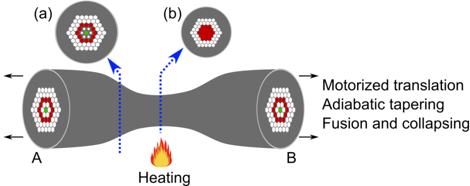
Figure III-16: Operation principle of the manufacturing of the mode converter.
