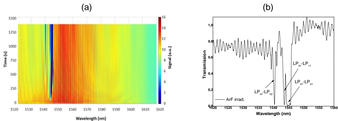
Figure III-7: (a) Evolution of FBG transmission according to time in the 1.5 \mu\text{m} -FMF. (b) FBG transmission spectrum at t = 1690 s
