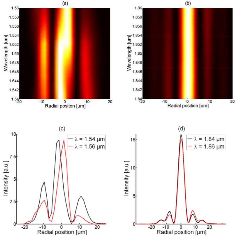
Figure III-19: Radial scan of the output near field of the mode converter excited by (a) the Erbiun ASE source with 41 points of measurements and (b) the Thulium ASE source with 101 points of measurements. (c) and (d) are the respective radial traces at the beginning and the end of both bandwidths.
