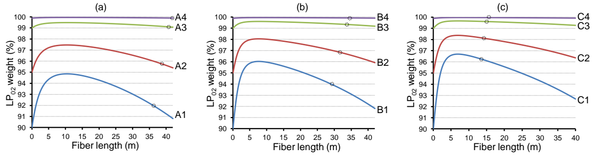
Figure IV-12: LP_{02} weight evolution along amplification in the Enhanced design few-mode fiber in (a) case A, (b) case B and (c) case C. Black dotted circles are the respective L_{opt} where the amount of power in the LP_{02} mode is the highest.
