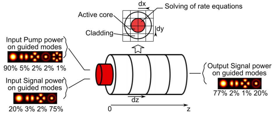
Figure IV-7: Modeling of a core-pumped multimode amplifier. The input powers of the pump and signal are split among the guided modes at the respective wavelengths. The output data give the new modal weights (and therefore modal power) at each wavelength.
