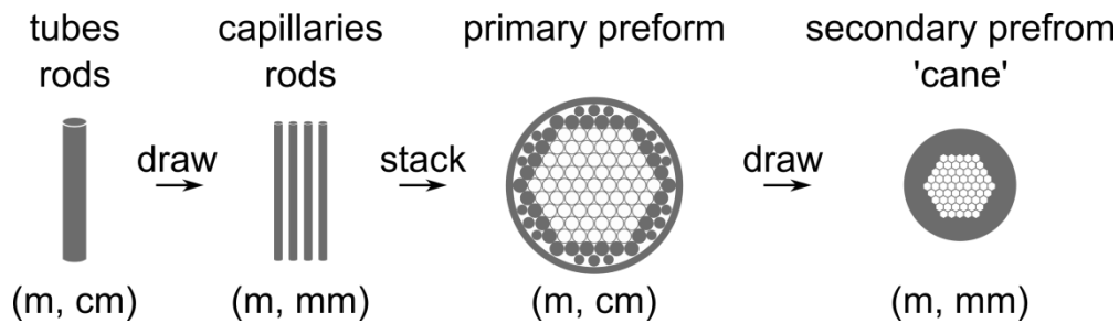
Figure III-15: Fabrication of a holey preform (or cane).
