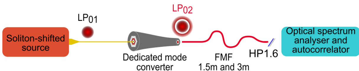
Figure III-27: Dispersion measurement setup using the SFSS source centered at 1.95 \mu\text{m} , the dedicated mode converter and the passive few mode fiber
