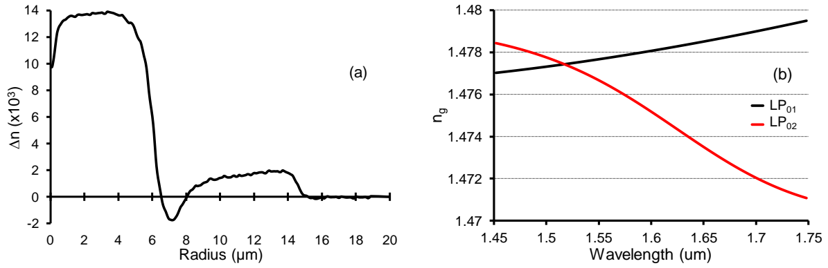
Figure III-6: (a) Measured refractive index difference of the 1.5 \mu\text{m} -FMF and (b) Calculated group index of the \text{LP}_{01} (black) and \text{LP}_{02} (red) modes.
