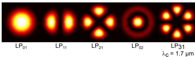
Figure IV-6: Guided LP modes of the few-mode TDF at \lambda = 1.56 \mu m .
