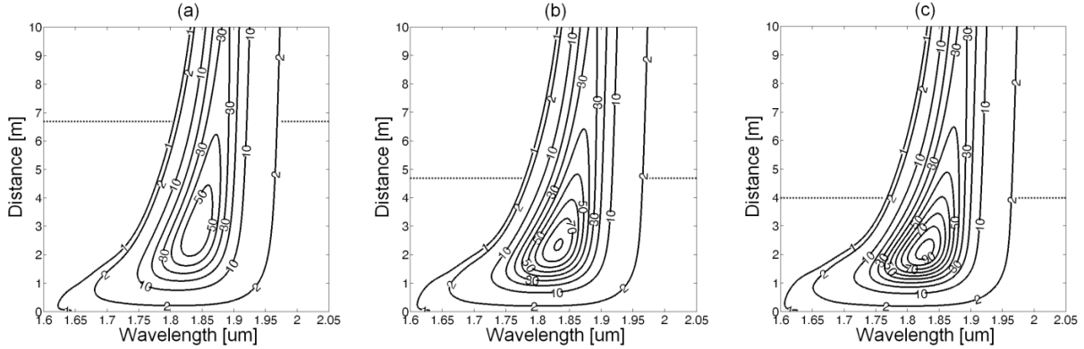
Figure IV-8: Results from modeling of LP 02 cw TDFA. Spectral and spatial evolution of the gain for (a) \lambda_p = 1.535 \mu\text{m} , (b) 1.55 \mu\text{m} , (c) 1.56 \mu\text{m} . Optimal lengths for maximal output power are (a) 6.66 m, (b) 4.75 m, (c) 3.97 m, shown by dotted lines.
