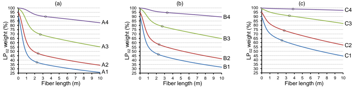
Figure IV-10: LP_{02} weight evolution along amplification in (a) case A, (b) case B and (c) case C. Black dotted circles are the respective L_{opt} where the amount of power in the LP_{02} mode is the highest.
