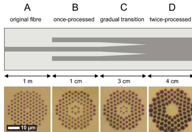
Figure III-11: Top, Schematic longitudinal cross section of the inflation-based mode converter, showing core areas in dark gray. Bottom: optical micrographs of the holey region in the cleaved fiber in each of sections A–D, on the same scale. From [32].
