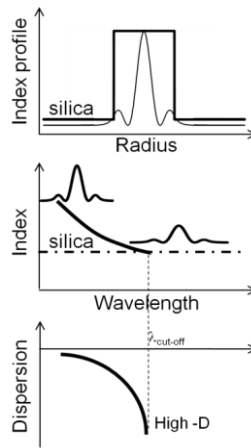
Figure II-1: Principle of operation of a moderately multimode fiber for dispersion control. Top: Generic profile of a step-index moderately multimode fiber. Associated LP_{02} intensity profile. Middle: LP_{02} mode effective index versus wavelength. Insets show the field spreading when \lambda increases. Bottom: LP_{02} dispersion versus wavelength.
