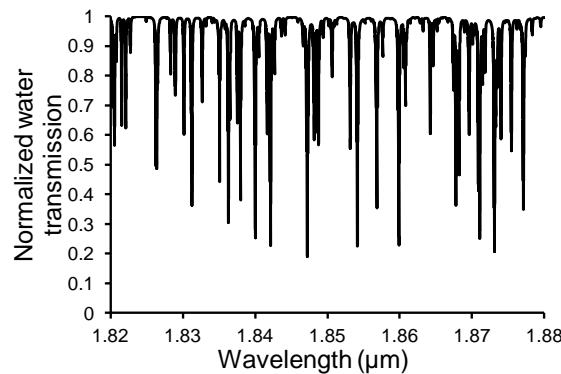
Figure A-IV-36: Water transmission from 1.82 \mu\text{m} to 1.88 \mu\text{m} in a 1 m gaz cell with 25% humidity ( http://spectralcalc.com/ ).
