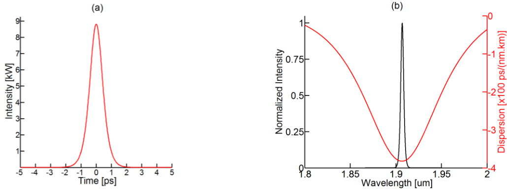
Figure IV-14: Numerical simulations of the input (a) temporal ( \Delta t = 1 ps) and (b-black) spectral profile ( \Delta\lambda = 4 nm) of the pulse carrying 10 nJ of energy seeding the core-doped optimal few-mode fiber with constant gain (1.9 Np/m), assuming constant effective area of 353 \mu\text{m}^2 and wavelength dependent dispersion (b-red).
