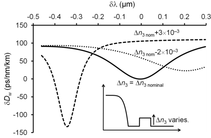
Figure II-7: Impact of the ring index difference \Delta n_3 on the dispersion spectrum.
