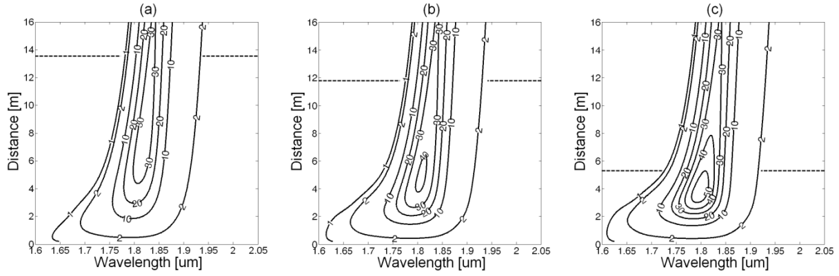
Figure IV-13: Results from modeling of LP 02 cw TDFA in the enhanced few-mode fiber design. Spectral and spatial evolution of the gain for case (a) A4 (b) B4 (c) C4. Optimal lengths for maximal output power are shown by dotted lines.
