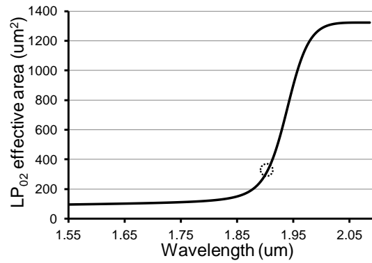
Figure IV-22: Calculated LP_{02} effective area according to wavelength in the optimal fiber. Dotted circle is A_{eff}^{02}(\lambda_{Dmax}) = 353 \mu m^2 .
