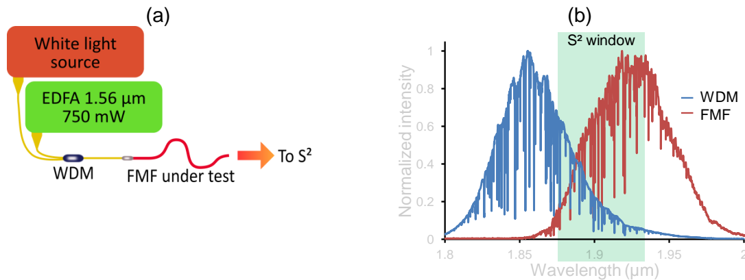
Figure A-IV-40: (a) S^2 setup for an active fiber. WDM: Wavelength division multiplexer. (b) Spectrum at the output of the WDM (blue) and of the active FMF (red). The S^2 measurement window is marked by the green surface.
