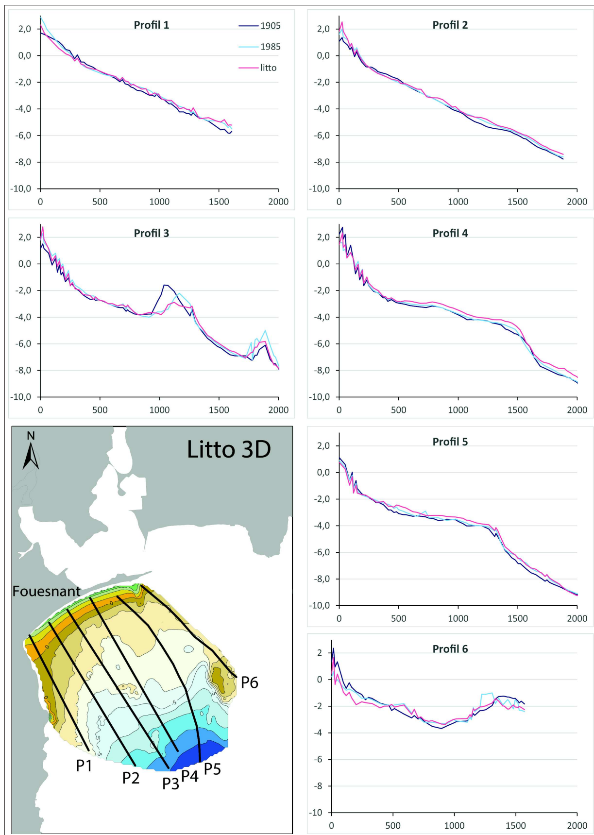
FIGURE 2.28 – Zone 2 : Profiles
