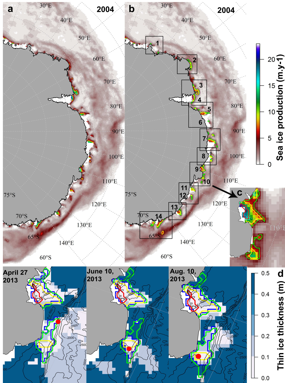
Figure V.2: Illustration of the polynya definition based on SIP and thin ice thickness. Example of yearly SIP ( \text{m}\cdot\text{y}^{-1} ) map obtained from the sum of monthly SIP during the freezing period from March to October in 2004 (a). Same as (a) with boxes superimposed defining some polynya areas based on literature, within which polynya definition polygons were computed based on threshold of SIP of 2.5 \text{m}\cdot\text{y}^{-1} (green contour), 5 \text{m}\cdot\text{y}^{-1} (yellow contour) and 10 \text{m}\cdot\text{y}^{-1} (red contour) (b). A total of 14 polynyas were identified: 1. Lützoh-Holm Bay, 2. Cape Borle, 3. Cape Darnely, 4. Mackenzie, 5. Barrier, 6. West Ice Shelf, 7. Shackleton, 8. Bowman Island, 9. Vincennes Bay, 10. Cape Poinsett, 11. Dalton, 12. Paulding Bay, 13. Dibble, 14. Mertz. The insert is a zoom of polynyas 9 and 10 to highlight the different contours (c). Examples of map of thin ice thickness data for three days in 2013 where SIP polynya definition (i.e. 2.5 \text{m}\cdot\text{y}^{-1} (green contour), 5 \text{m}\cdot\text{y}^{-1} (yellow contour) and 10 \text{m}\cdot\text{y}^{-1} (red contour)) and bottom topography are superimposed (d). Within the green polygon (i.e. the larger polynya definition based on SIP), polygons of thin ice were daily drawn for thickness comprised between 0 and 0.2 m (blue contour). The red dot corresponds of one the seal position for this given day.
