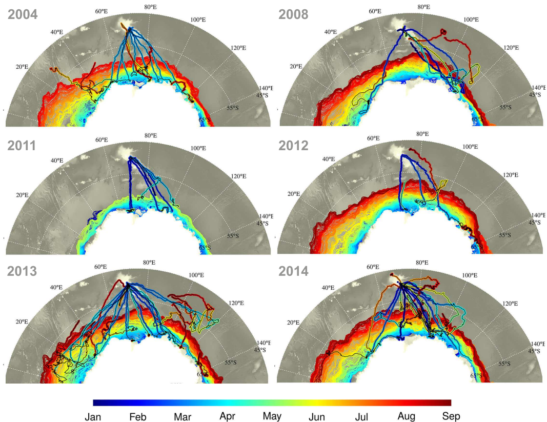
Figure III.3: Tracks of the 46 post-moulted individuals equipped with CTD-SRDs from 2004 to 2014, linked with the seasonality of the sea ice in the East Antarctic region. The colour scale represents the time and the same colour is used for sea ice extent and tracks of animals; the sea ice extent of a given day and associated seal positions are colored in the same way. For visual purposes, tracks and sea ice extent were limited to September (annual maximum sea ice extent) and the unique individual in 2009 was removed. For all years, sea ice extent was obtained from SSMI/S daily sea ice concentration (resolution 25 km).
