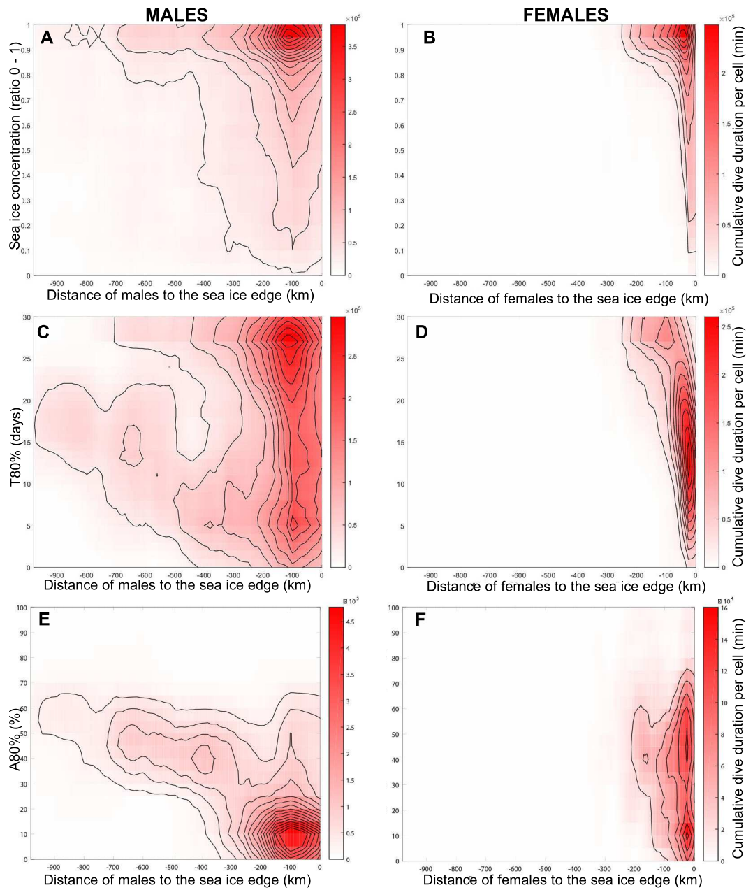
Figure III.6: Density plot of the distance of males and females to the sea ice edge relative to: A, B) Sea ice concentration; C, D) The temporal variability of concentrated sea ice patches ( T_{80\%} , expressed as the number of days with sea ice concentration above 80% at a given location within a 30 day window); and E, F) The spatial variability of concentrated sea ice patches ( A_{80\%} , expressed by the area covered by sea ice with concentration above 80% within a 50 km radius around the animal). The colour scale represents the sum of dive duration (in minutes) per grid cell (note that a sliding window has been applied for smoothing purposes). Distances on the x-axis represent when seals are inside the sea ice zone, with values increasing towards the ice edge (at 0 km). One contour is drawn every 0.25 \cdot 10^5 min.
