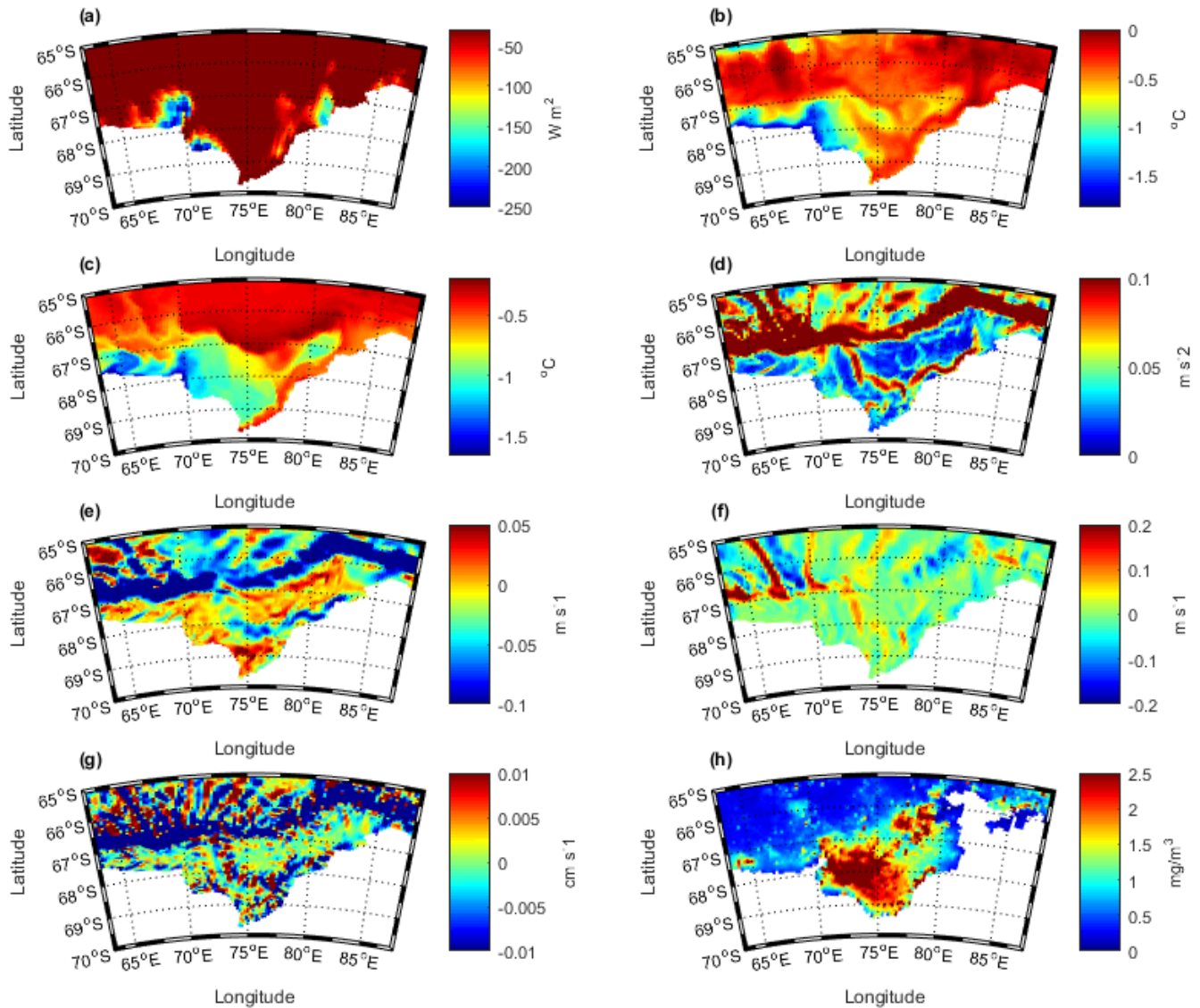
434 Fig 6. Physical and biological predictors fields used to build the seasonal GAMM for PM1.
