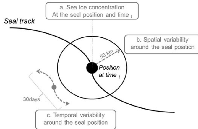
Figure III.1: Schema illustrating the three sea ice variables used in the study: (a) the sea ice concentration at the position of the seal at the present time, (b) the area covered by sea ice with a concentration of > 80\% within a 50 km radius around the animal ( A_{80\%} ) and (c) the number of days with a sea ice concentration of > 80\% at a given location within a 30 day window ( T_{80\%} ).
