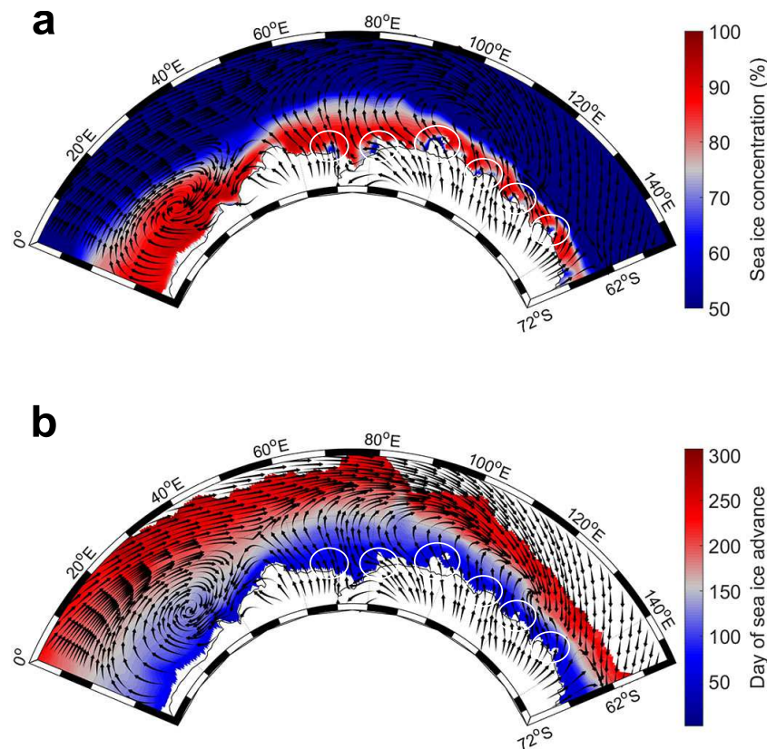
Figure IV.2: Climatological patterns of sea ice and near-surface winds from 2004 to 2014. (a) Mean sea ice concentration (expressed as percentage) and monthly-averaged ERA-Interim 10 m winds zonal and meridional component are shown for the winter season (June-August). (b) Mean day of sea ice advance and monthly-averaged ERA-Interim 10 m winds zonal and meridional component from March to June. Ellipses represent coastal polynya sites, from left to right: Cape Darnley/Mackenzie, Barrier, Shackleton, Vincennes Bay, Dalton, and Dibble. For illustration purposes, autumn-averaged sea ice concentration (March-May) is not represented. Maps were made using MATLAB software (version 8.5.0.197613 (R2015a), URL http://fr.mathworks.com/ ).
