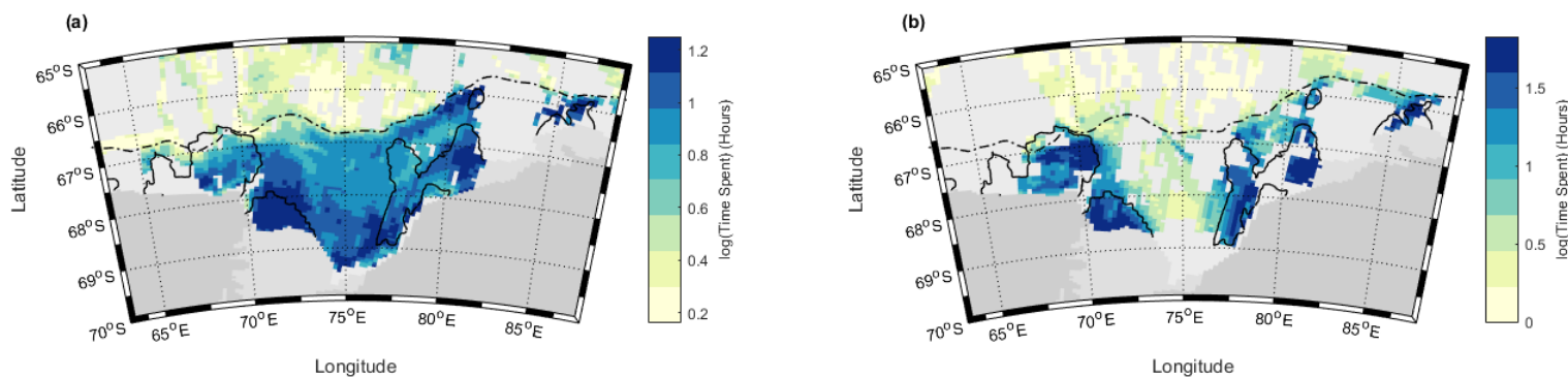
472 Fig 7. Generalised additive mixed model predictions of SES habitat selection.
