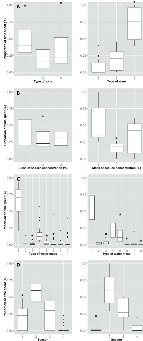
Figure II.5: Boxplots representing the proportion of time spent in each type of environment for the 28 post-moulting animals equipped with CTD-SRDs from 2004 to 2013 and including tracks from 55°S to the Antarctic continent. Statistics are presented separately for males (left panels) and females (right panels). Part A indicates the time spent in different type of zone, (1) the Antarctic shelf, (2) the continental slope, (3) the pelagic area. Part B indicates the time spent in different type of sea ice concentration, (1) from 0% to 5%, (2) from 5% to 80%, (3) from 80% to 100%. Part C indicates the time spent in different water masses (1) AASW, (2) AAIW, (3) CDW, (4) MCDW, (5) HSMCDW, (6) MSW, (7) AABW, (8) HSSW, (9) ISW. Part D indicates the time spent in different seasons (1) Summer, (2) Autumn, (3) Winter, (4) Spring. Significant differences of time spent in each type of environment between males and females are indicated by a star.
