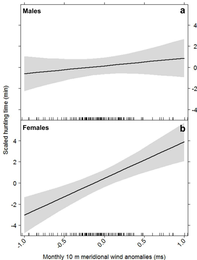
Figure IV.5: Relationships between foraging activity and meridional near-surface wind anomalies for (a) males and (b) females. Linear mixed effect models (LMMs) were used to quantify the links between foraging activity of males and females and monthly ERA-Interim 10 m meridional wind anomalies within the sea ice zone, from March to August for females and March to October for males. For each graph, the thick lines represent the predictive values from the population and the grey shaded envelopes represent the boundaries of the variation between the predicted values per individual.
