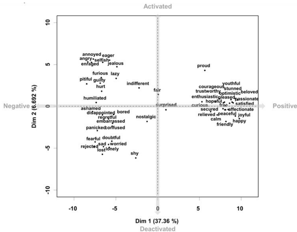
Figure 1.3 Representation of the emotions issued from MFA
