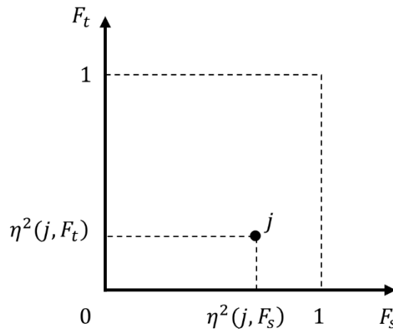
Figure A-1 Illustration of categorical variable on the plane constituted by vectors F_s and F_t by using the correlation ratio.
