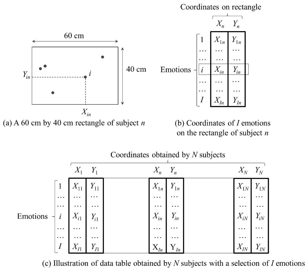
Figure 2.4 Illustration of data table obtained by the Napping® method
