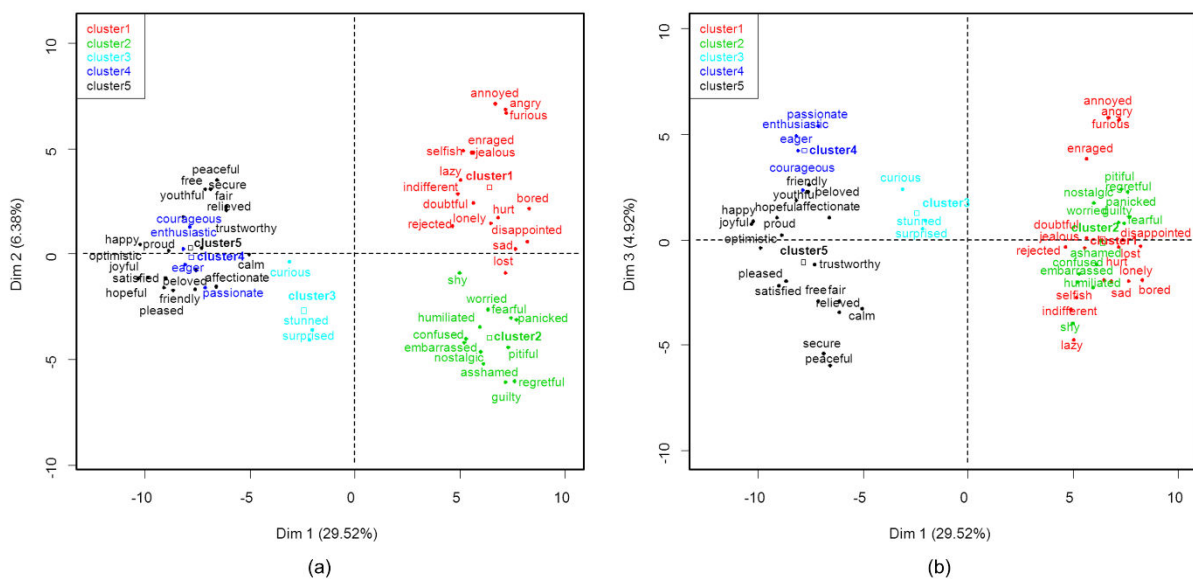
Figure 2.9 The typology of 5 clusters was illustrated on the factorial planes obtained by MFA: (a) the first-two dimensional plane, and (b) the first-three dimensional plane.
