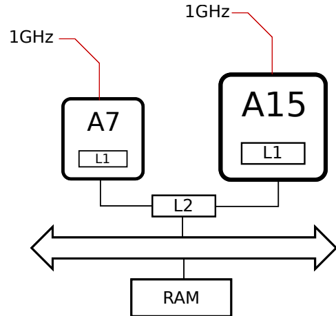
Figure 1.13: A simplified big.LITTLE architecture
