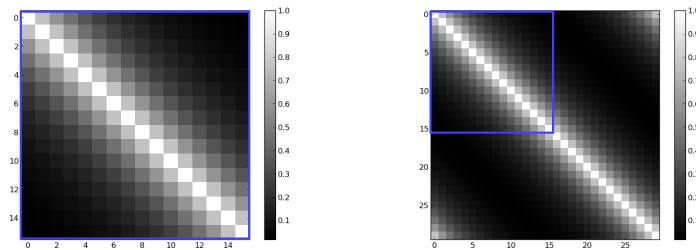
Figure 5.1: Circulant embedding (right) of a symmetric 1D Toeplitz matrix (left), namely a Gaussian kernel matrix evaluated on a 1D grid of 16 points. The Toeplitz matrix (blue frame) is embedded in the upper left corner of the circulant matrix (right).
