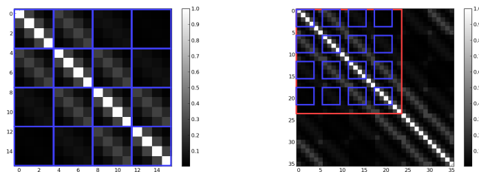
Figure 5.2: Circulant embedding (right) of a symmetric 2D Toeplitz matrix (left), namely a Gaussian kernel matrix evaluated on a 1D grid of 4-by-4 points. The small Toeplitz matrices (blue frames) are embedded in the upper left corner of the small circulant matrices (right), while blocks are also embedded in the upper left corner (red frame) of a circulant block structure (right).
