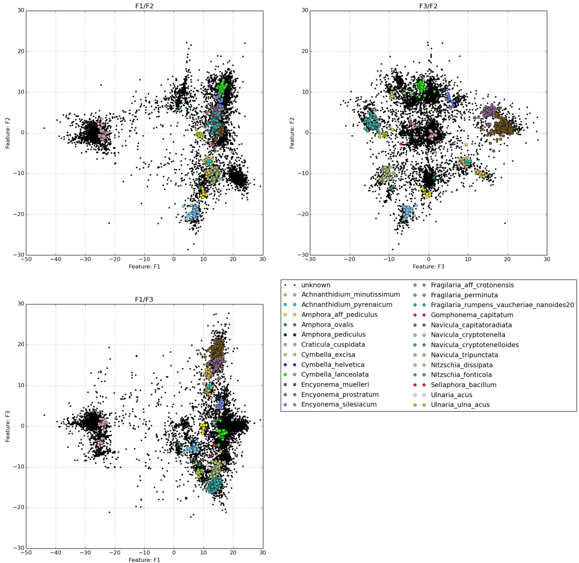
Figure 8.7: Representation of the point cloud associated to 10.000 random reads of the sample L_6 on the first 3 features F1 , F2 , F3 using 2D plots. The components were computed using rSVD with s = r = 200 . Identified species are represented using large colored markers, while unknown species are represented in black. Observation: Such representation allows for easily verifying that individuals of the same identified species gather in clusters. However random subsampling does not allow to represent all individuals and in particular all the previously identified ones.
