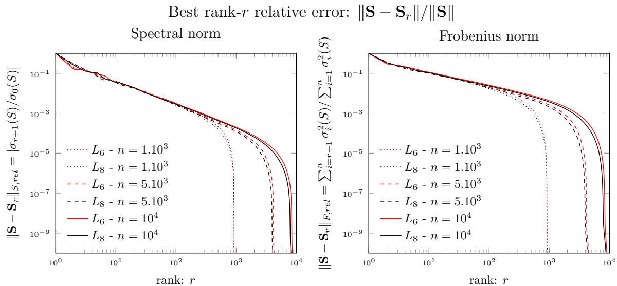
Figure 8.1: Best rank- r error w.r.t. the rank in term of Frobenius (right) and Spectral (left) norm for a subset of a full sample from Lake Geneva at various times. \mathbf{S}_r is obtained by mean of a full SVD, therefore we can only afford to compute small subsamples, namely up to n = 10^4 .
