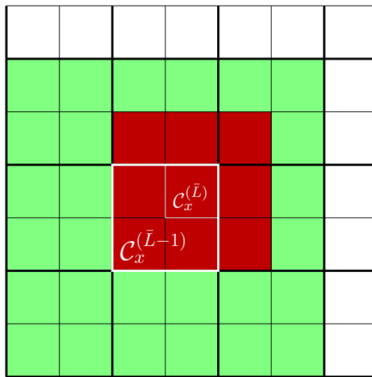
Figure 1.2: The portion of a quadtree at level \bar{L} and \bar{L} - 1 used to precompute the M2L operators. The interaction list \mathcal{I}(c_{\mathbf{x}}^{(L)}) (green) and neighbor list \mathcal{N}(c_{\mathbf{x}}^{(L)}) (red) of a target particle \mathbf{x} are represented at the leaf level for \gamma = 2 .
