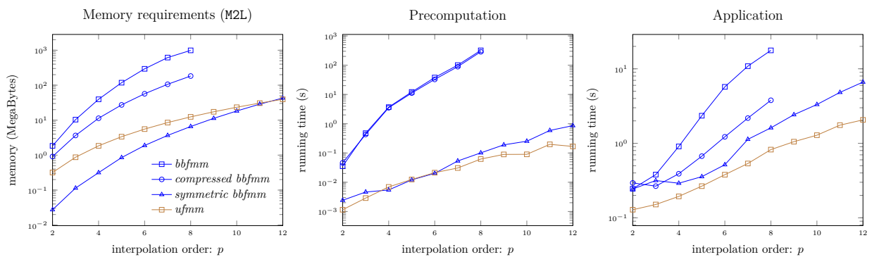
Figure 5.10: Experimental memory requirements and computational time of the ufmm and variants of the bbfmm w.r.t. the interpolation order p . We use the homogeneous Laplacian kernel k(r) = 1/r on a uniform distribution of 20.000 particles inside the unit cube with \bar{L} = 3 . The computation is done on simple desktop computer.
