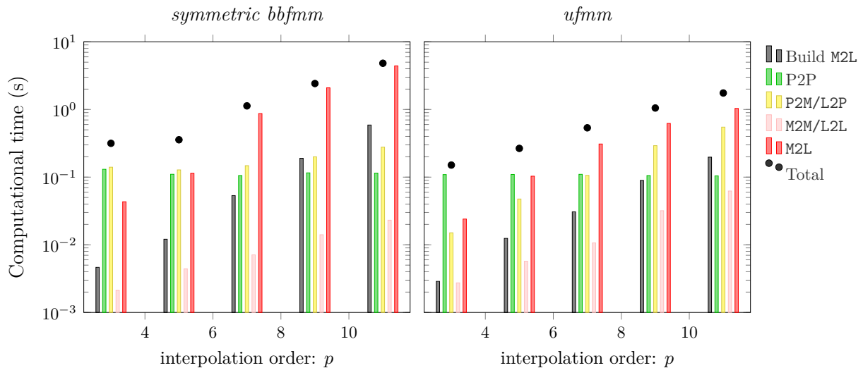
Figure 5.11: Detailed computational time for the symmetric-bbfmtm (left) or the ufmm (right) w.r.t. the interpolation order p . We used n = 20,000 particles distributed uniformly in the unit cube with \bar{L} = 3 .
