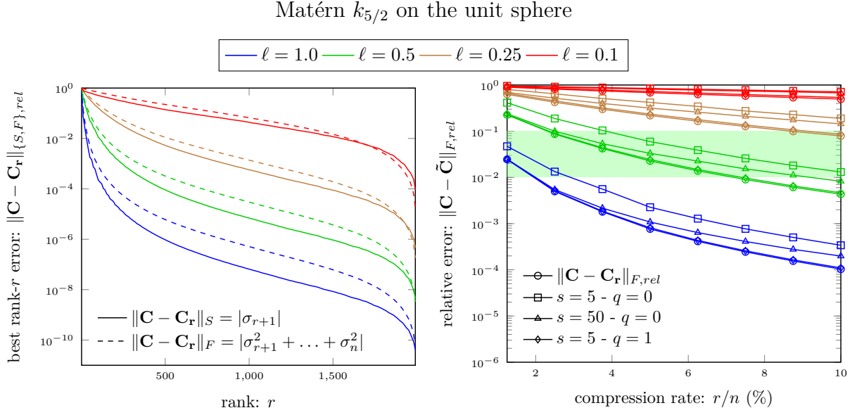
Figure 7.6: Accuracy of the fixed rank r SVD w.r.t. the compression rate for a Matérn \nu = 2.5 correlation and n = 2,000 particles distributed on the unit sphere. Left: Optimal relative error in Spectral and Frobenius norms w.r.t. to r = 1, \dots, n . Right: Accuracy of the r SVD w.r.t. prescribed rank r = 20, \dots, 200 . Observations: The correlation is smoother than the exponential, therefore its spectrum decreases faster. On one hand, it seems insufficient to increase the oversampling by a constant value, namely s = 5 or s = 50 . On the other hand, one power iteration leads to a near-optimal error but the optimal error remains relatively high. In fact, a 1% relative error is not reachable for \ell < 0.5 for a maximum compression rate of 10%.
