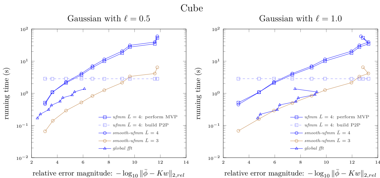
Figure C.1: Running time of a multi- rhs FMM w.r.t. the relative error magnitude using various algorithms: ufmm and smooth-ufmm with p = 2 \dots 11 , and global fft with p = 6 \dots 14 . We used 72.000 particles randomly distributed in a cube. Observations: ufmm and smooth-ufmm have approximately the same cost when they share the same tree depth. The smooth-ufmm is significantly faster if we choose an optimal tree depth, e.g., \bar{L} = 3 represented in solid brown lines. If the Gaussian decreases sufficiently slow, i.e., the rank is sufficiently low, then the cost of the global fft is similar to the optimal smooth-ufmm . However, the global fft exhibits an instability for the highest interpolation order.
