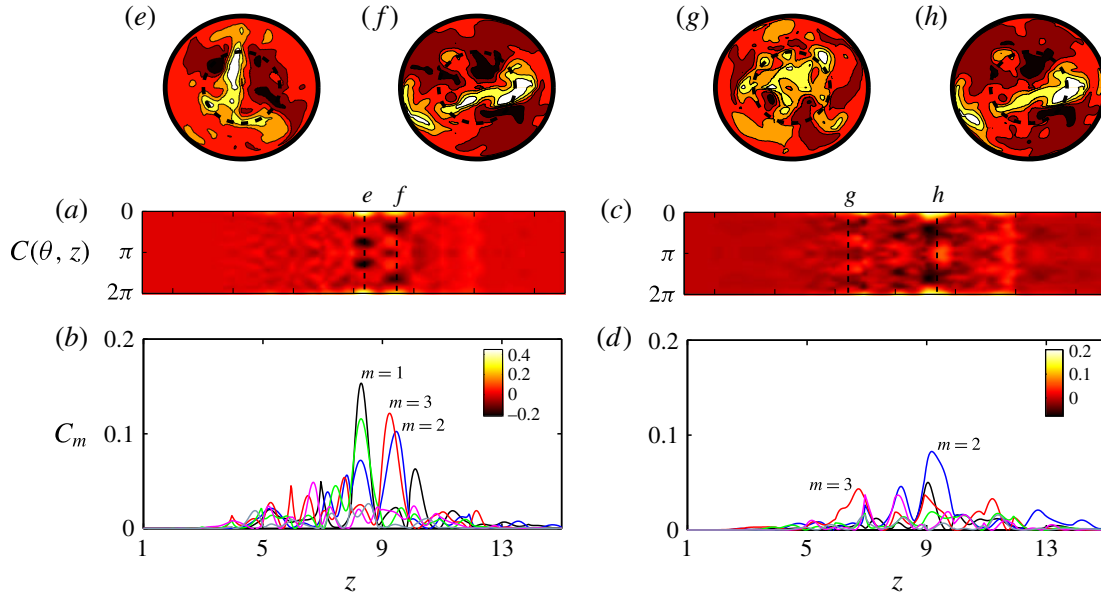
FIGURE 8. Spacial correlation on the streamwise velocity of localised turbulence at Re = 2000 . Contour of correlation, C(\theta, z) , at (a) r = 0.5d and (c) r = 0.8d . Projection function of C(\theta, z) for different azimuthal wavenumbers m at (b) r = 0.5d and (d) r = 0.8d . (e–h) Cross-sections of the axial flow relative to the time averaged profile with fast flow (white) and slow flow (red) taken at the corresponding vertical dashed lines.
