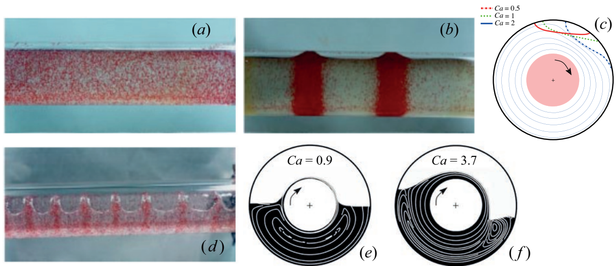
Figure 3.6: (a, b and d) Particle segregation in monodisperse sheared suspensions in a horizontal cell, images from experiments from Tirumkudulu et al. 46 . (a) Initial state: well mixed 10% suspension (red) at 95% fill level before shearing, (b) final state: after shearing at 9 rpm and (d) final state: 15% suspension at 50% fill level sheared at 6 rpm. (c, e and f) Fluid flow simulations of the partially filled cell using the mean field method showing flow cross-section and the interface deformation: (c) 90% fill level at Ca = 0.5, 1 and 2 (e) 50% fill level at Ca = 0.9 and (f) 3.7 . Note the cusp formation.
