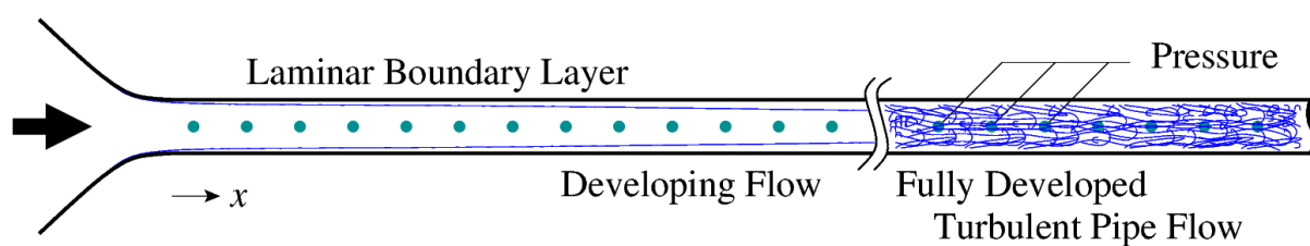
Figure 2.11: Schematic of the developing pipe flow transition. The flow is from left to right, the dots indicate the position of pressure taps and the blue line in the developing region represent the developing boundary layer.
