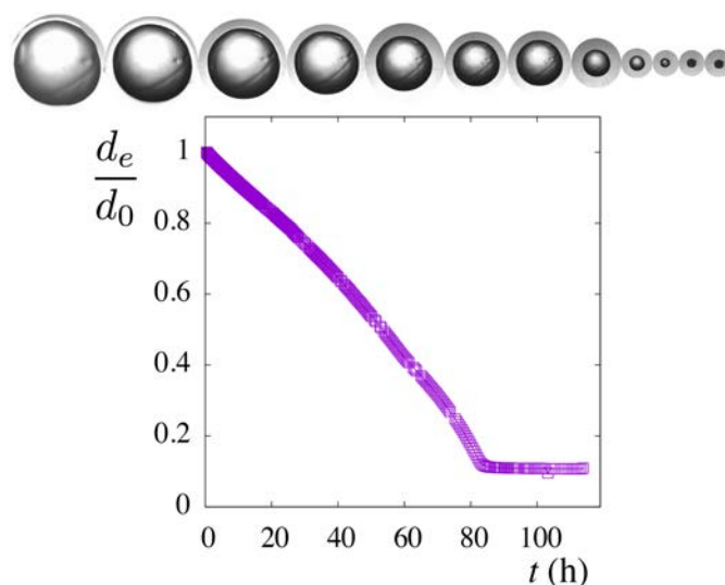
Figure 4.8: Time evolution of the diameter of the spherical gel during drying. Here d_0 is the fully swelled or wet diameter. At t = 0 , the swollen (wet) sphere is taken out of water and put on a watch glass. A sequence of images showing the drying of the polymer over the course of 120 hours. The whole experiment is conducted at T = 22 \pm 1^\circ\text{C} .
