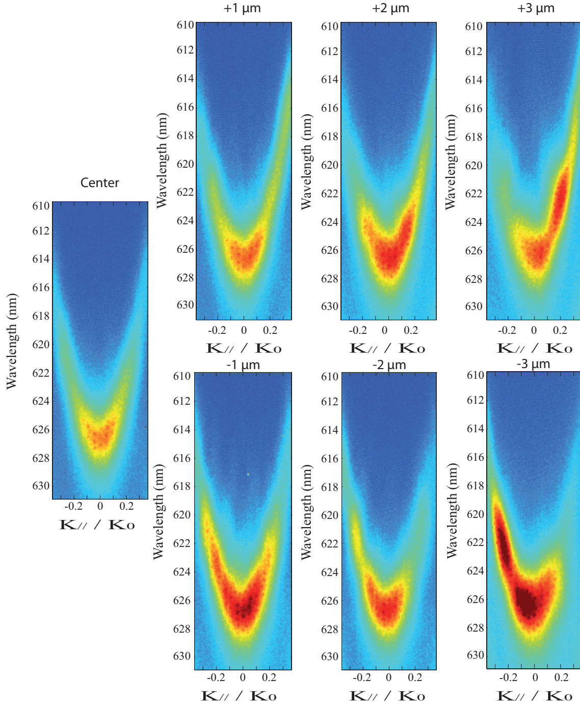
Figure 2.31: Measured emission pattern from a 10 \mu\text{m} disk with respect to the laser excitation position
