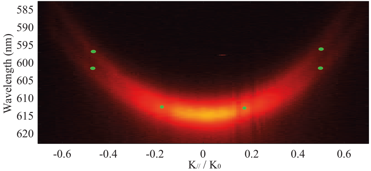
Figure 2.16: Photoluminescence from the 2D-Tamm sample analyzed as a function of wavelength and emission angle \sin \theta = k_{\parallel}/k_0 . The green dots indicate the 2D-Tamm dispersion relation obtained from the reflection spectra.
