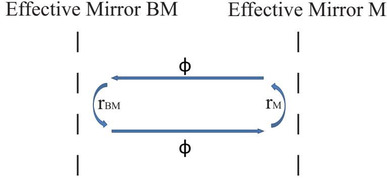
Figure 2.3: Effective mirror description for the optical Tamm structure: r_{BM} is the reflectivity of the Bragg mirror, r_M is the reflectivity of the metallic surface and \Phi is the phase introduced by the light propagation between these two effective mirrors.
