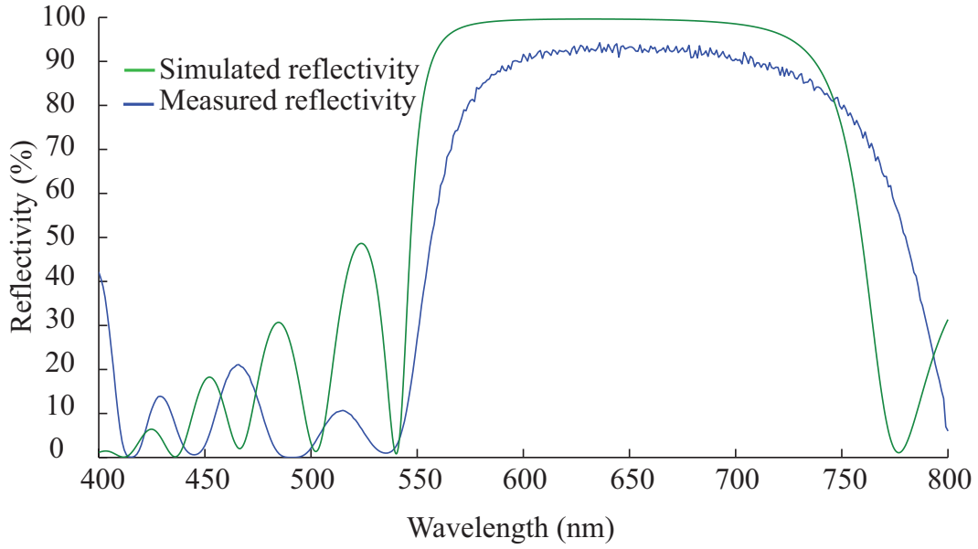
Figure 2.11: Simulated and measured reflection spectra of the fabricated Bragg Mirror.
