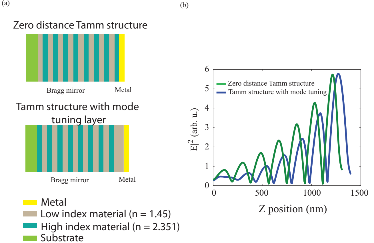
Figure 2.6: (a) Schematic of two different Tamm structures. Top: a Tamm structure with zero dephasing \Phi . Bottom: the Tamm structure studied in this PhD: a layer of dielectric is added between the Bragg mirror and the metal layer to tune the resonance wavelength. (b) Electric field intensity |E|^2 distribution of the corresponding Tamm state along the z -axis of the structure (7 pairs of quarter wave TiO_2 and /SiO_2 on Si substrate and 45 nm of silver on top).
