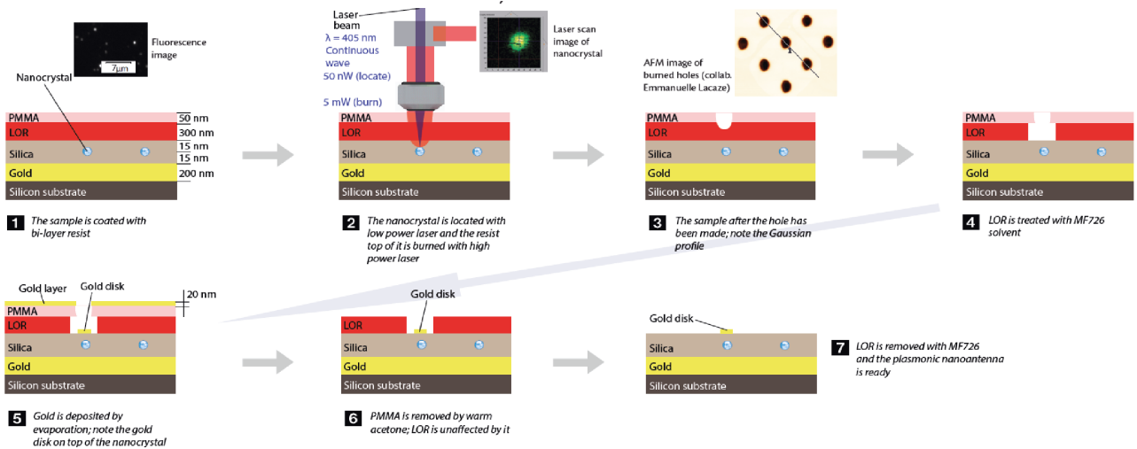
Figure 2.26: Schematic presentation of in situ lithography technique for colloidal nanocrystal at visible range (technique developed during the thesis of Cherif Belacel and Amit Raj Dhawan) [26]
