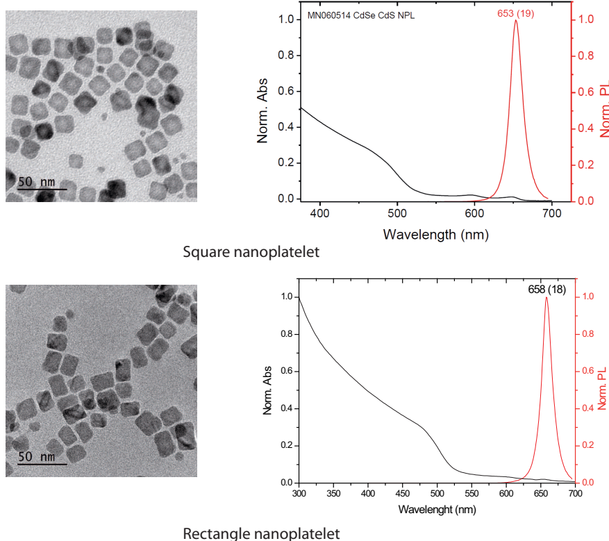
Figure 3.7: TEM image, absorption and emission spectra (in solution) of the square and rectangle nanoplatelets excited by a UV lamp. (Figure from Benoit Dubertret, ESPCI)
