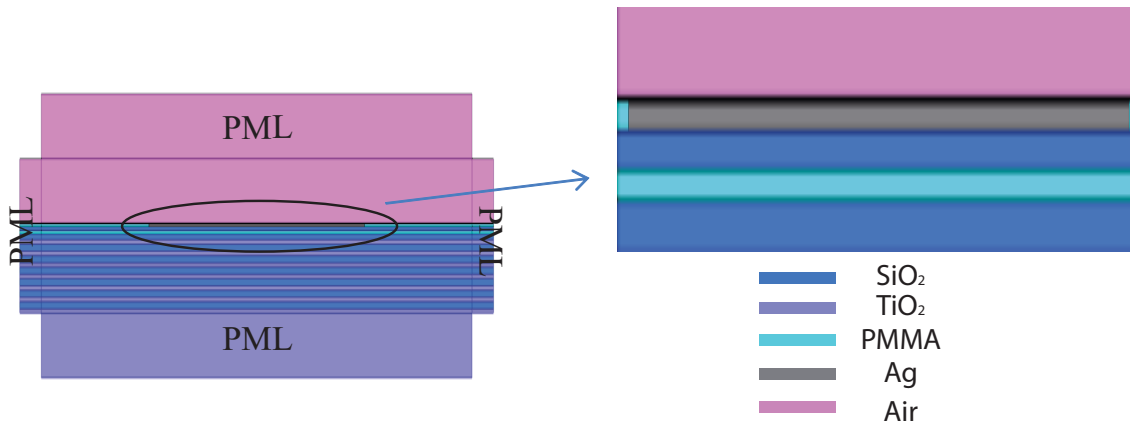
Figure 2.19: Schematic representation of the simulated structure
