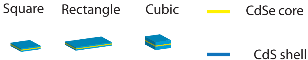
Figure 3.6: Schema of the structure of a nanoplatelet
