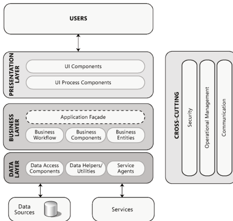
Figure 2.3 – Common layers in a software architecture 1
