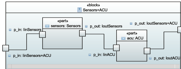
Figure 8.10 – IBD for the second iteration
