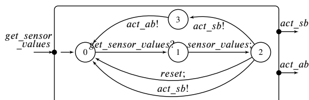
Figure 8.8 – IA for the composition of Sensors and ACU blocks
