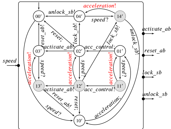
Figure 6.12 – Product A_1 \otimes A_2 between the automata Sensors and ACU
