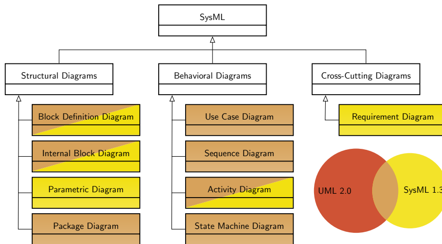
Figure 3.1 – Relation between UML and SysML
