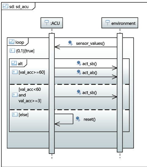
Figure 7.4 – SD for the ACU block
