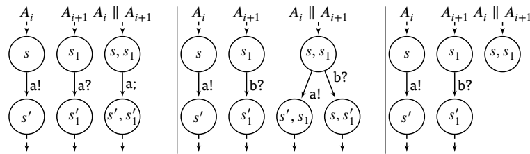
Figure 8.5 – Interface automata composition alternatives
