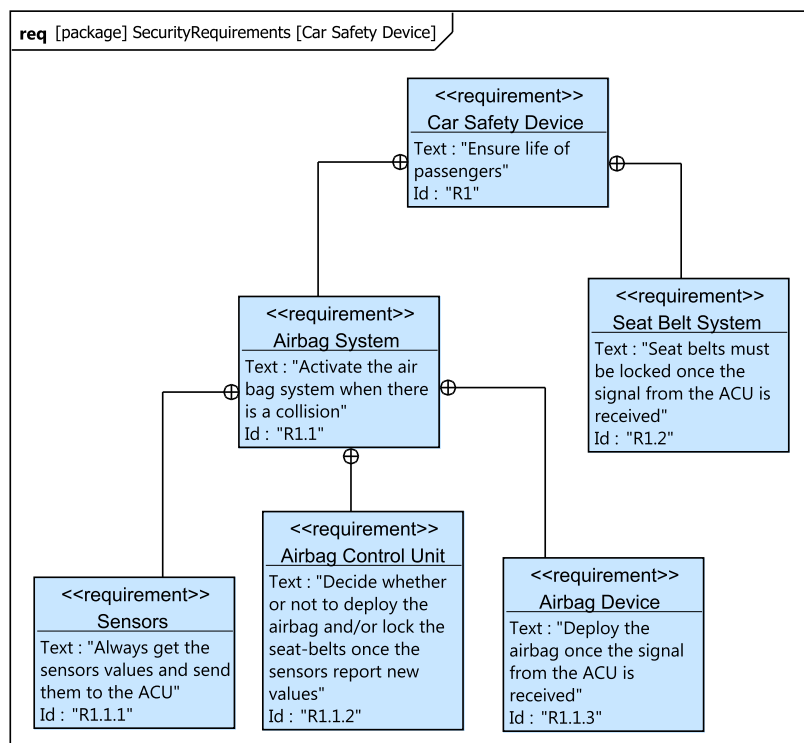
Figure 3.5 – A requirement diagram
