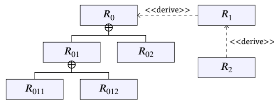
Figure 8.4 – A SysML requirement diagram
