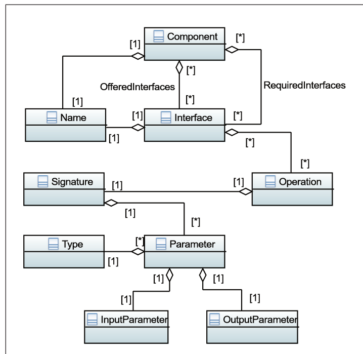
Figure 2.2 – UML metamodel for the specification syntax of a component
