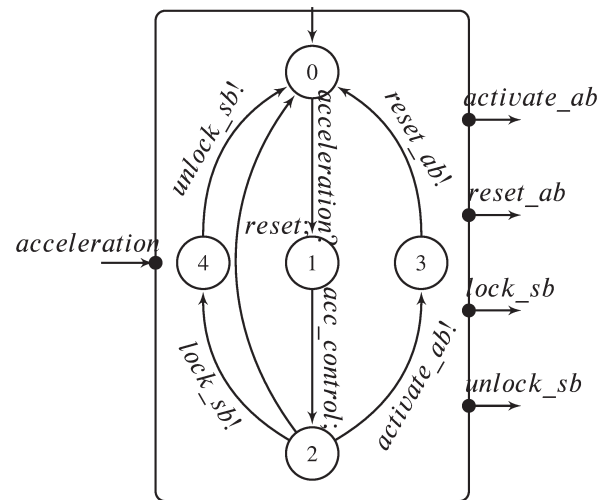
Figure 6.11 – Interface automaton A_2 associated to the ACU
