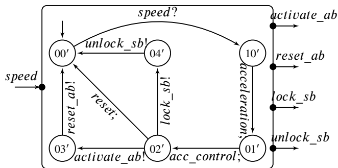
Figure 6.13 – Composition A_1 \parallel A_2 between the automata Sensors and ACU
