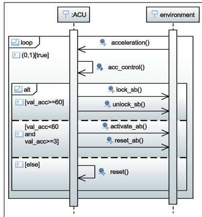
Figure 6.10 – ACU sequence diagram
