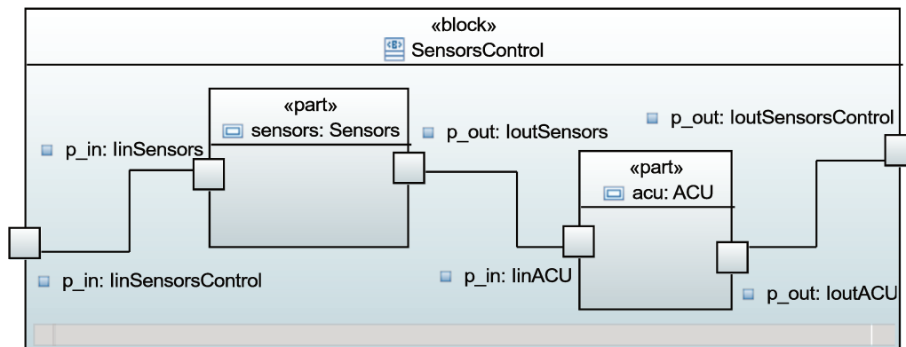
Figure 3.3 – An internal block diagram
