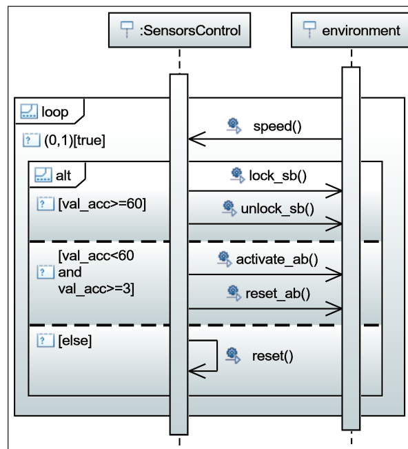
Figure 3.4 – A sequence diagram
