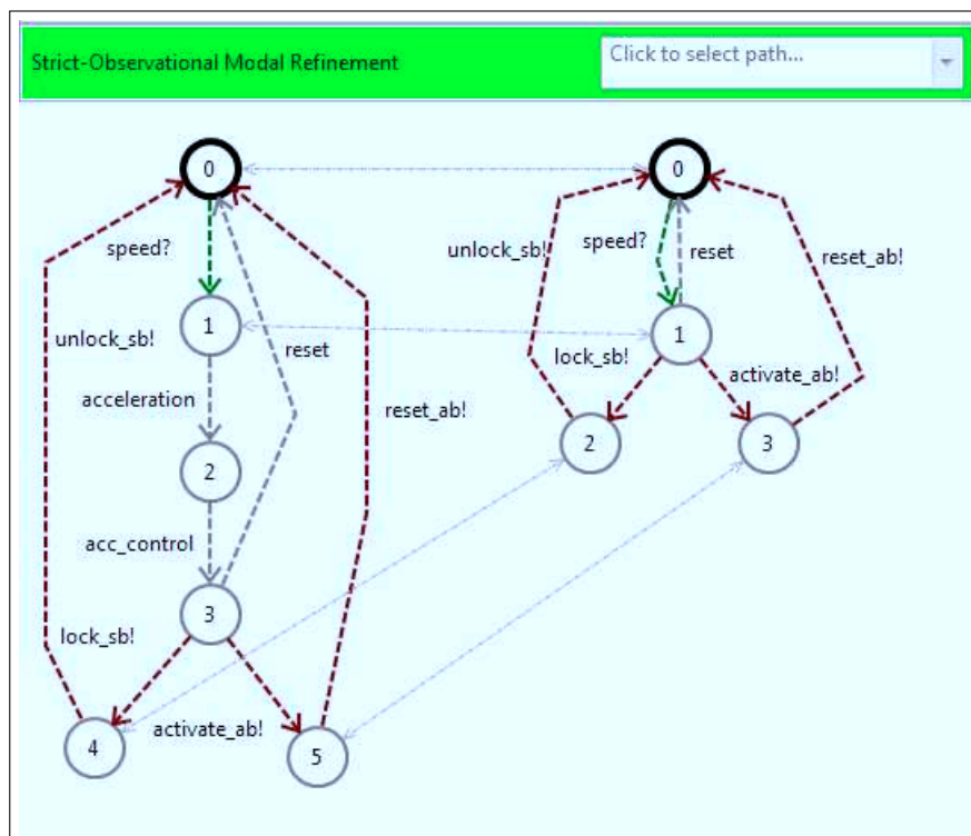
Figure 6.16 – Refinement in MIO Workbench
