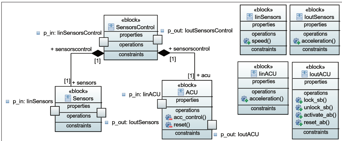
Figure 3.2 – A block definition diagram
