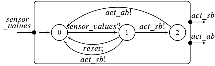
Figure 4.2 – Interface automaton B for the ACU block
