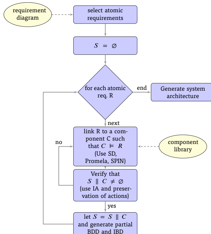
Figure 8.2 – Proposed approach to generate CBS architecture from SysML requirements
