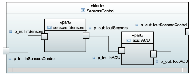
Figure 6.7 – Internal block diagram of the SensorsControl block
