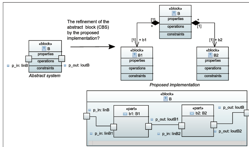
Figure 6.2 – Proposed approach for verifying structure and behavior refinement in SysML
