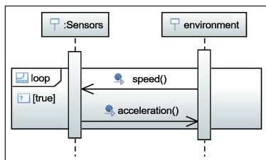
Figure 7.2 – SD for Sensors block
