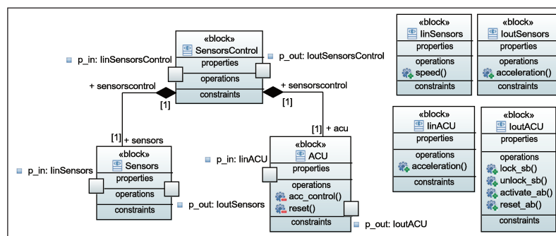
Figure 6.6 – Proposed block definition diagram for SensorsControl block
