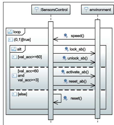
Figure 6.14 – SD for SensorsControl abstract block
