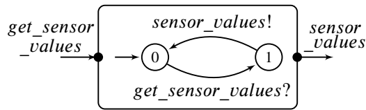
Figure 4.1 – Interface automaton A for the sensor block
