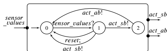
Figure 8.7 – IA for the ACU block
