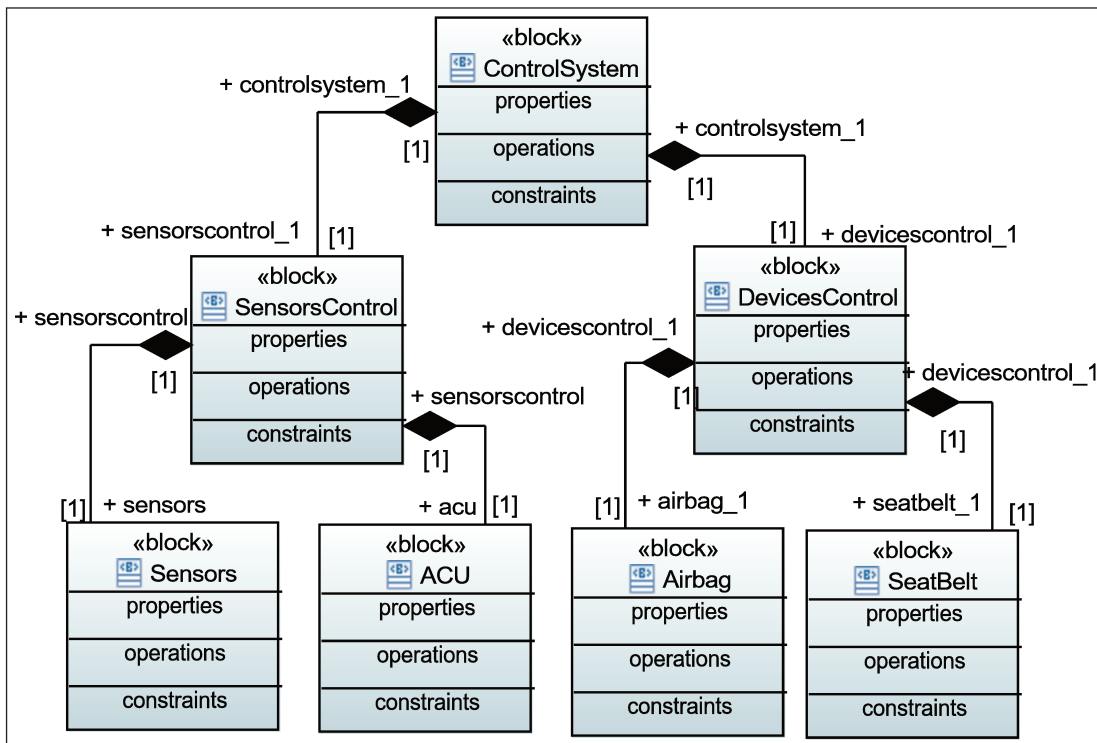
Figure 6.17 – The final BDD of the safety vehicle system
