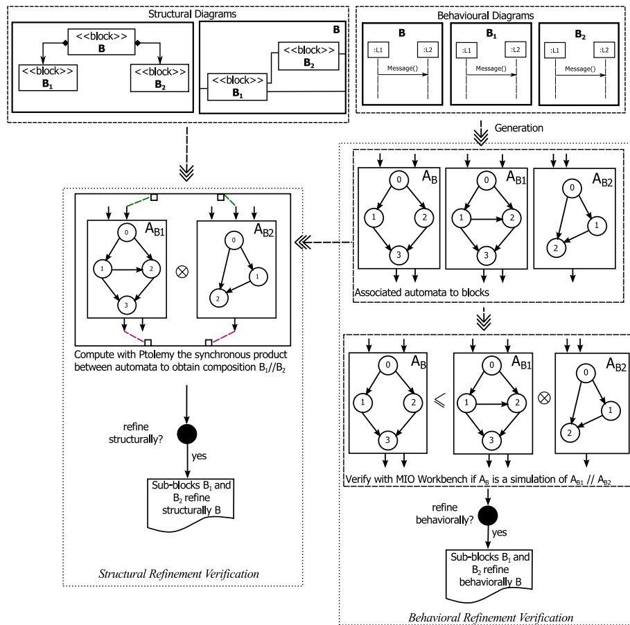
Figure 6.3 – Structural and behavioral refinement verification in a SysML Block Decomposition
