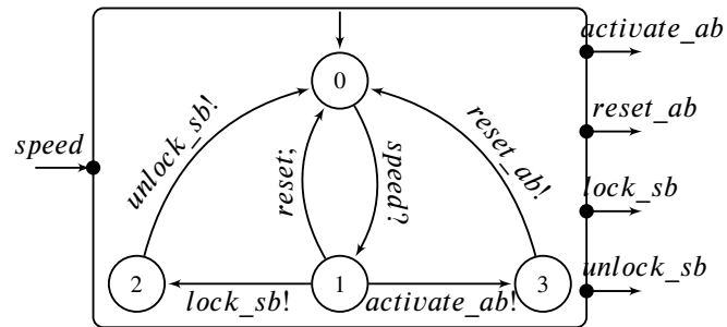
Figure 6.15 – IA associated to the SensorsControl abstract block
