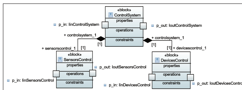
Figure 6.4 – The preliminary BDD of the safety vehicle system
