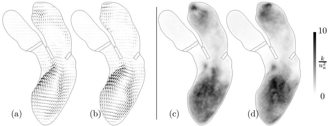
Figure 5.14: Velocity (left plots) and TKE maps (right plots) obtained with the dynamic Smagorinsky and with the \sigma -model. For each plots couple, the left is the results of simulation with dynamic Smagorinsky model, the right with \sigma -model. The displayed maps correspond to t/T_a = 0.65 .
