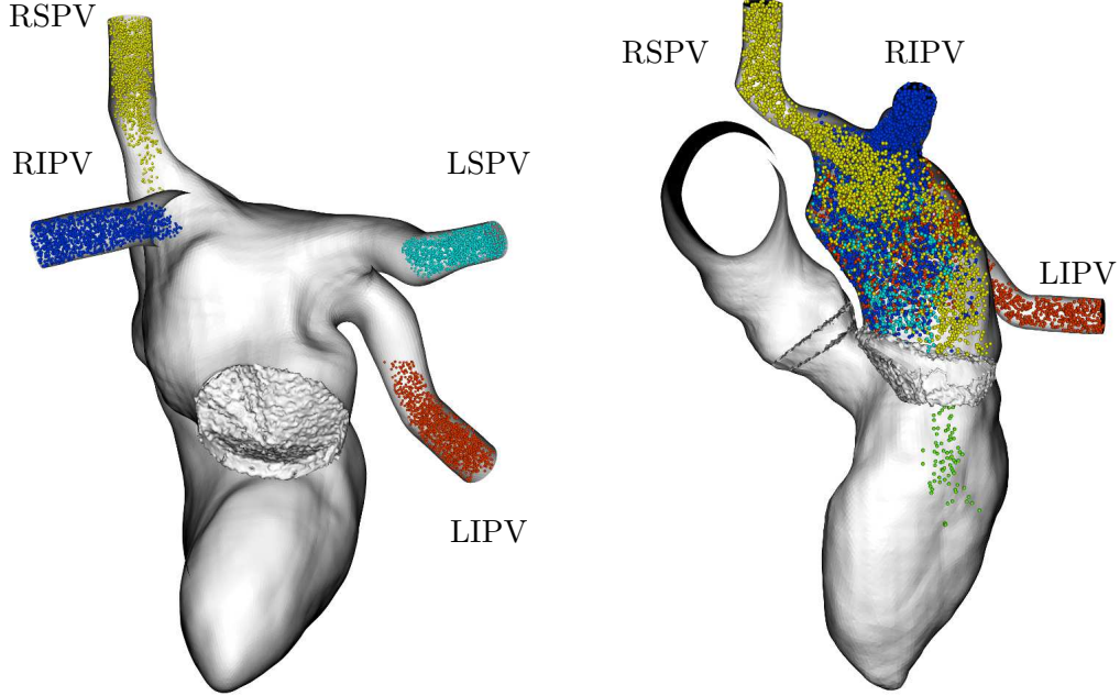
Figure 8.1: Scheme of heart A . The names of the four pulmonary veins are indicated. Statistics are saved first when the particles pass through the mitral valve (coloured in green in the right figure to indicate that they are accounted for in statistics) and then when the particles pass through the aortic valve.
