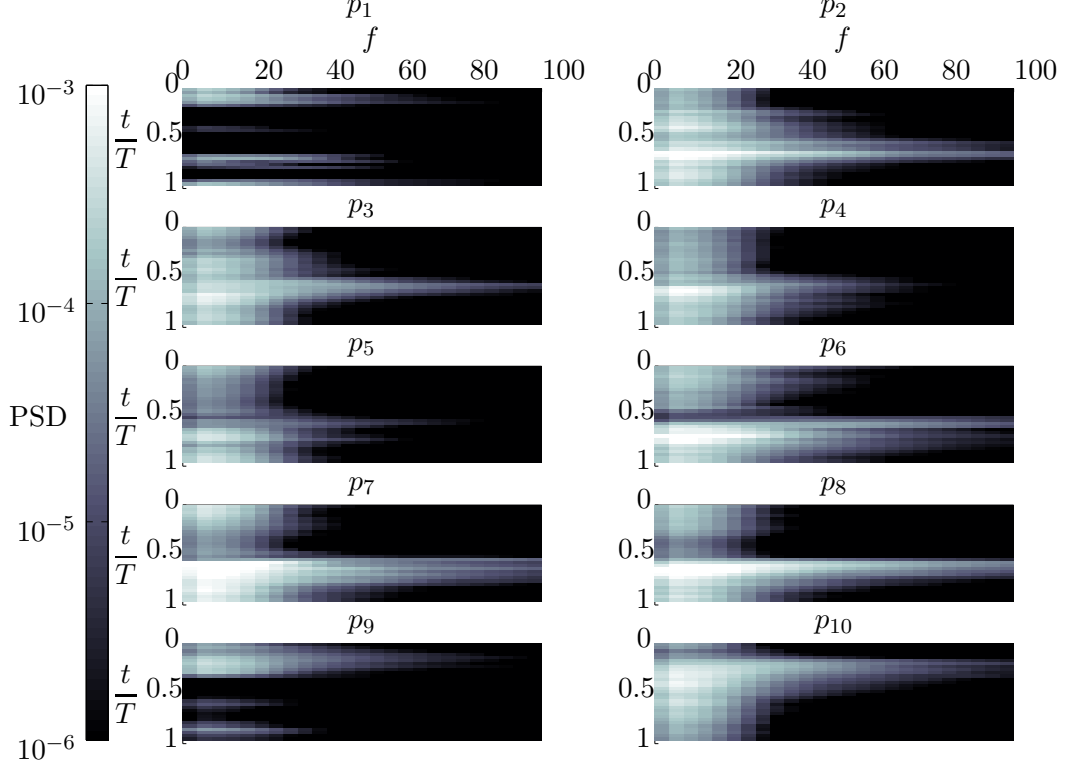
Figure 6.19: Time-frequency representation of the Power Spectral Density (PSD) of the vertical fluctuating velocity u_3 at the 10 probes locations. PSD is color coded (scale on the left) with the same range as Fig. 6.18.
