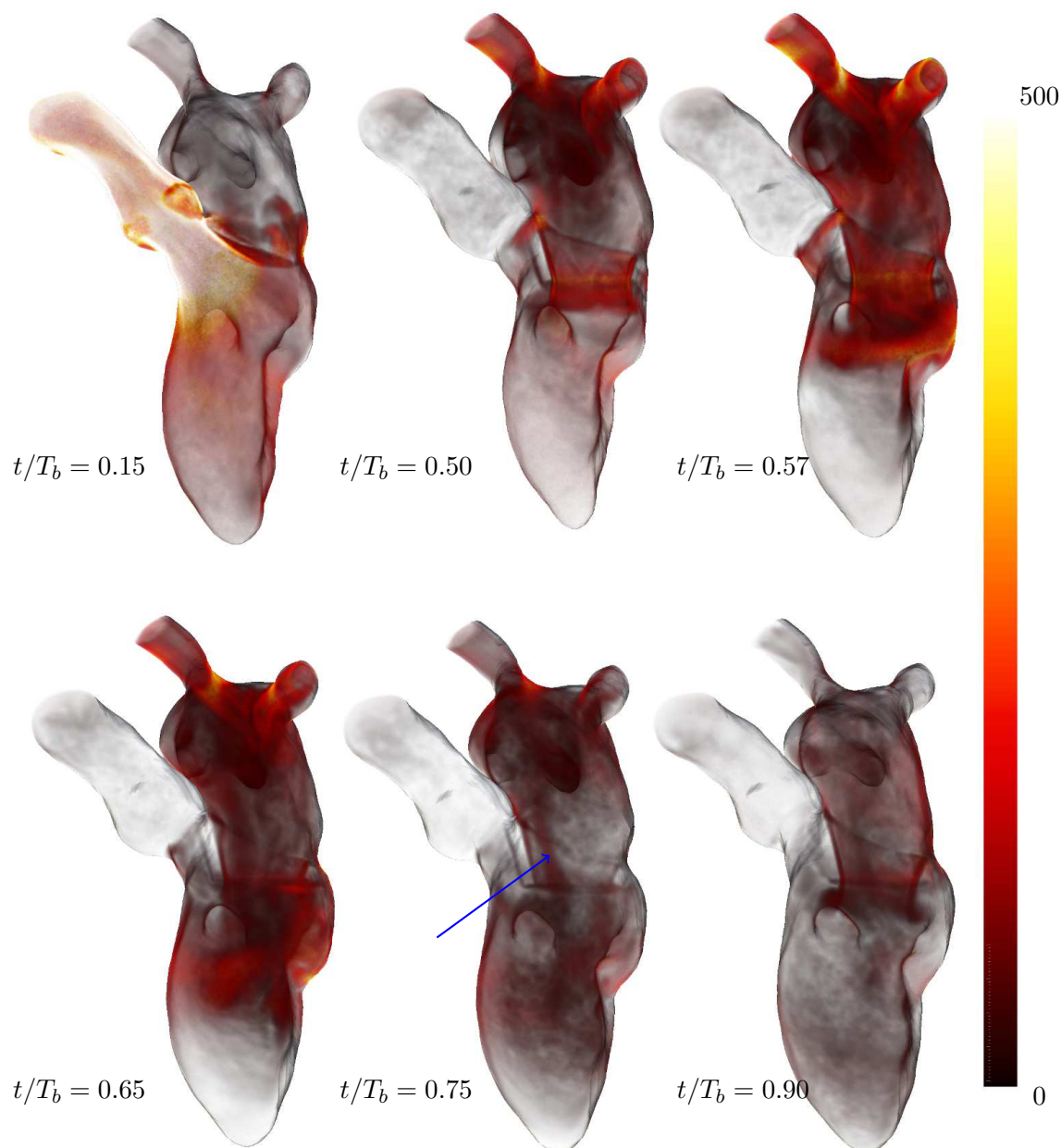
Figure 7.7: Volume rendering of non-dimensional vorticity magnitude of the phase-averaged velocity fields at different times of the simulation. First row, left plot: t/T_b=0.15 . Center plot: t/T_b=0.50 . Right plot: t/T_b=0.57 . Second row, left plot: t/T_b=0.65 . Center plot: t/T_b=0.75 . Right plot: t/T_b=0.90 . The mapping relating vorticity magnitude with opacity is linear. The heart wall is made partially transparent to allow a better observation of the flow behaviour.
