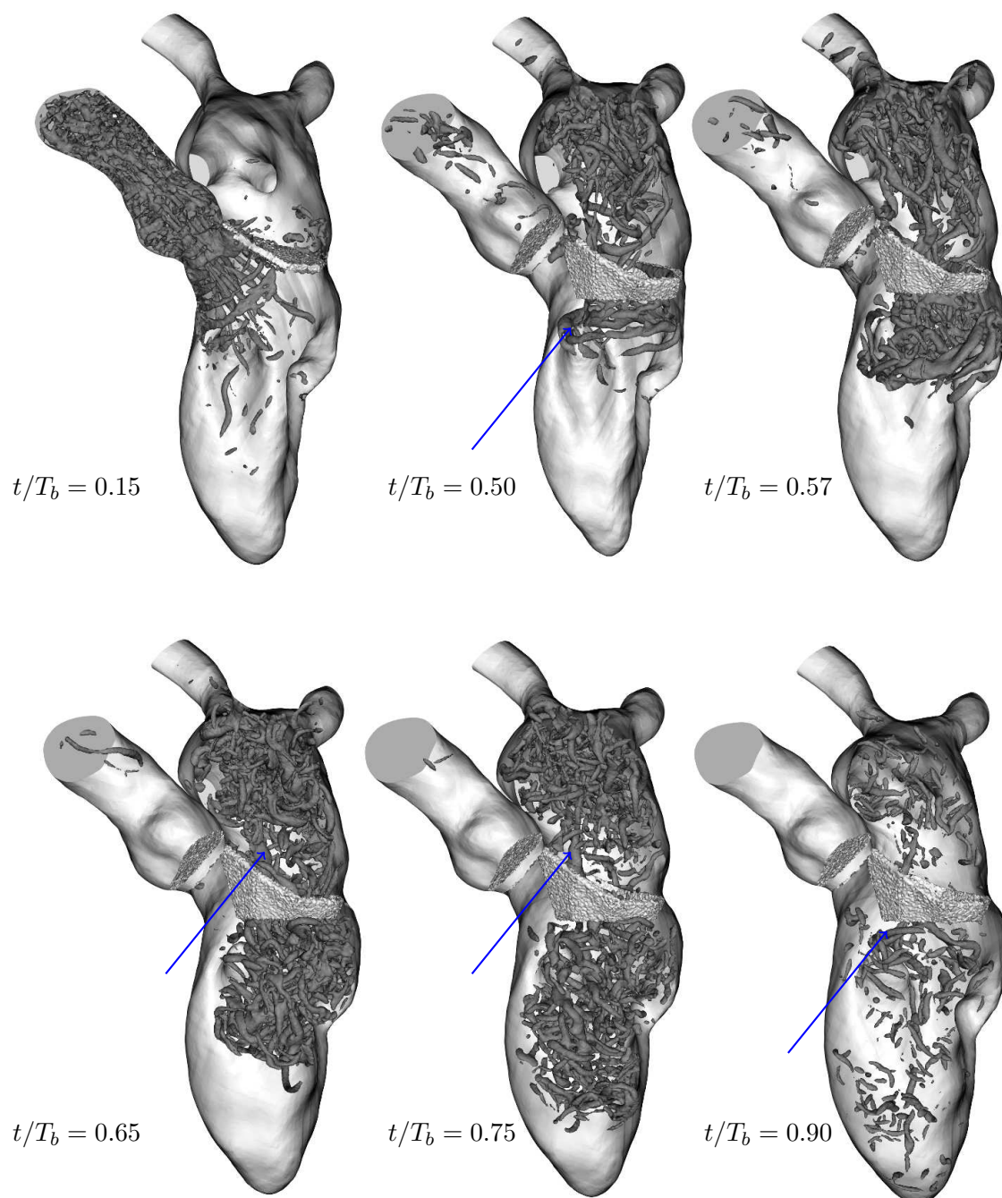
Figure 7.8: Evolution of Q criterion isosurface ( Q = 70u_b^2/R_a^2 ) showing the vortical structures present in a typical instantaneous velocity field.
