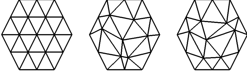
Figure 3.3: Visualization of the mesh deformation. From left to right, mesh at t = 0 , t = \tau/3 , t = 2\tau/3
