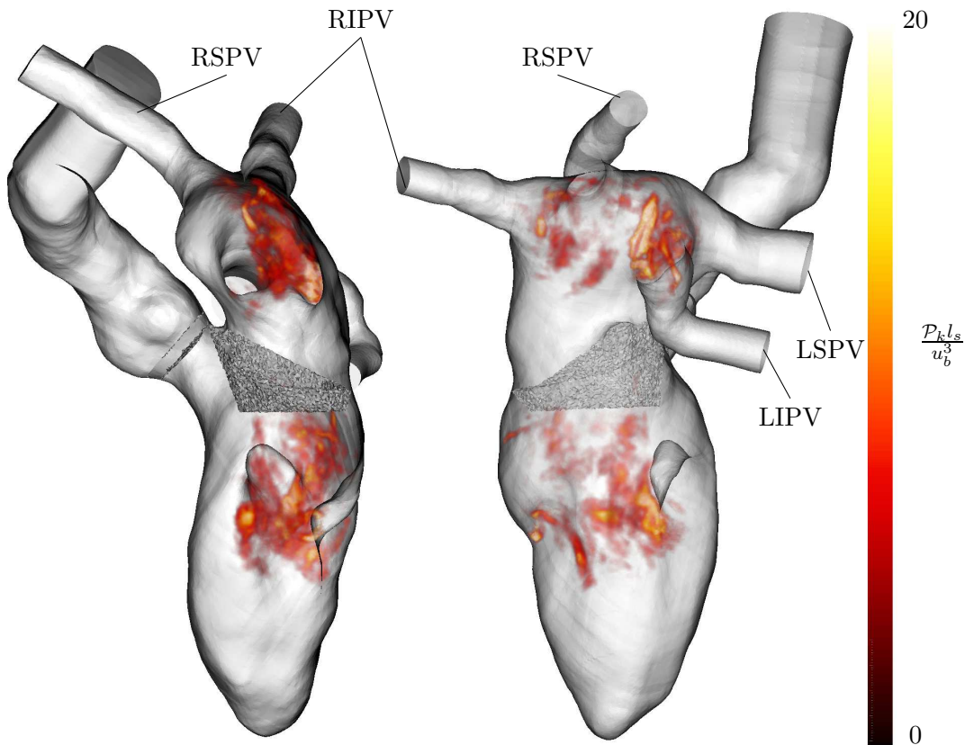
Figure 7.17: Volume rendering of the production of turbulent kinetic energy \mathcal{P}_k non-dimensionalised by u_b^3/l_s at t/T_b = 0.65 . The mapping relating production magnitude with opacity is linear. Heart wall is made partially transparent to allow observation.
