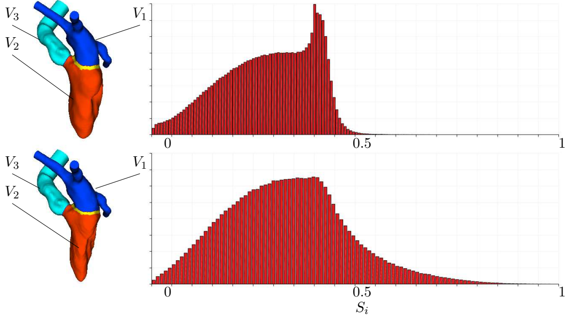
Figure 4.8: Skewness histograms for a left heart grid at end diastole (top figure) and mid-systole (bottom figure). Each left heart cavity is color tagged.
