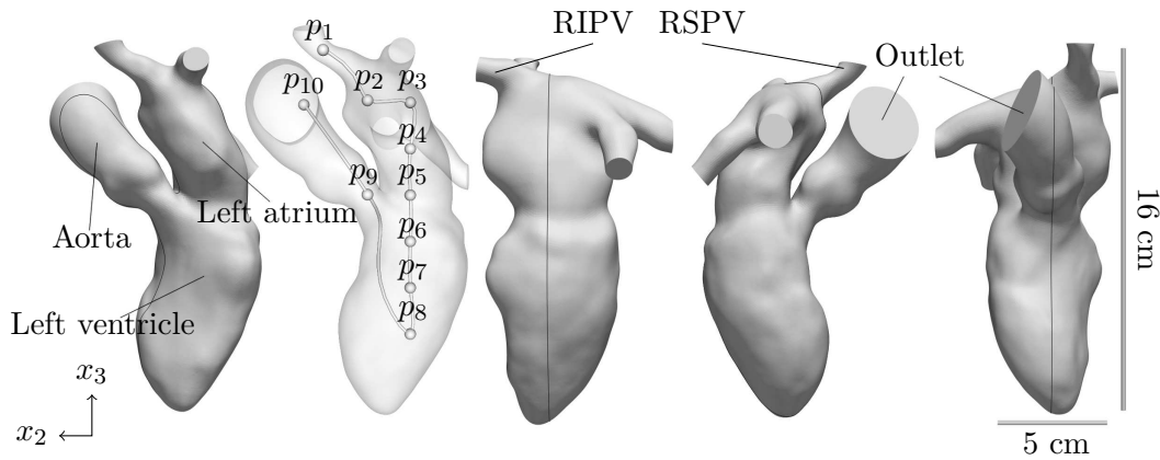
Figure 6.1: Template computational domain extracted from a 3D medical image. The same domain is represented from four different points of view and the left ventricle (LV), left atrium (LA), Aorta (AO) and two pulmonary veins are indicated. Black line passing through the left heart indicates the position of slices used to describe the flow in section 6.3. Probes locations and outflow patch are also indicated.
