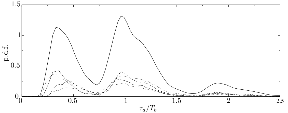
Figure 8.18: Probability density function of residence time in the left atrium (solid line). Each pulmonary vein contribution is plotted as well: RSPV (dashed line), RIPV (dotted line), LIPV (dashed dotted dotted line) and LSPV (dashed dashed dotted line).
