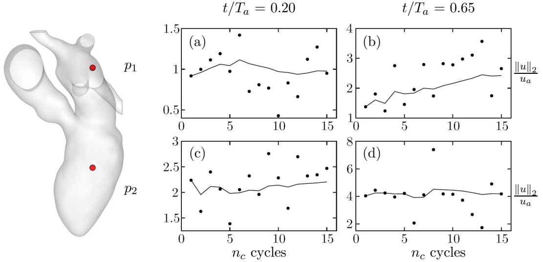
Figure 5.4: Left: left heart with probes p_1 and p_2 indicated. Right: solid lines represent the phase averaged velocity magnitude at probes locations using n_c cycles. The dots represent the instantaneous velocity magnitude for the n -ith cycle. The first column of plots represents the data at t/T_a = 0.20 , the second column at t/T_a = 0.65 . Top plots represent data from probe p_1 while the bottom plots represent data from probe p_2 .
