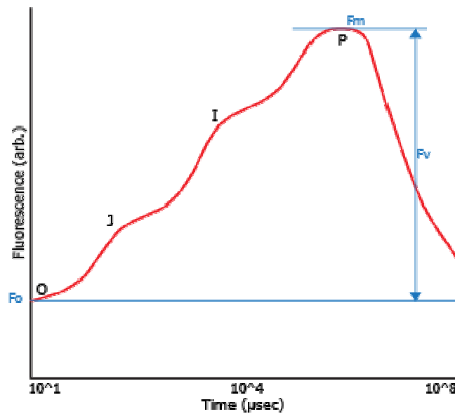
Figure 2-4 Kautsky curve
