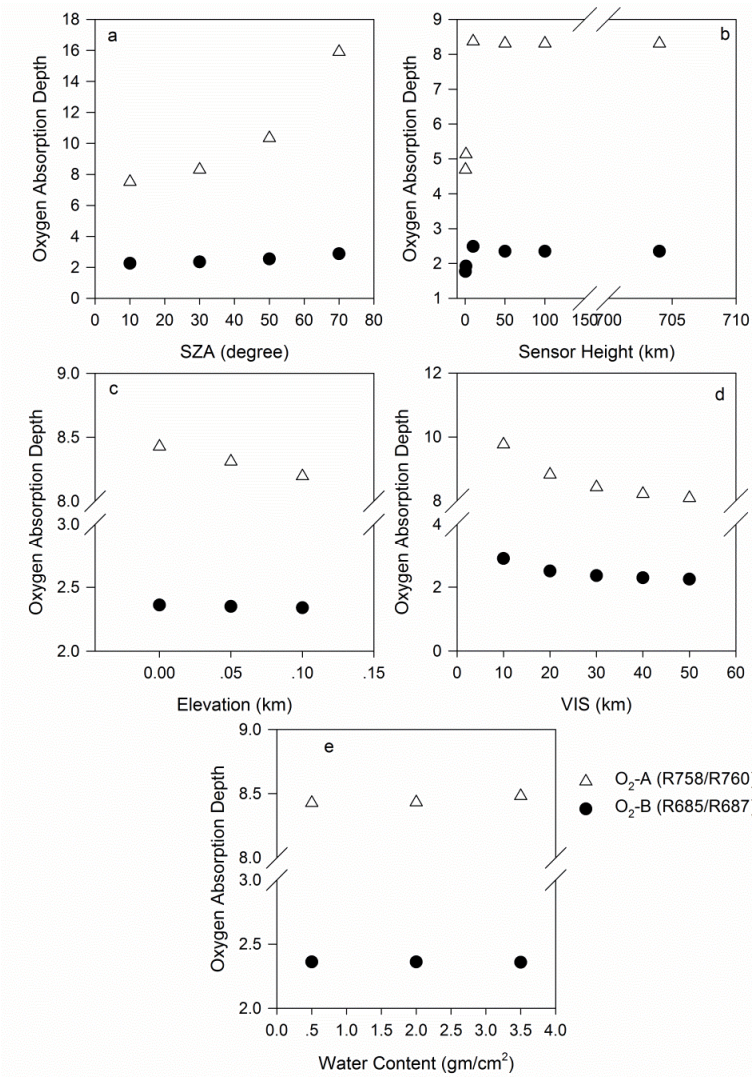
Figure 5-4 Atmospheric effects on the oxygen absorption band depth
