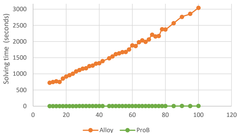
Figure 3.25 – Varying the number of vertices versus the solving time (13 rules, 10 contexts)
