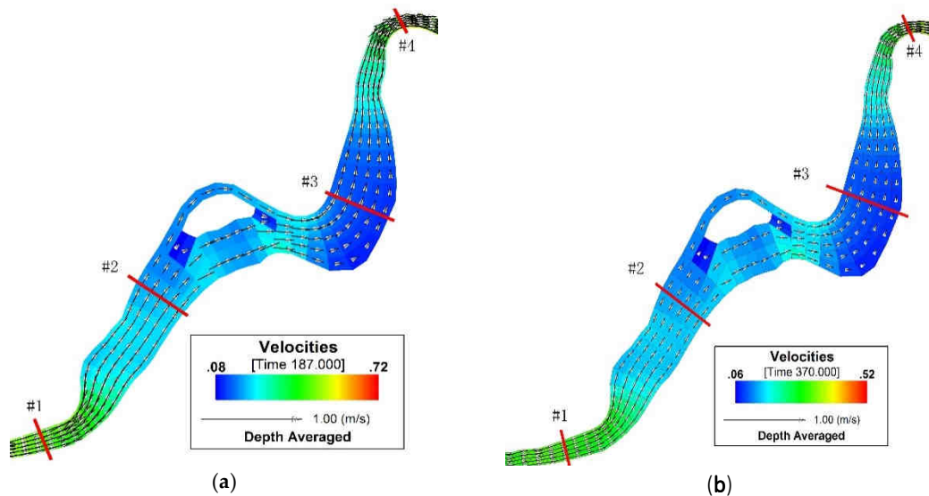
Figure 3-22. Schematic diagram for flow field in the urban section of Mudan River trunk stream. (a) open-water period; (b) ice-covered period.
