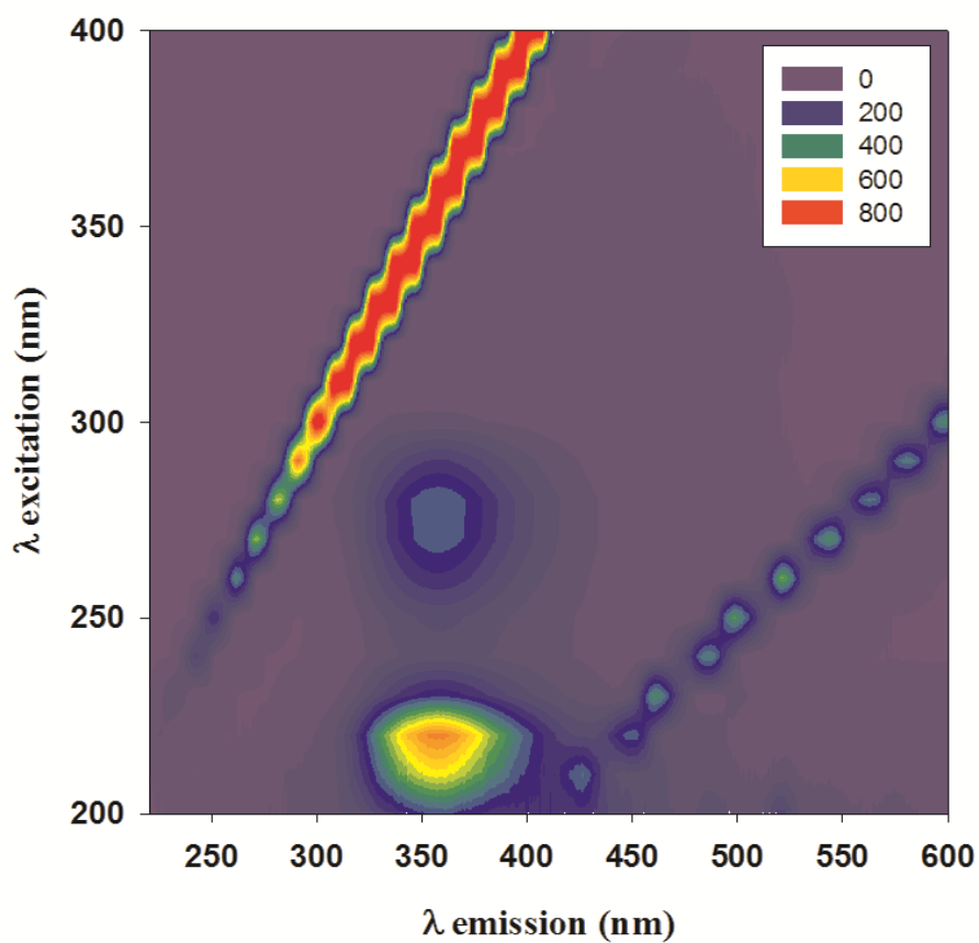
Figure SM1: 3D fluorescence excitation-emission matrix (as contour plot) of 10\mu\text{M} tryptophan M in milli-Q water. Fluorescence intensity is scaled from 0 to 800 intensity units. The linear feature (in red) is the Raman signal.
