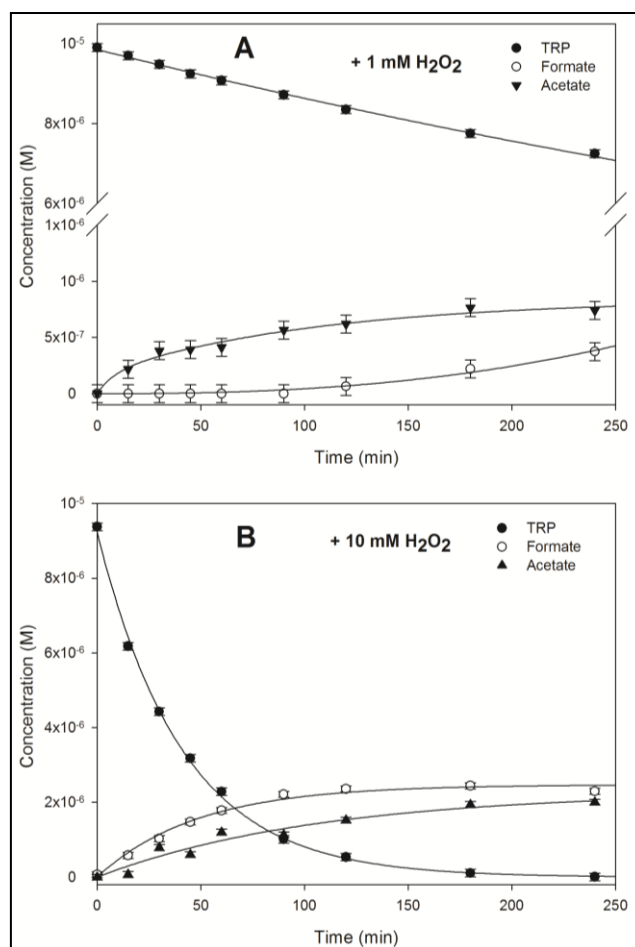
Figure 5: Disappearance of TRP (10 \mu M) in the presence of \text{H}_2\text{O}_2 1 mM (A) and 10 mM (B) and the formation of formate and acetate under polychromatic irradiation in water at a pH of approximately 5.5 and T = 288 \pm 3 K.
