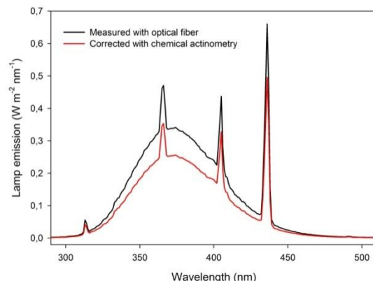
Figure 18: Lamp emission centered at 365 nm measured with optical fiber and corrected by chemical actinometry.
