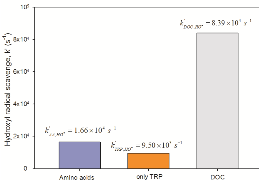
Figure 4: HO^\bullet scavenging rates ( k' ) of AAs, TRP and DOC. These values were determined based on the average values of \sum_i k''_{HO^\bullet,AA} [AA]_i , \sum_i k''_{HO^\bullet,TRP} [TRP]_i and \sum_i k''_{HO^\bullet,DOC} [DOC]_i using the concentrations and second-order rate constants reported in Tables S1 and S3. The k''_{HO^\bullet,DOC} value was taken from Arakaki et al. 103
