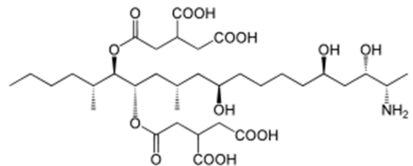
Fumonisines
