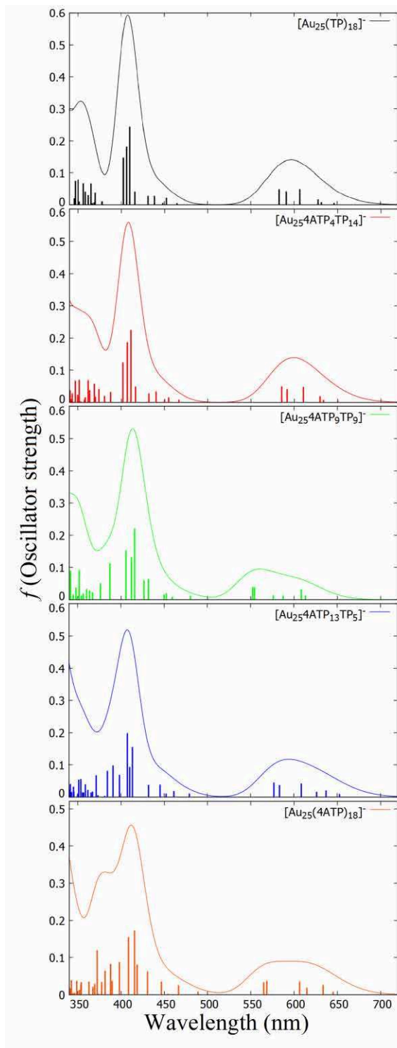
Figure 19. Computed UV-vis absorption spectra of the Janus [Au_{25}(4ATP)_x(TP)_{18-x}]^- clusters together with the monoligand protected [Au_{25}(4ATP)_{18}]^- and the [Au_{25}(TP)_{18}]^- at the DFT/CAM – B3LYP level. The height of the vertical bars give the oscillator strength of each transition and the spectra are obtained by convolution with Gaussian line shapes ( \sigma = 0.085 eV).
