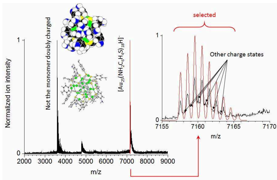
Figure 10. Negative – mode ESI – MS spectrum of the [Au_{25}(4ATP)_{18}]^{-} cluster. The inset shows the isotopomer splitting highlighting the presence of other charge states (other than one) in very low intensities. Clusters were analyzed in DMSO. Figure provided by Dr. J.-F Greisch (KIT).
