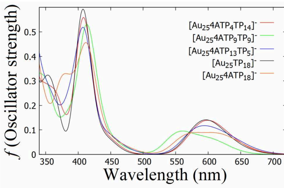
Figure 18. Computed UV–vis absorption spectra of the Janus [Au_{25}(4ATP)_x(TP)_{18-x}]^- clusters together with the monoligand protected [Au_{25}(4ATP)_{18}]^- and the [Au_{25}(TP)_{18}]^- at the DFT/CAM – B3LYP level.
