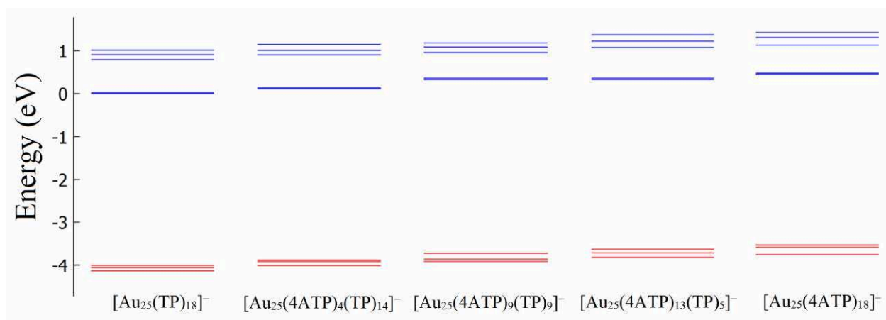
Figure 20. Molecular orbital diagram of the Janus [Au_{25}(4ATP)_x(TP)_{18-x}]^- clusters at the DFT/CAM – B3LYP level. The red bars are the p – SAMO three – fold quasi – degenerate HOMO (HOMO – 1, HOMO – 1 and HOMO – 2) and the blue bars stand for the 5 d – SAMO; the two degenerate LUMO and the 3 – fold quasi – degenerate LUMO + 1.
