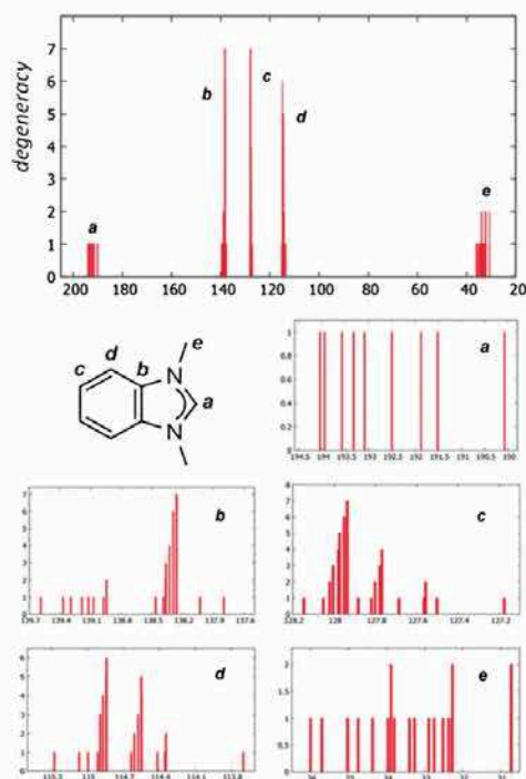
Figure 9. Calculated 13 C NMR spectrum of the (NHCa) 9 -Au 38 system in [D 2 ]DMSO. TMS (tetramethylsilane) was used as 13 C NMR reference. All calculations have been performed at the DFT CAM-B3LYP level of theory. The relativistic pseudopotential and basis set LANL2MB were used in the case of gold and for the other atoms 6–311 + G(2d,p) was employed.
