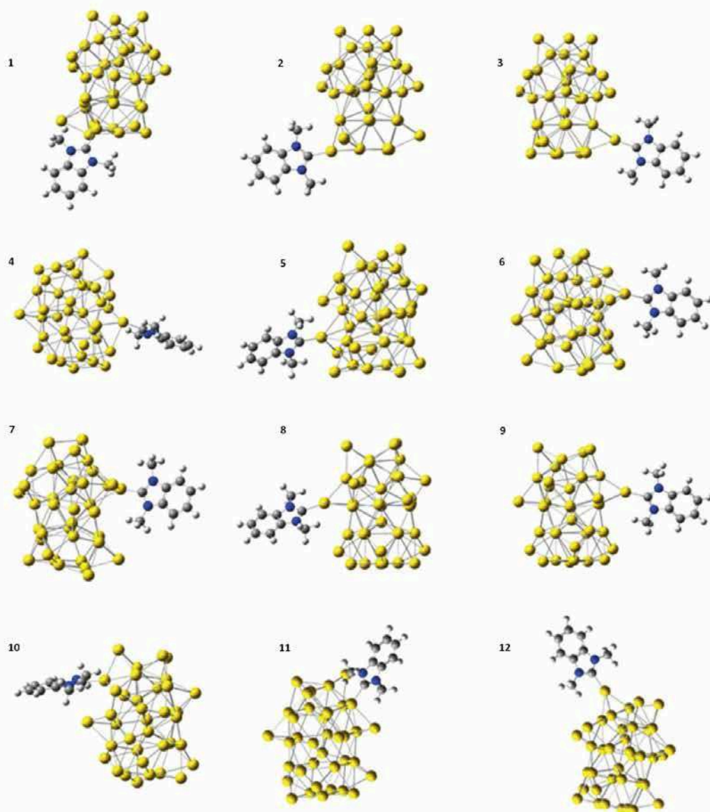
Figure 6. Equilibrium structures of the NHCa–Au 36 system, computed at the CAM-B3LYP LANL2MB/6-31G(d) level in the gas phase.
