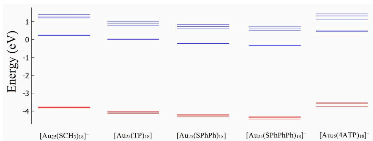
Figure 8. Molecular orbital diagram of the [Au_{25}(SR)_{18}]^- clusters at the DFT/CAM – B3LYP level. The red bars are the p – SAMO 3 – fold quasi – degenerate HOMO (HOMO – 1, HOMO – 1 and HOMO – 2) and the blue bars stand for the five d – SAMO; the two degenerate LUMO and the 3 – fold quasi – degenerate LUMO + 1.
