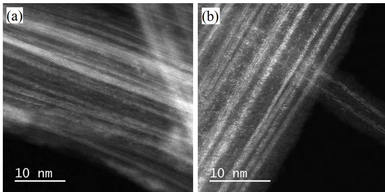
Fig. 3.20 - ADF images of (a) \text{FeI}_2@\text{DWCNTs-p} and (b) \text{FeF}_3@\text{DWCNTs-p} showing the encapsulated (here amorphous-like) material in both samples.
