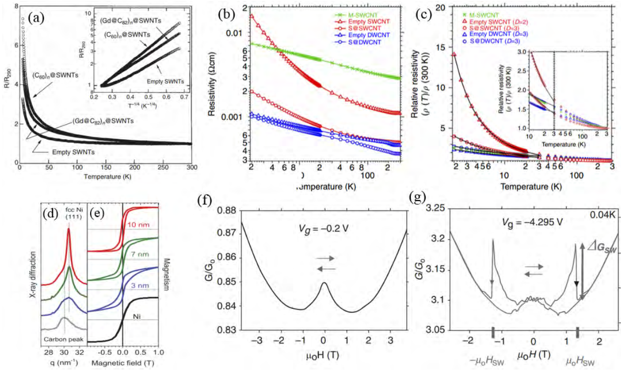
Fig. 1.18 (a) Temperature dependence of the resistance for buckypapers of (\text{Gd}@C_{82})@SWCNT , C_{60}@SWCNT , and empty SWCNTs. Inset is a semi-logarithmic plot against T^{-1/4} [49]; (b) and (c) Relationship between temperature and resistivity as well as relative resistivity (normalized by the T=300 K value) for films prepared with empty SWCNTs, S@SWCNTs, empty DWCNTs and S@DWCNTs, in comparison with pristine M-SWCNTs. In (c), hopping model is used to fit the curves of the above samples (black solid line) except M-SWCNTs whose curve could not be reproduced by the model and D refers to the dimensionality of electron hopping in these systems. The enlarged relative resistivity curves for temperature between 10 and 300 K are shown in the inset of (c) [42]; (d) X-ray diffraction profiles for nickel clusters confined in SWCNTs with diameter of 3 nm, 7 nm and 10 nm respectively. The diffraction profile of empty SWCNTs is also shown; (e) magnetization curves for the same materials as measured by SQUID at 5 K. The magnetization curve of bulk Ni is also show; (f) and (g) Variation of conductance as a function of cycling magnetic field measured on isolated Co@SWCNT bundles contacted (with Pd) following the transistor-type device, for an angle of 25^\circ between the direction of the outer magnetic field and the elongation axis of the contacted bundle, and at a temperature
