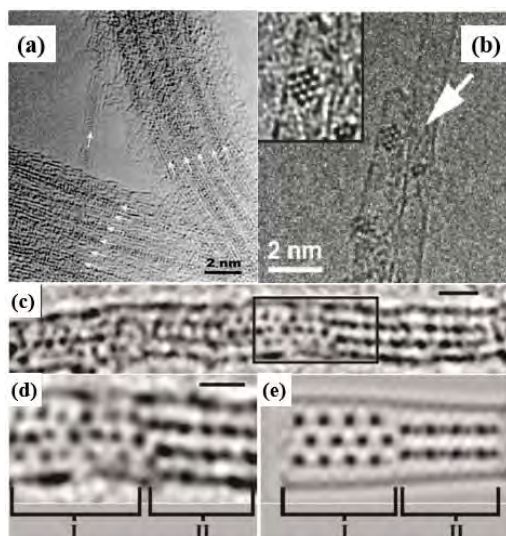
Fig. 1.13 - (a) HRTEM image of SWCNTs filled with PbO. White arrows point to nanotubes filled with lead oxide, a high filling rate \geq 70\% was reported [108]; (b) HRTEM image and detail of \text{UO}_2 clusters inside SWCNTs [33]; (c)-(e) TEM image and detail of CsOH crystals inside SWCNTs (scale bar = 1.0 nm), and corresponding Scherzer defocus simulated TEM image [33].
