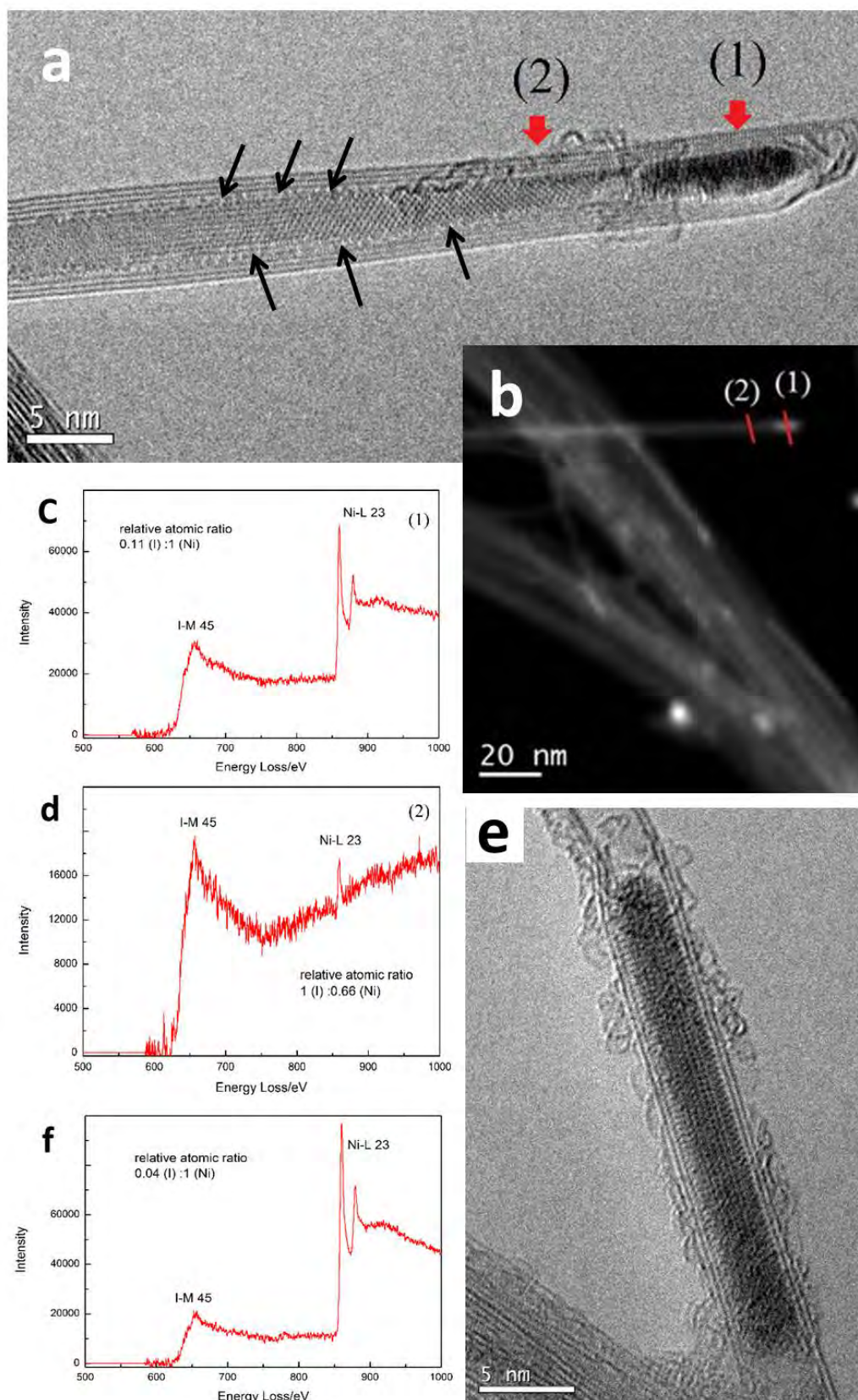
Fig. 3.18 - (a) and (b) HRTEM and HAADF images of a \text{NiI}_x crystal with various compositions; (c) and (d) EEL spectra collected from fragment (1) and (2) labelled in (a) and (b); (e) HRTEM image of another intermediate \text{NiI}_x ( x < 2 ) crystal encapsulated within a DWCNT; (f) EEL spectrum collected from the crystals shown in (e).
