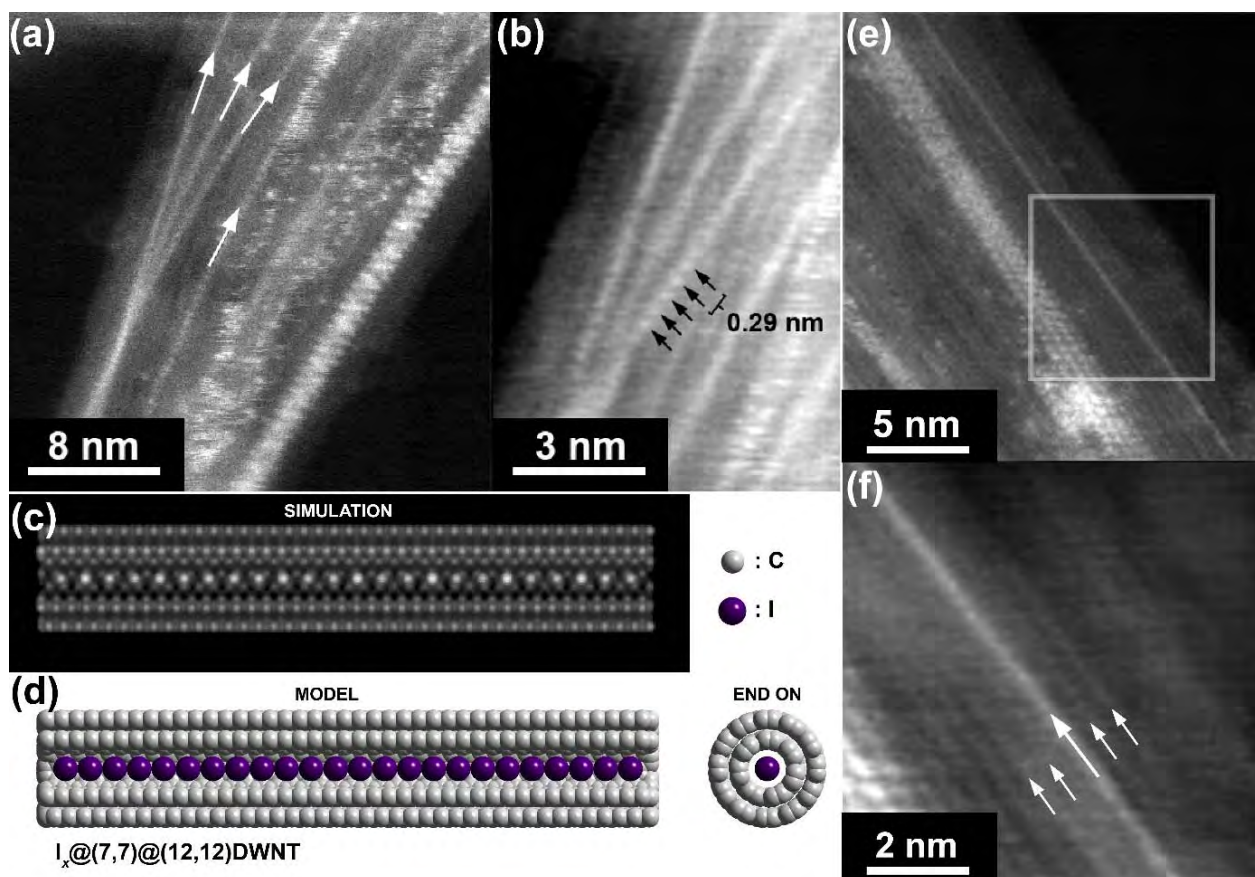
Fig. 2.18 - (a) ADF image of a bundle of CNTs from \text{NiI}_2 @DWCNT sample with at least four 1D iodine-chains (arrowed) visible. (b) Detail from (a) indicating measured distances between I atoms in a chain. (c) and (d) are a simulated ADF image and the corresponding structural model of a 1D iodine-chain inside a (7,7)@(12,12) DWCNT. The wall helicities of the model for the DWCNT are derived from (e) and (f) where the DWCNT walls are visible. Indeed, (e) and (f) show an ADF image and a detail of it respectively, showing a DWCNT which contains a 1D iodine chain (large white arrow) in-between the two walls of the DWCNT (small white arrows). Note that in order to accommodate the 1D iodine chain, the inner SWCNT must fit perfectly around the chain in order to retain a linear structure.
