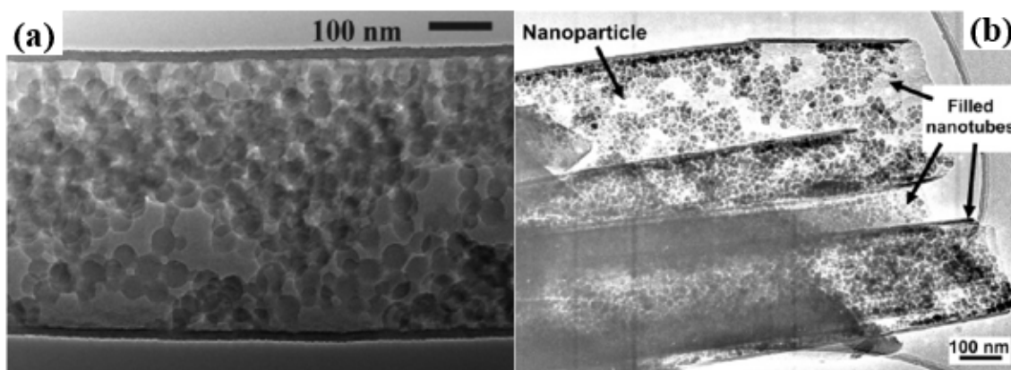
Fig. 1.7 - TEM images of MWCNTs filled with (a) polystyrene nanobeads via bringing MWCNTs into contact with the related suspension in ethylene glycol and deionized water [94]; (b) \text{Fe}_3\text{O}_4 nanoparticles via bringing MWCNTs into contact with organic- or water-based ferrofluids [95].
