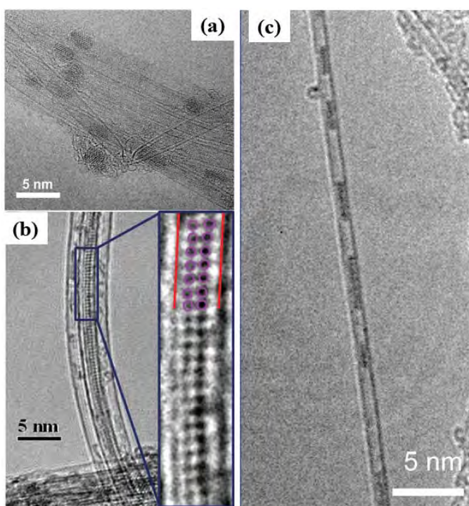
Fig. 1.12 - HRTEM images of (a) Ni clusters filled SWCNTs obtained by annealing initial \text{NiCp}_2 -filled SWCNTs at 500 °C for 2 hours [159]; (b) SWCNTs filled with Eu nanowires (left) and magnified image (right). In the magnified image, red lines correspond to the side wall of the SWCNT, and purple circles correspond to the Eu atoms [154]; (c) a Co-nanoparticle-filled SWCNT [156].
