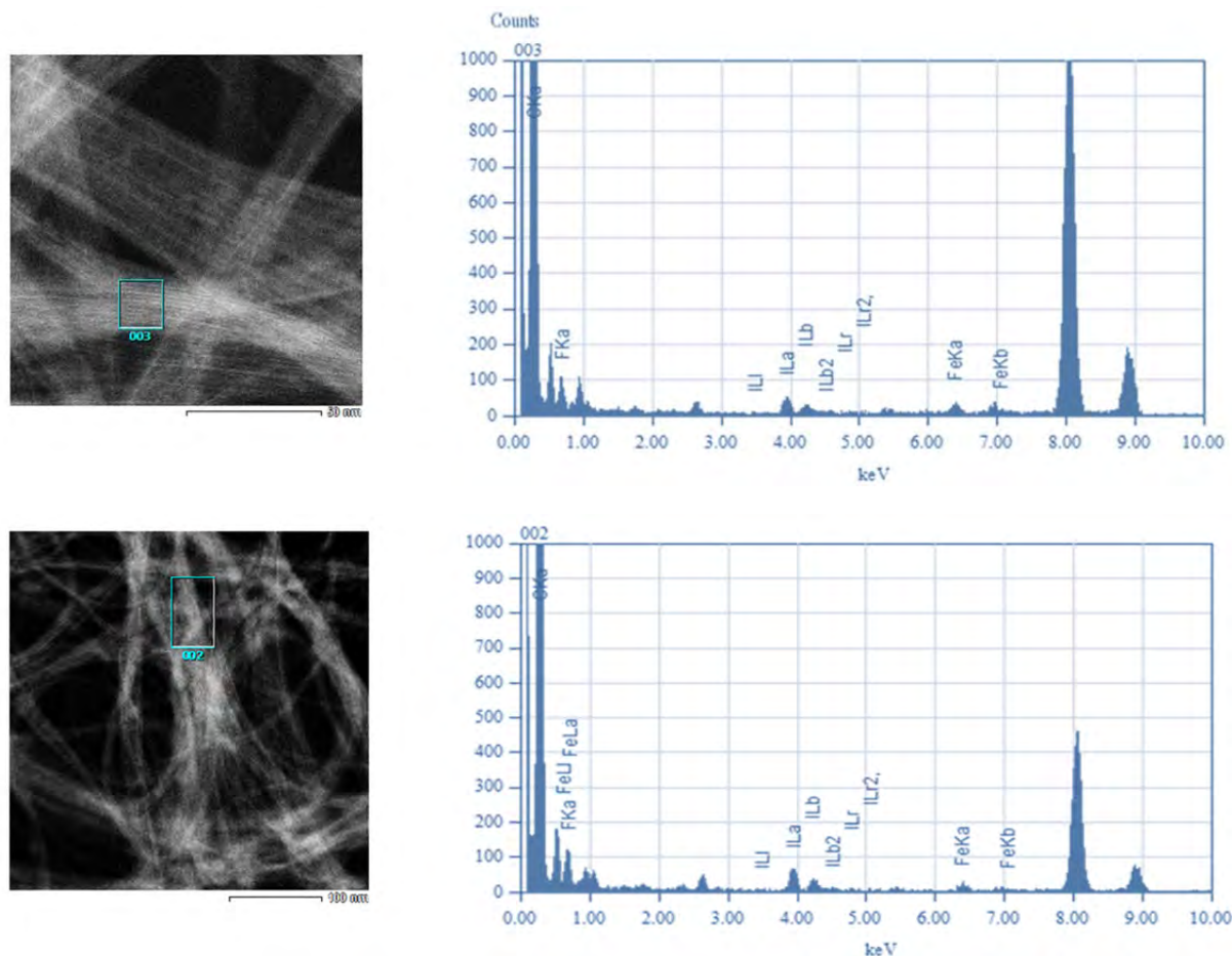
Fig. 3.22 - (a) and (c) are STEM images of \text{FeF}_3\text{@DWCNTs-p} and (b) and (d) are X-EDS spectra collected from the DWCNT bundles boxed in (a) and (c).
