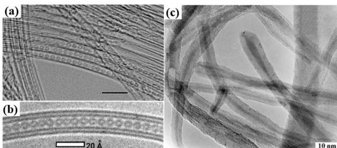
Fig. 1.6 - HRTEM images of (a) C_{60} @SWCNTs prepared by annealing SWCNTs and C_{60} at 1100^{\circ}\text{C} for 14h [46]; (b) C_{60} @DWCNTs prepared by annealing DWCNTs and C_{60} altogether in a closed vessel at various temperatures in the range of 200\text{--}520^{\circ}\text{C} for 48h [92]; (c) Se@MWCNTs prepared by heating MWCNTs and Se at 500^{\circ}\text{C} for 1h [89].
