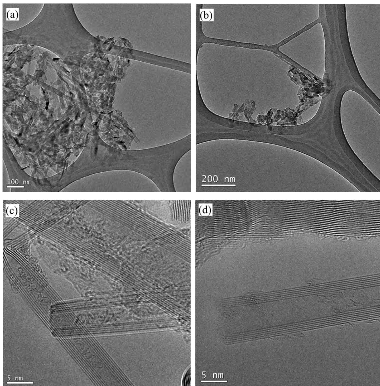
Fig. 2.12 - (a) and (b) TEM images of \text{NiI}_2\text{@BNNTs} showing the destroyed network of BNNTs after filling; (c) and (d) HRTEM images of some remaining BNNTs from the \text{NiI}_2\text{@BNNTs} experiment showing that they are unfilled, even if opened.
