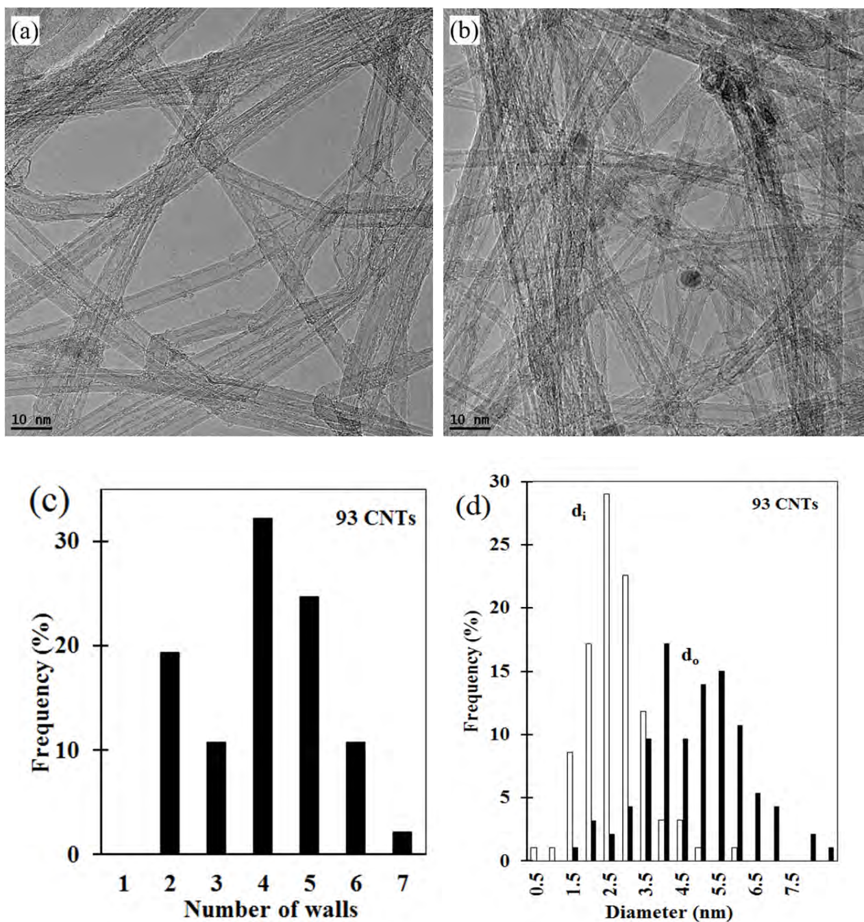
Fig. 2.2 - (a) and (b) are HRTEM images of FWCNTs showing the presence of tubes with 2~6 walls; (c) and (d) are distributions of the numbers of walls and inner ( d_i ) and outer ( d_o ) diameters for the whole population (established from 93 individual CNTs).
