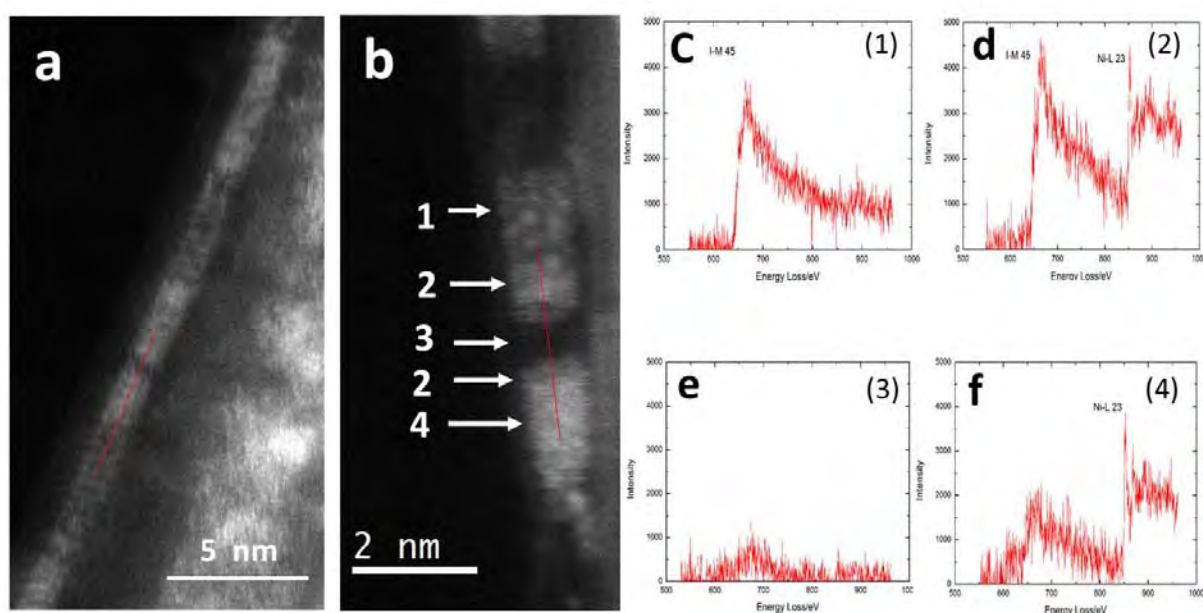
Fig. 3.14 - (a) and (b) ADF images of encapsulated crystals showing contrast variations in Ni@DWCNTs_500_7; (c) to (f) are the corresponding EEL spectra collected from positions 1 to 4 indicated by arrows in (b), respectively. Meanwhile, the absence of any signal in spectrum (e) demonstrates the spatial resolution of the electron probe.
