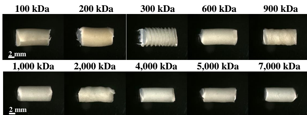
Figure 10: Impact of the PEO molecular weight on the appearance of hot melt extrudates processed at 100 °C.
