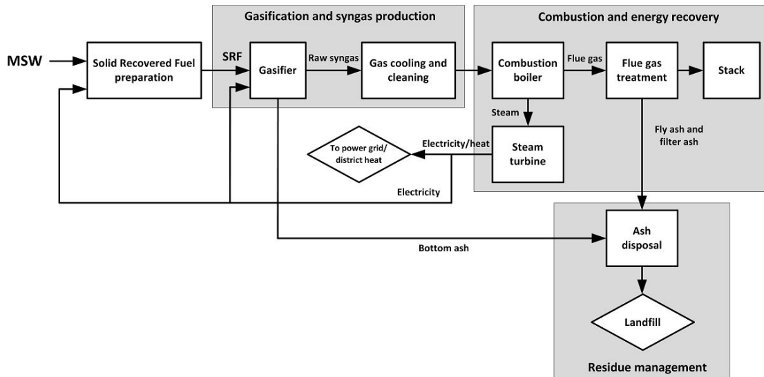
Figure 6. 2 Flowchart of the gasification-based WtE process (S1)
