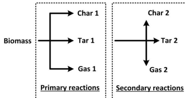
Figure 1. 3 Biomass pyrolysis concept proposed by the University of Waterloo [4]
