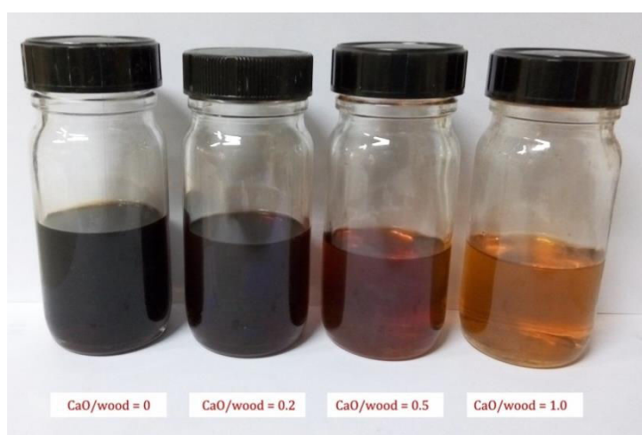
Figure 4. 5 Effect of CaO/wood mass ratio on the characteristics of collected tar (steam flowrate = 160 g/h; temperature = 700 °C; reaction = 15 min); from left to right: CaO/wood mass ratio of 0, 0.2, 0.5 and 1
