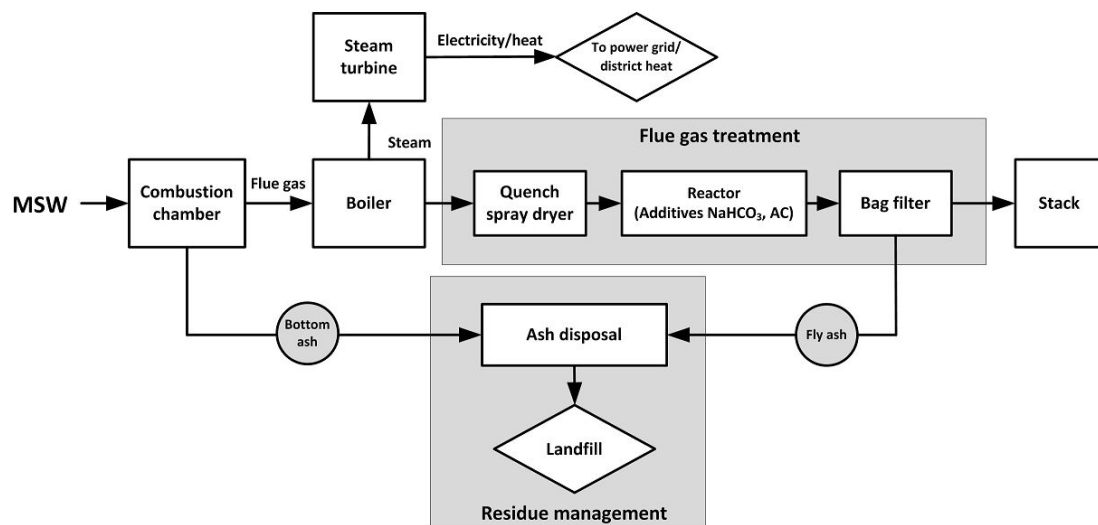
Figure 6. 3 Flowchart of the incineration process
