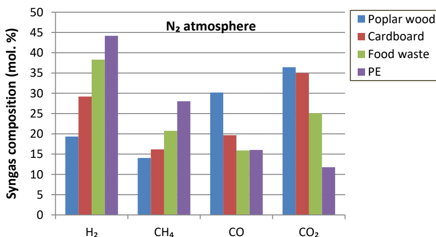
Figure 3. 1 Syngas composition from pyro-gasification of different MSW single-component under N_2 atmosphere (data obtained from lab-scale fluidized bed at 650 °C for 15 min)
