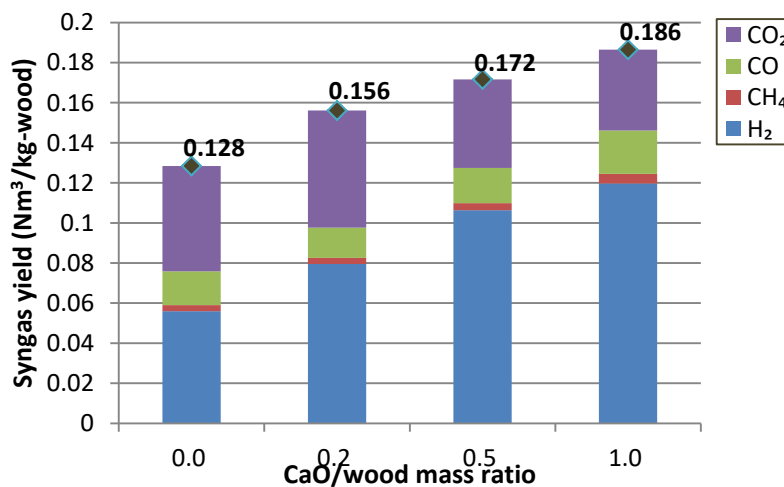
Figure 4. 2 Effect of CaO/wood mass ratio on syngas yield (steam flowrate = 160 g/h; temperature = 700 °C; reaction = 15 min)
