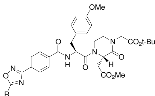
Figure 1.7 1,2,4-Oxadiazole-based double prodrugs of the potent GPIIb/IIIa antagonists
