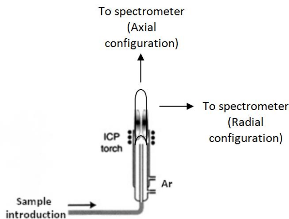
Figure 2.5 Radial and axial view configurations available for ICP-AES, Thermo Scientific iCAP 6500.
