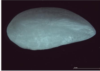
Trisopterus sp.
