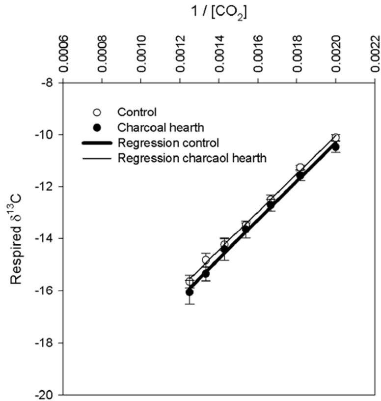
Figure III-31 : Keeling plots measured by CRDS showing the \delta^{13}\text{C} of respired CO 2 fluxes versus the reciprocal of CO 2 concentration for control and charcoal hearth incubated soils ( \delta^{13}\text{C}_{\text{CONTROL}} = 7353 \cdot [\text{CO}_2]^{-1} - 24.8 , R^2 = 0.99 ; \delta^{13}\text{C}_{\text{CHARCOAL HEARTH}} = 7467 \cdot [\text{CO}_2]^{-1} - 25.2 , R^2 = 0.99 ). Horizontal and vertical bars indicate standard deviations (n = 3).
