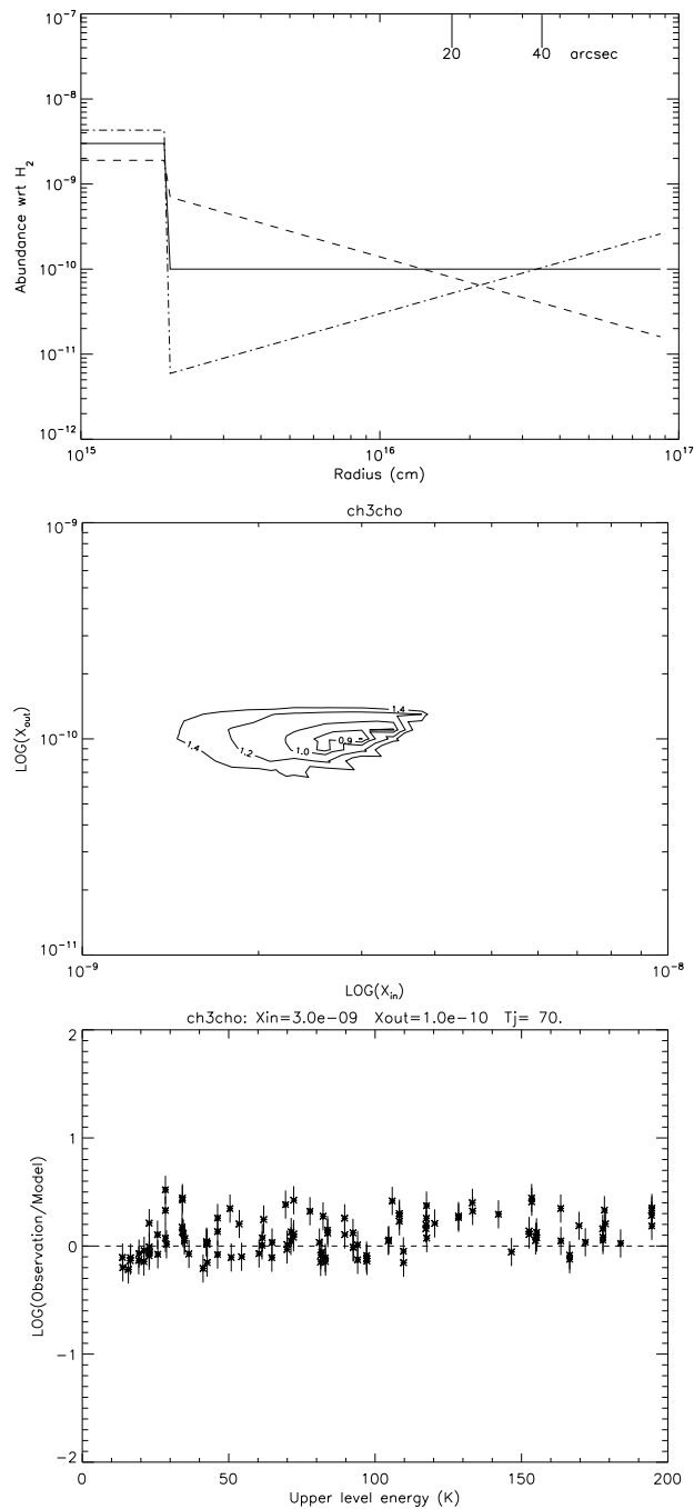
FIGURE 4.1: Example of the acetaldehyde analysis. Upper panel: Abundance profiles of the best fit obtained considering the cold envelope abundance profile following a power law dependence with radius (Eq.5.1) of \alpha equal to -1 (dashed), 0 (solid) and 1 (dotted-dashed) respectively. Middle panel: \chi^2 contour plot assuming the best fit T_{jump}=70 K and \alpha=0 . Bottom panel: Ratio of the observed over predicted line flux as a function of the upper level energy of the transition for the best fit solution (Table 4.1).
