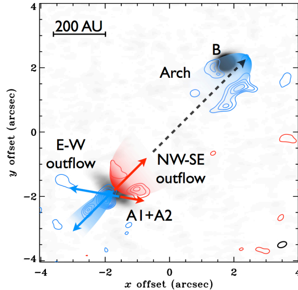
FIGURE 2.5: The CO J=6-5 emission integrated over the highest velocities. The different features are highlighted by arrows and are labeled. The black dashed arrow is an extrapolation of the red lobe of the NW-SE outflow (Kristensen et al. 2013).
