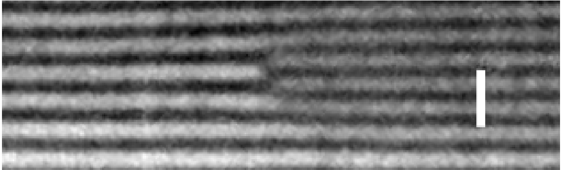
Figure 5.5: Photomicrograph of oily streaks having concentration c = 4 wt.-% at temperature \Delta T = 1.3^\circ\text{C} , clearly showing the edge dislocations. Bar corresponds to 2 \mu\text{m} and is parallel to the easy axis.
