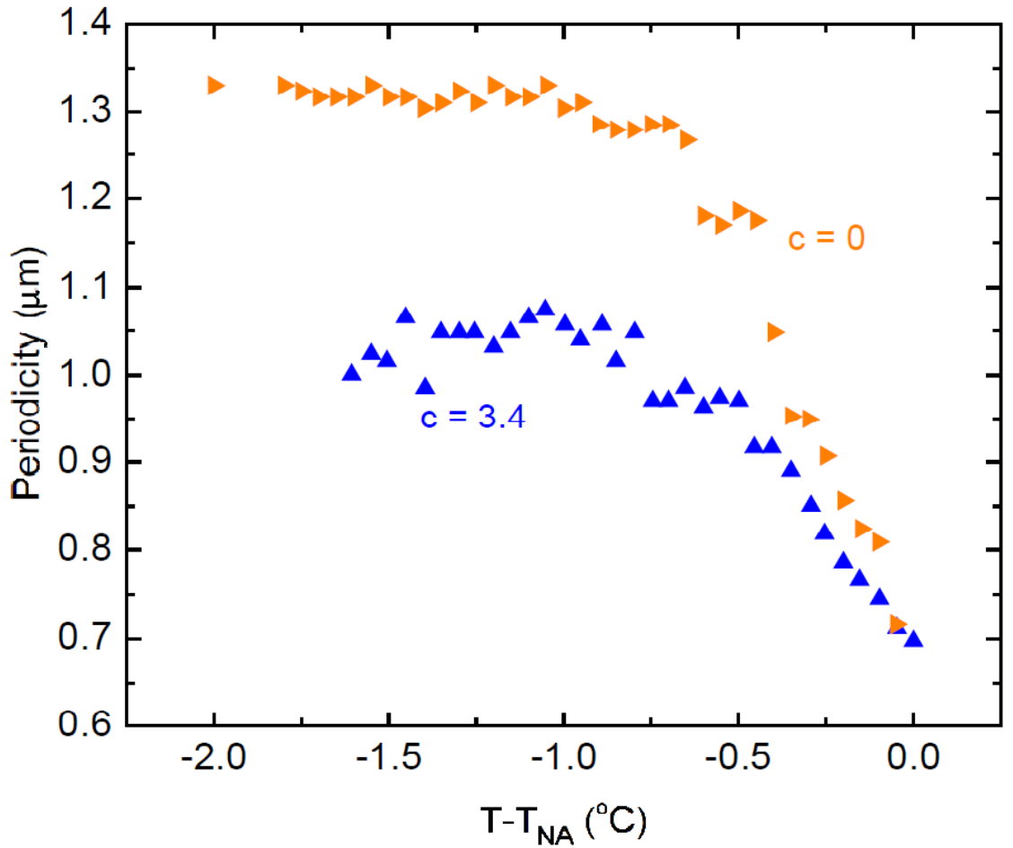
Figure 5.12: Average periodicities \langle p \rangle for two concentrations, c = 0 and 3.4 wt-%, vs. temperature on polyimide.
