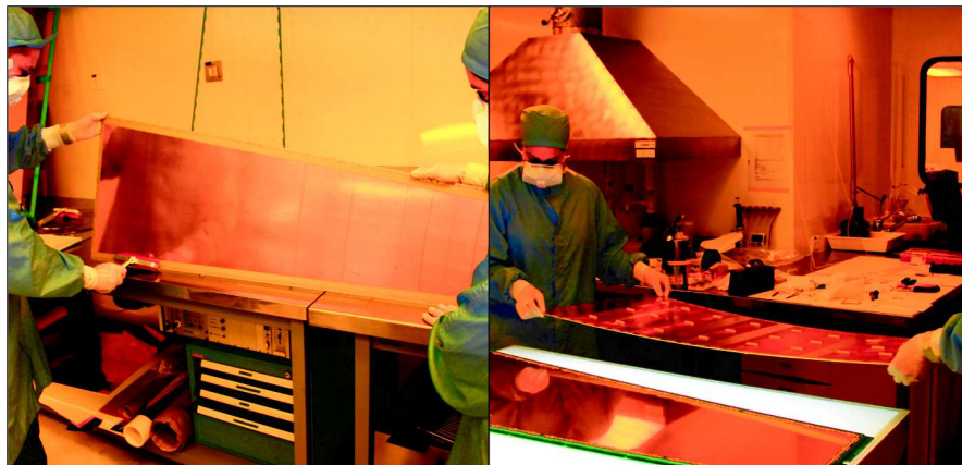
FIGURE B.15: Step 15: after being cleaned (left), the readout board is placed on top of the external frame to close the chamber.
