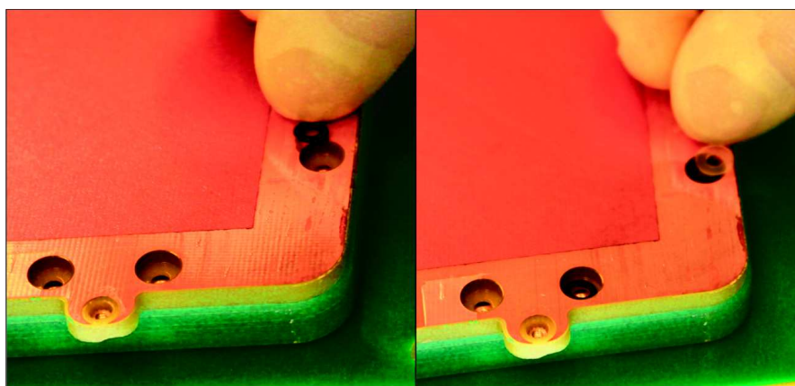
FIGURE B.16: Step 16: finally, O-rings and washers are inserted in the dedicated housings of the readout board before the last screws are used to attach all the elements together and close the gas volume.
