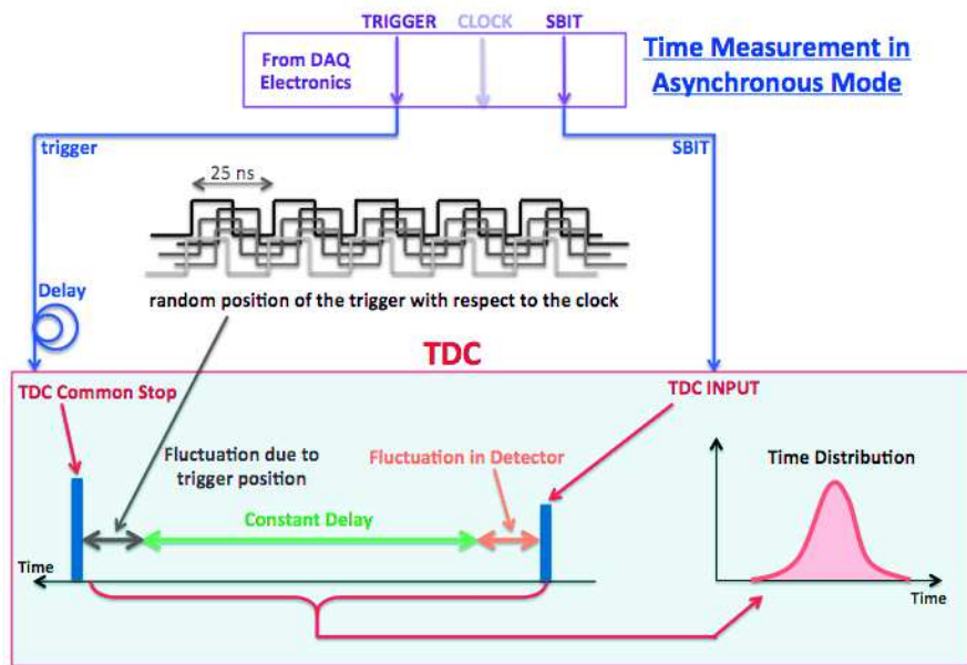
FIGURE 6.24: Schematic representation of the timing DAQ showing the different contributions to the delay between the trigger signal and the SBIT from the GE1/1 chamber.
