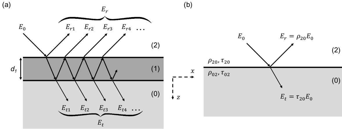
Figure C.1 – (a) Multiple-beam interference from a one layer of medium (1) and thickness d_1 encapsulated in semi-infinite media (0) and (2). E_0 is the incident electric field and E_r ( E_t ) is the total reflected (transmitted) electric field. (b) Equivalent representation of the problem where medium (1) is represented as an interface separating media (2) and (0) with reflection \rho and transmission \tau coefficients. Note that the beams are drawn with an angle for better illustration but the calculations are done for normal incidence.
