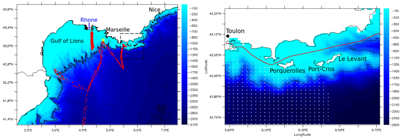
Fig. 1 Bathymetry and area names for the studied domains. These regions also correspond to the domains computed with the HRC (GLAZUR64), left panel, and the VHRC (NIDOR192), right panel.
