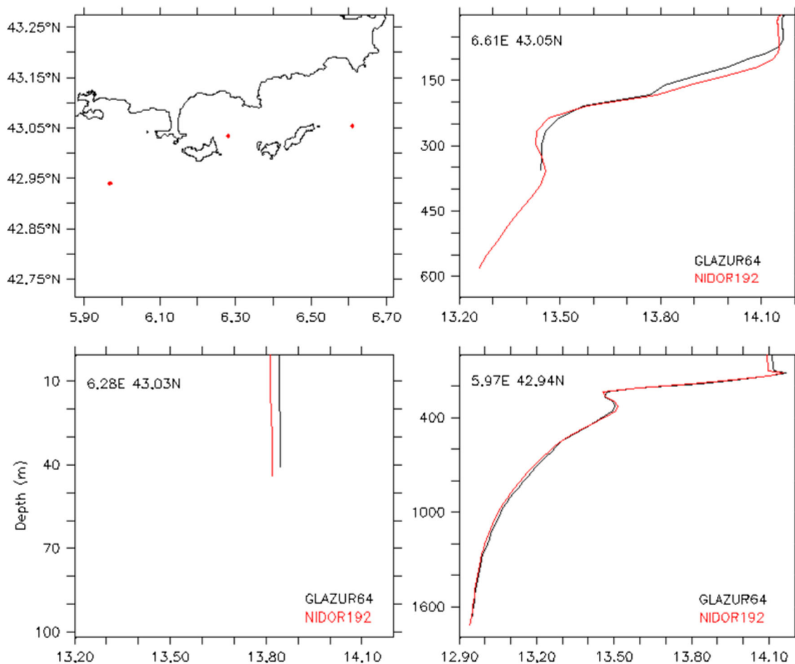
Fig. 3 Daily mean temperature profiles ( ^{\circ}\text{C} ) from the HRC (black) and VHRC (red) at three different locations: two in the NC path and one in the bay for the last day of the exploited run (2014/01/31)
