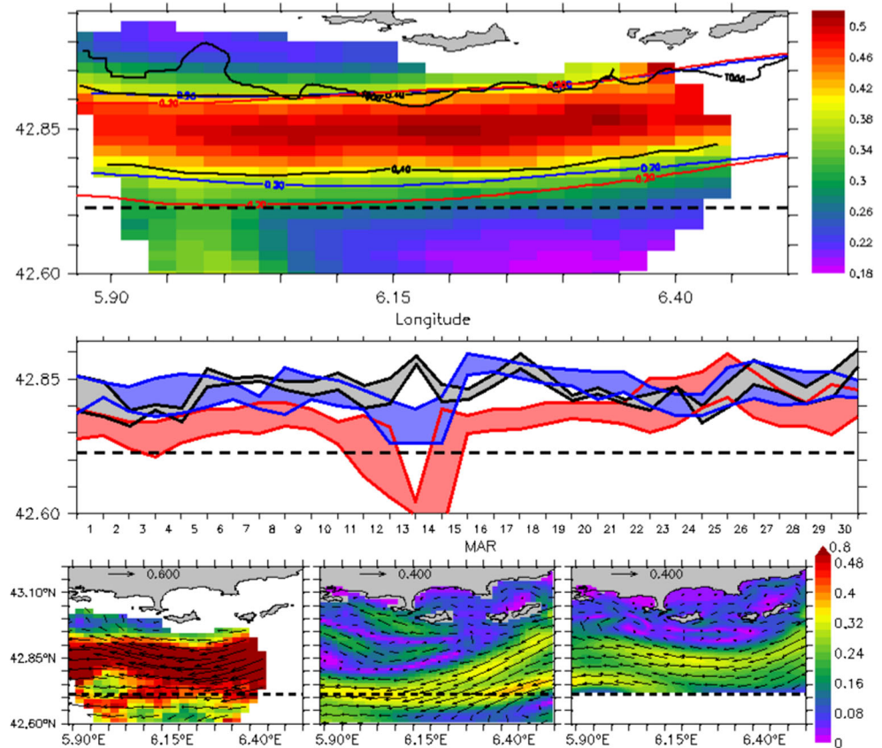
Fig. 4 Top : Time averaged surface velocities measured by HF radar from 2013/09/06 to 2014/05/31 (m/s). The iso-current 0.4 m/s is overlaid for the radar, and 0.2 m/s for the model simulations ( red : HRC and blue : VHRC). The 1000-m isobath is also overlaid in black . Middle : Temporal evolution of the positioning of the estimated NC core, between maximum and 80 % of it iso-current, at 6.34° E for March 2014, red : HRC, blue : VHRC, grey : HF radar observations daily averaged. Bottom : Surface velocities for the 2014/03/12 observed by the radar ( left ) and simulated by the HRC ( middle ) and the VHRC-2W ( right )
